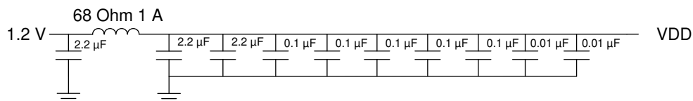
✎ 10-3. VDD Recommended Filter
