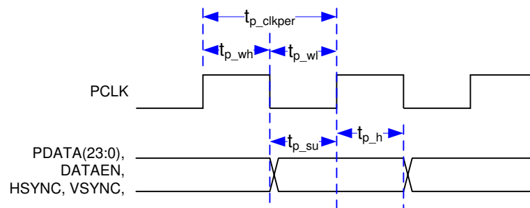
FIG 6-3. Parallel Video Interface General Timing
