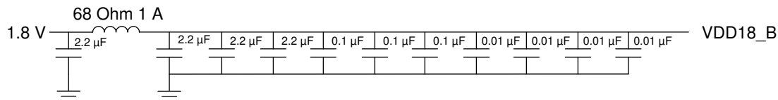
✎ 10-2. VDD18_B Recommended Filter
