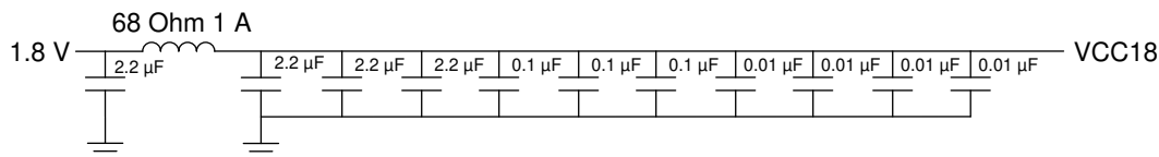
✎ 10-1. VCC18 Recommended Filter
