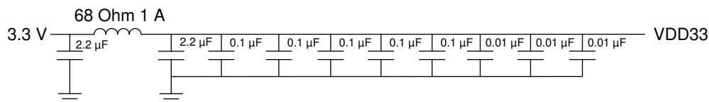
✎ 10-4. VDD33 Recommended Filter
