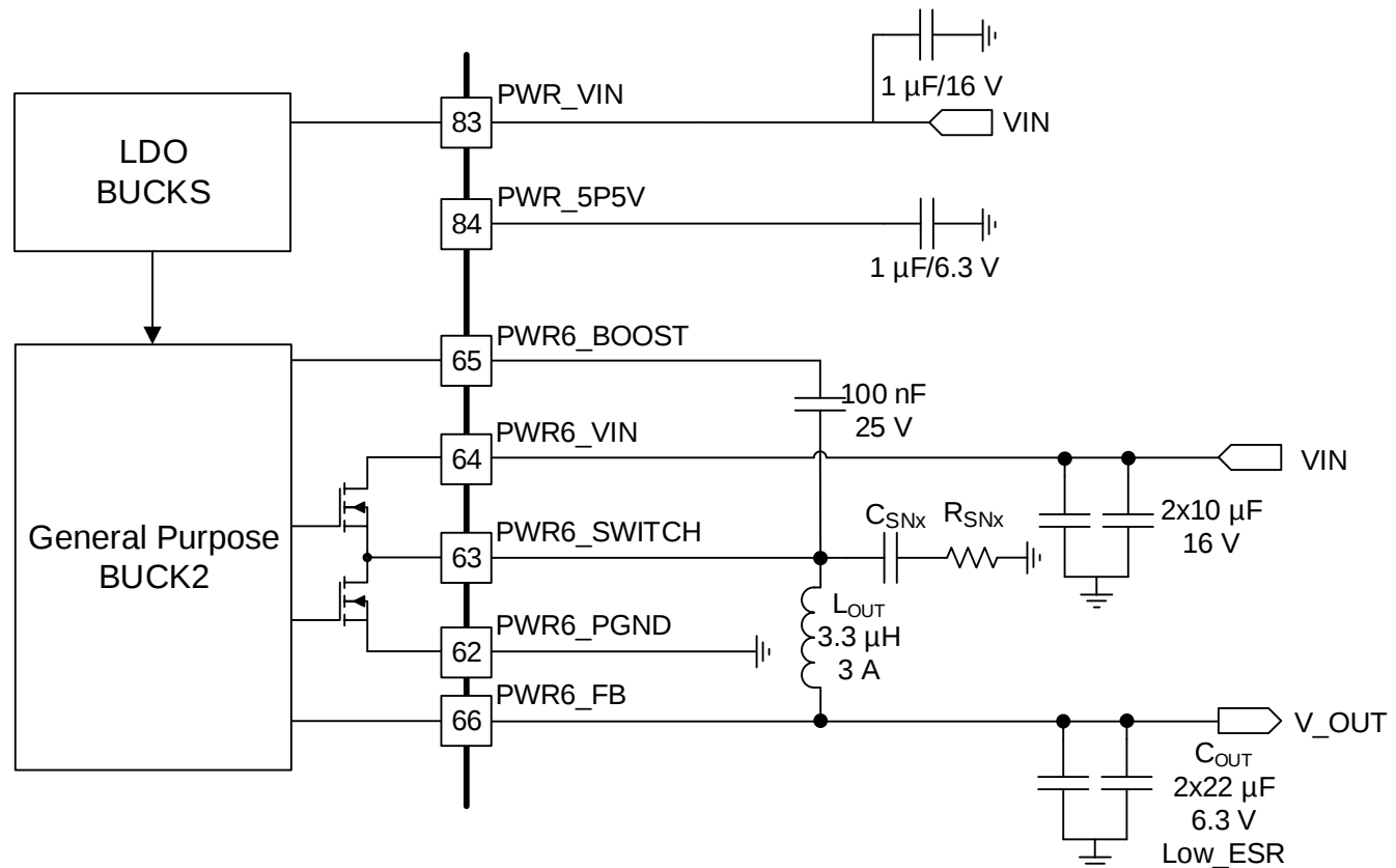
Figure 16. Buck Converter
