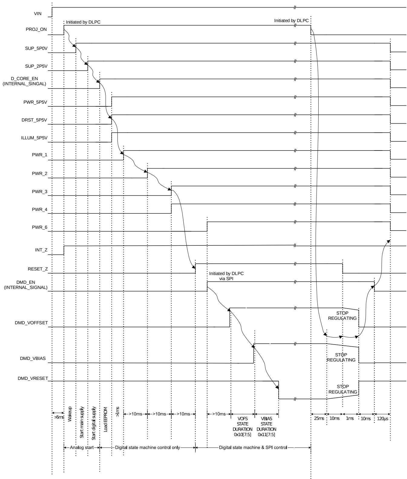
23. Power Sequence Normal Shutdown Mode
