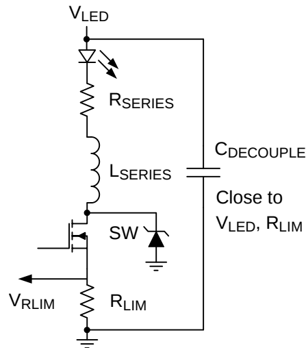
FIG 32. Parasitic Inductance ( L_{\text{Series}} ) and Resistance ( R_{\text{series}} ) in Series with LED
