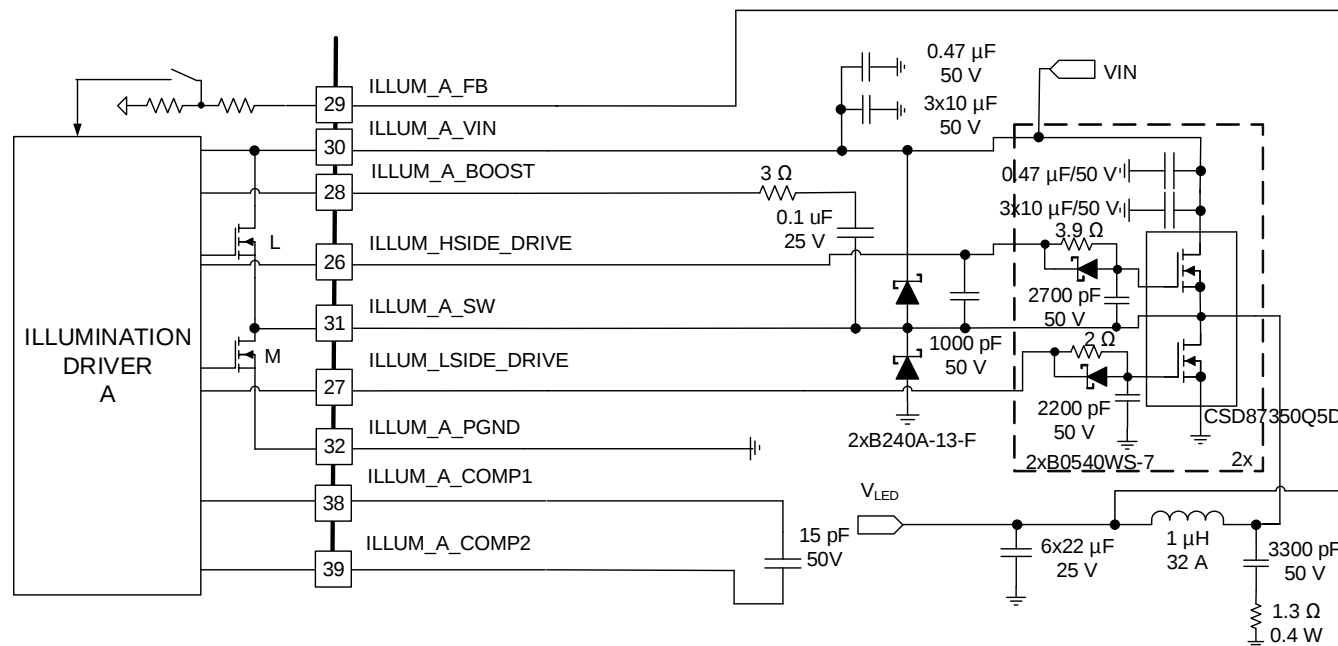
Figure 6. Typical Illumination Driver Configuration
