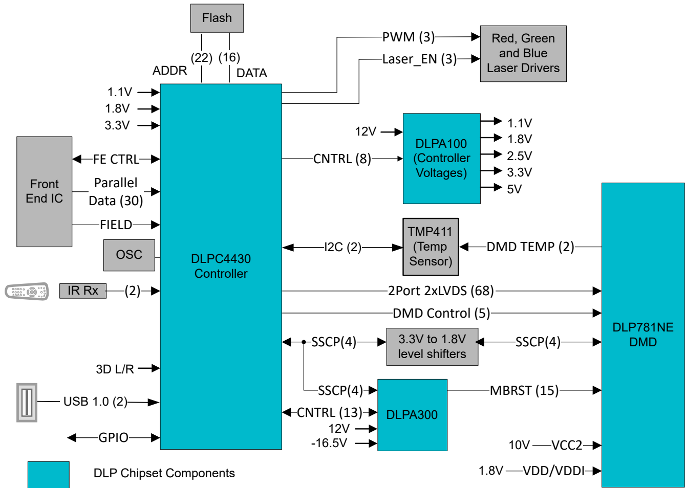
図 7-1. Typical WUXGA RGB Laser Application
