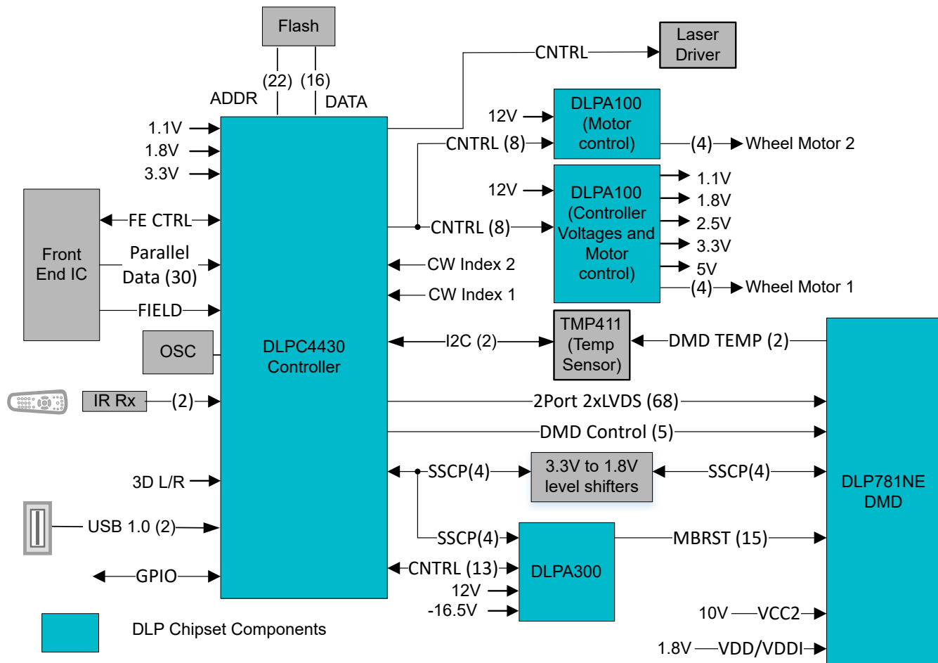
図 7-2. Typical WUXGA Laser Phosphor Application
