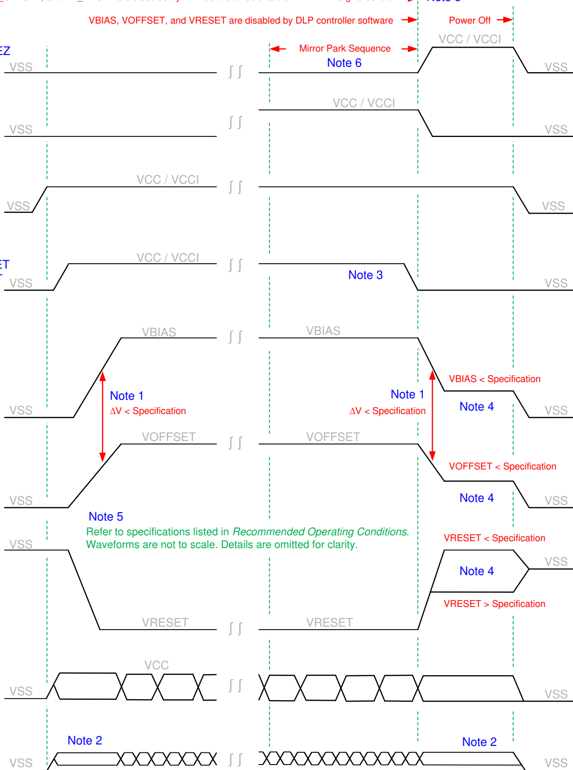
8-1. DMD Power Supply Sequencing Requirements
