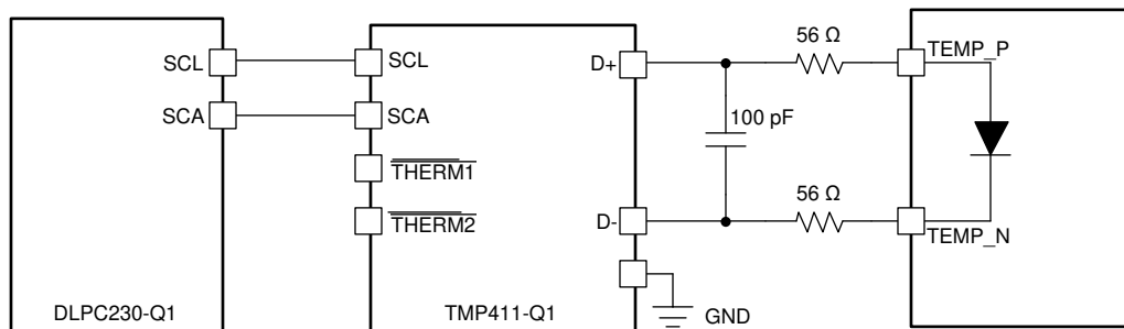
7-1. Temperature Sense Diode Typical Circuit Configuration
