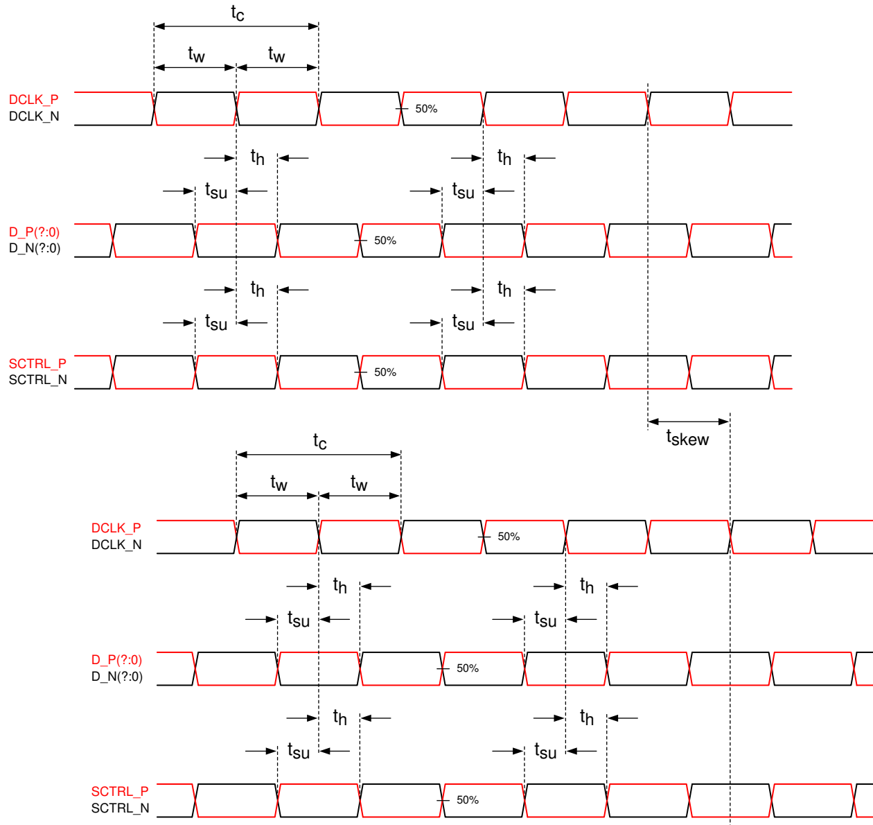
図 5-6. Timing Requirements
