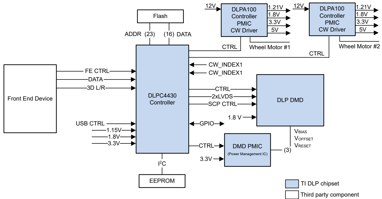
FIG 7-1. Typical DLPC4430 Application (LED, Top; LPCW, Bottom)
