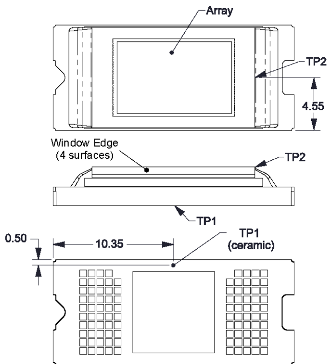
8-4. Thermal Test Point Location - FQD Package
