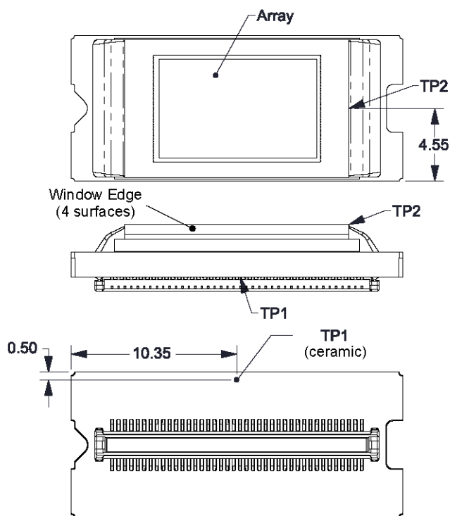
8-3. Thermal Test Point Location - FQE Package
