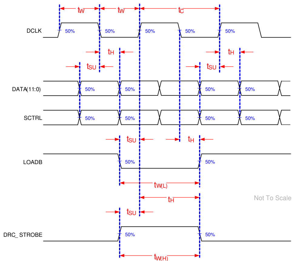
Figure 6-2. Switching Parameters 1
