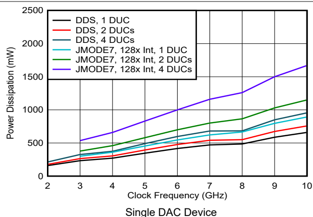
FIG 6-57. VDDDIG Current vs Clock Frequency and Digital Mode
