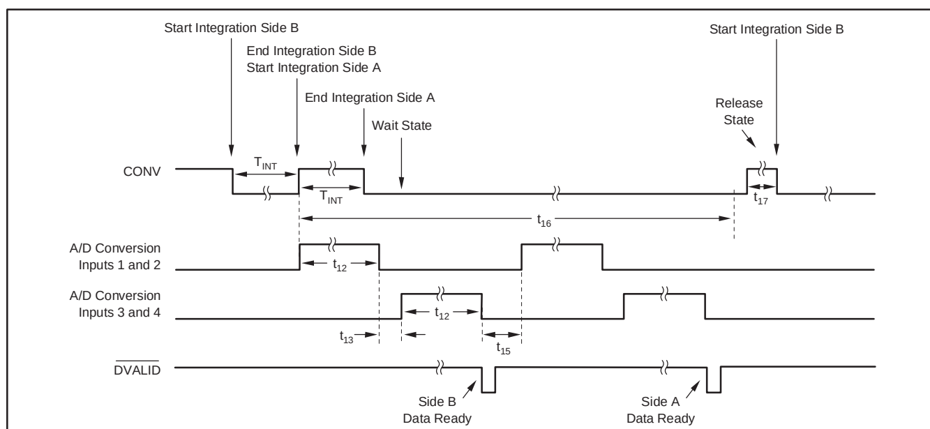
Figure 15. Internal Operation Timing Diagram of Non-Continuous Mode with Side B Integrated First
