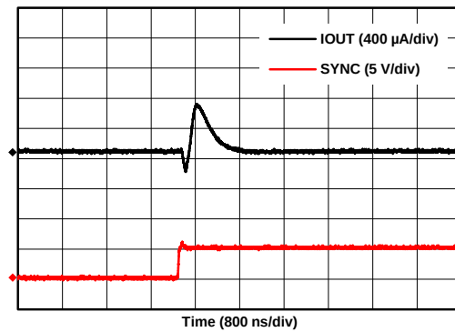
FIG 27. IOUT Full-Scale Settling Time, Falling Edge
