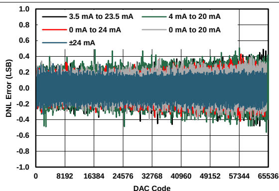
図 4. IOUT Differential Linearity Error vs Digital Input Code
