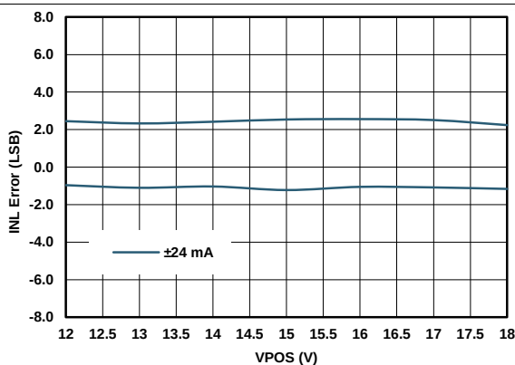
FIG 15. IOUT Linearity Error vs Power Supplies
