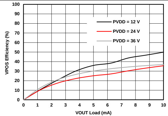
FIG 95. VPOS Efficiency (VOUT Mode) vs Load Current
