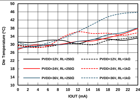
FIG 94. Internal Die Temperature (IOUT Mode) vs Load Current
