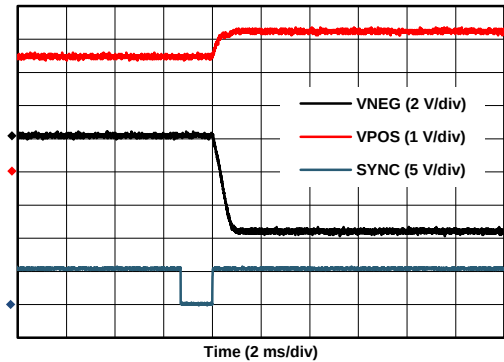
Fig. 84. Buck-Boost Converter Power-On (VOUT Mode)
