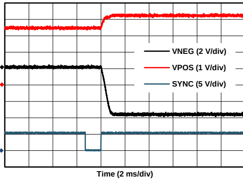
Fig. 83. Buck-Boost Converter Power-On (IOUT Mode)
