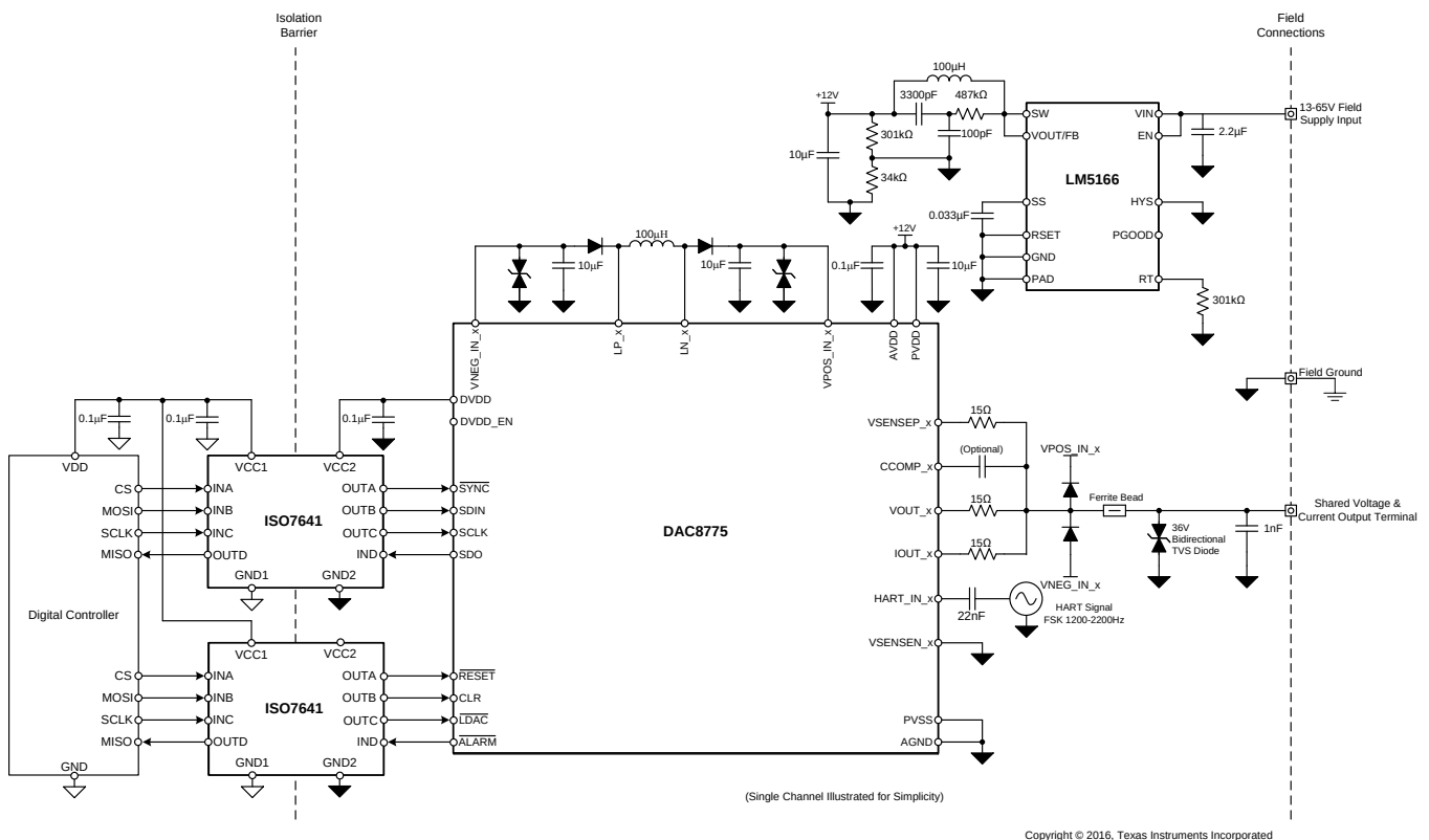
FIG 130. DAC8775 in Quad-Channel PLC AO Module
