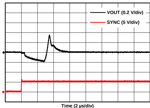
FIG 65. VOUT Glitch Impulse, Falling Edge, 1LSB Step
