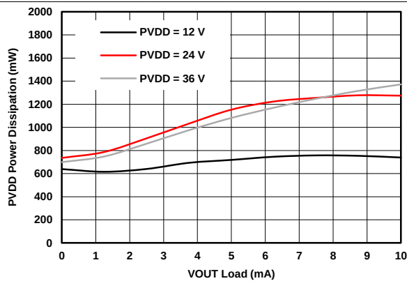
FIG 96. PVDD Power Loss (VOUT Mode) vs Load Current
