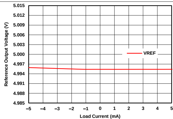
FIG 77. Internal Reference Voltage vs Load Current
