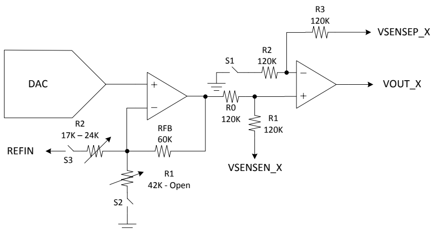
Figure 102. Voltage Output
