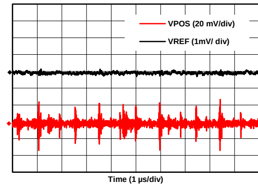
FIG 82. Internal Reference Ripple
