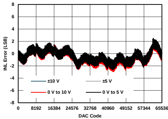
FIG 44. VOUT Linearity Error vs Digital Input Code
