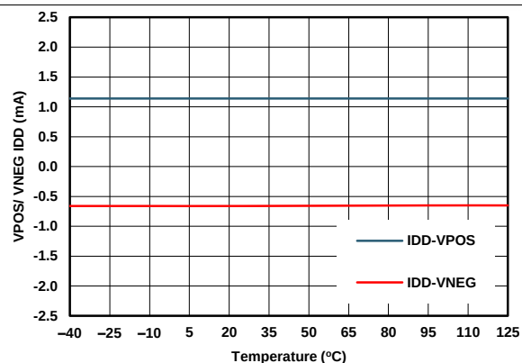
FIG 22. IOUT Power Supply Current vs Temperature
