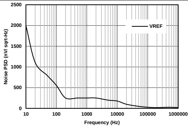
FIG 81. Internal Reference Noise Density vs Frequency
