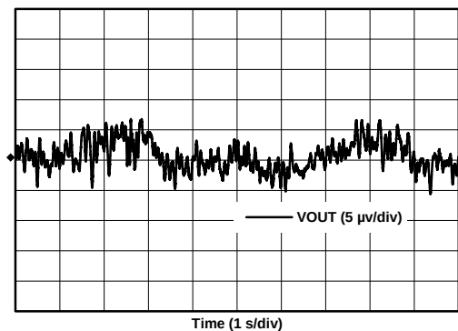
FIG 68. VOUT Noise, 0.1 Hz to 10 Hz
