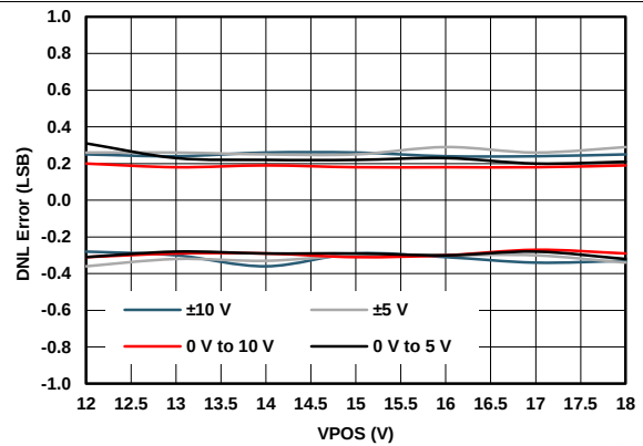
FIG 57. VOUT Differential Linearity Error vs Power Supplies
