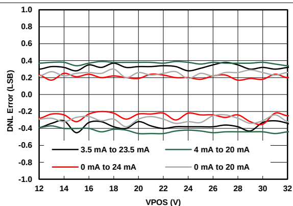
FIG 16. IOUT Differential Linearity Error vs Power Supplies
