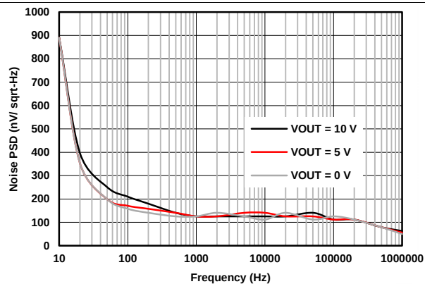
FIG 69. VOUT Noise Density vs Frequency
