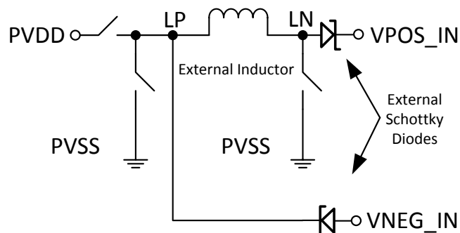
Figure 99. Buck-Boost Converter
