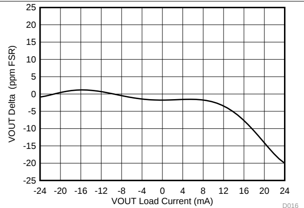
Figure 20. VOUT Load Regulation (SCLM = 11)
