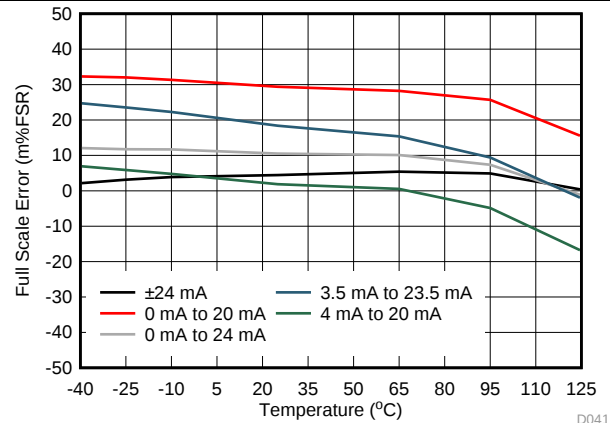
图 45. IOUT Full-Scale Error vs Temperature
