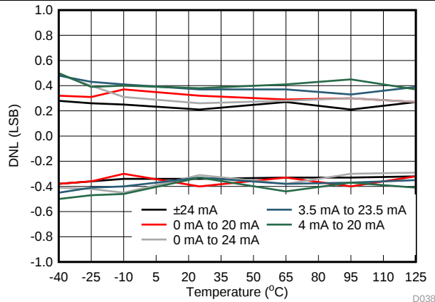
FIG 42. IOUT DNL vs Temperature
