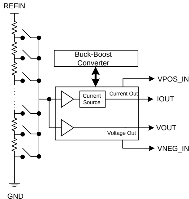
FIG 96. General Architecture
