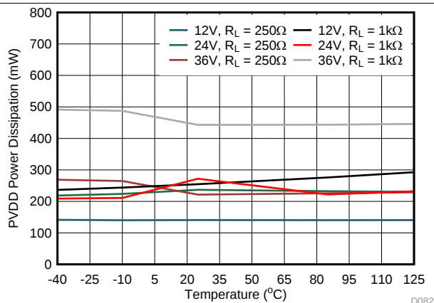
FIG 84. IOUT Power Dissipation vs Temperature
