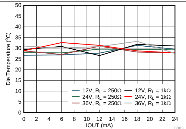
FIG 85. IOUT Die Temperature vs Load
