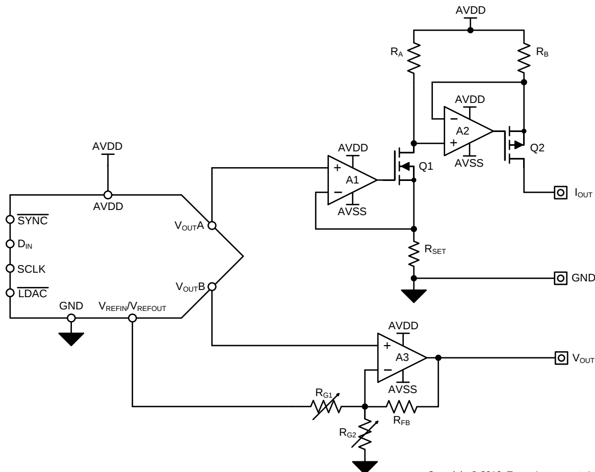
126. Generic Design for Typical PLC Current and Voltage Outputs
