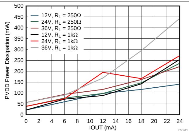
FIG 83. IOUT Power Dissipation vs Load
