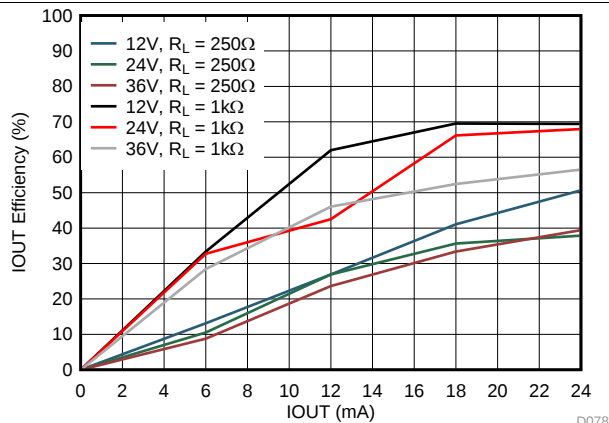
FIG 80. IOUT DC/DC Efficiency
