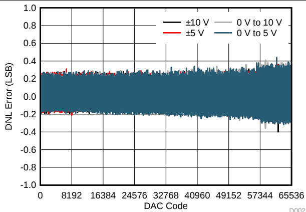
図 5. VOUT DNL vs Code (DC/DC Disabled)
