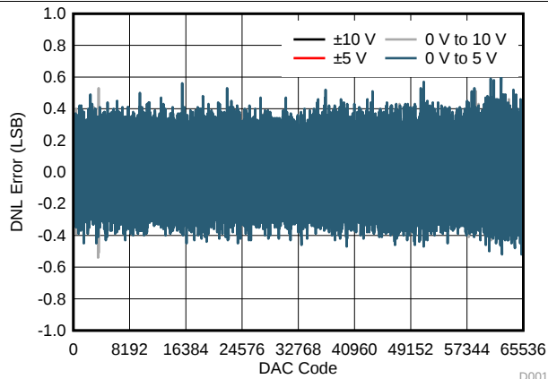
図 3. VOUT DNL vs Code (DC/DC Enabled)
