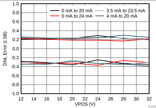
FIG 52. IOUT Unipolar Ranges DNL vs VPOS
