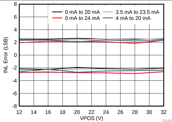
FIG 50. IOUT Unipolar Ranges INL vs VPOS
