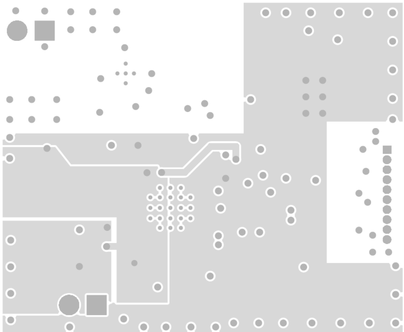
✎ 133. Example Design Internal Copper Pours
