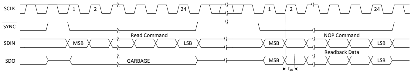
2. Readback Mode Timing
