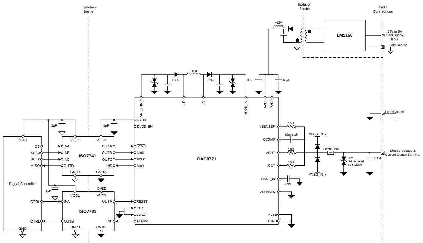
FIG 125. DAC8771 in Isolated Single-Channel PLC AO Module
