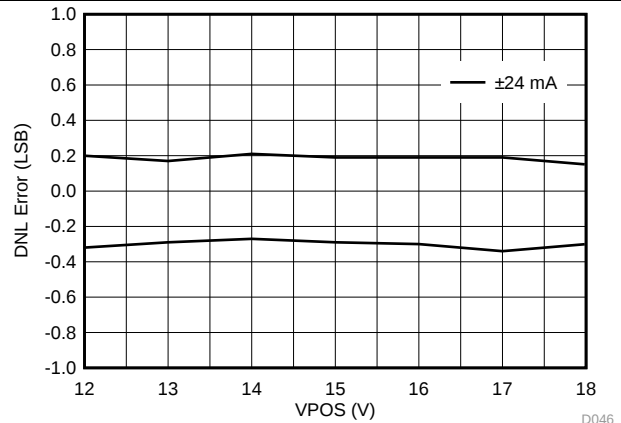
FIG 51. IOUT Bipolar Range DNL vs VPOS
