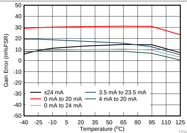
图 46. IOUT Gain Error vs Temperature
