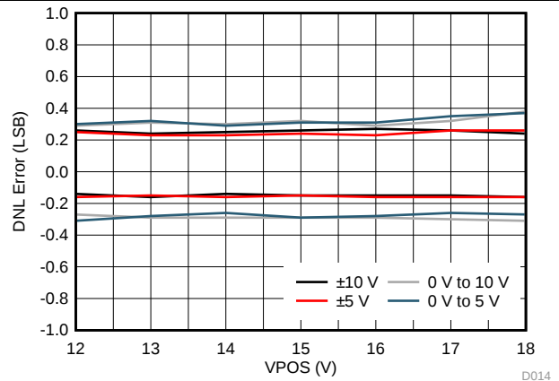
Figure 18. VOUT DNL vs VPOS
