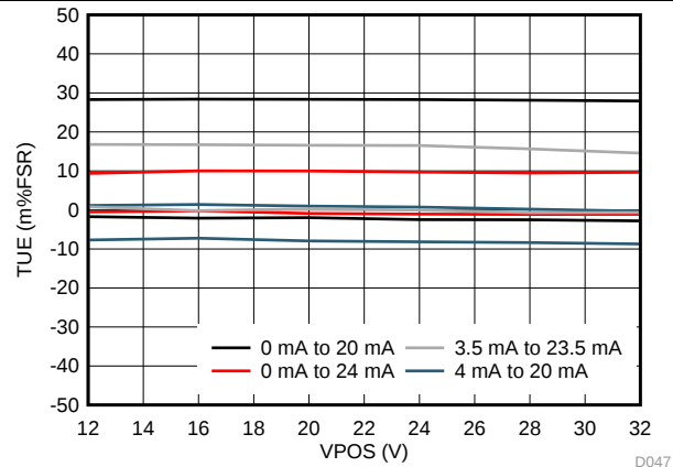
FIG 54. IOUT Unipolar Ranges TUE vs VPOS
