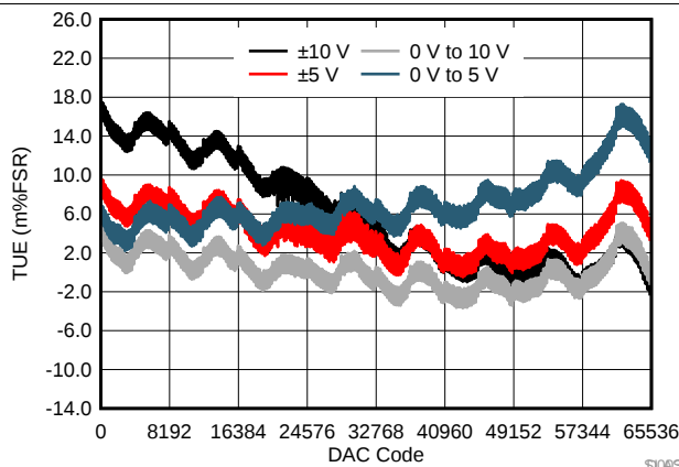
図 7. VOUT TUE vs Code (DC/DC Enabled)
