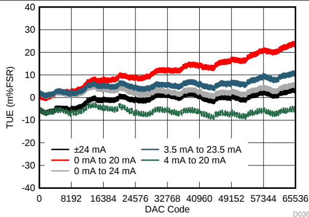
FIG 40. IOUT TUE vs Code (DC/DC Enabled)
