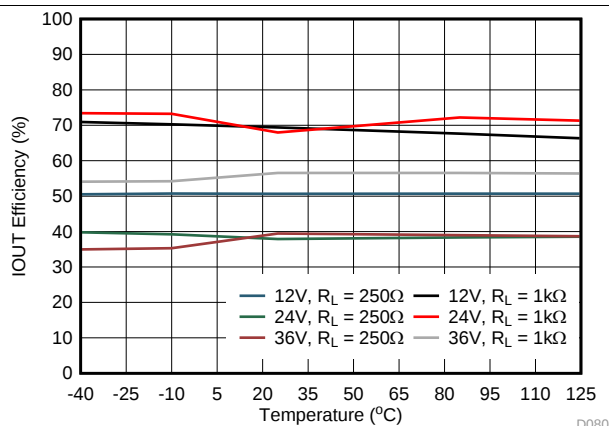
FIG 82. IOUT DC/DC Efficiency vs Temperature
