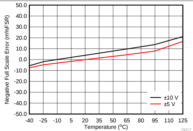
Figure 16. VOUT Negative Full-Scale Error vs Temperature
