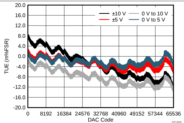
図 8. VOUT TUE vs Code (DC/DC Disabled)
