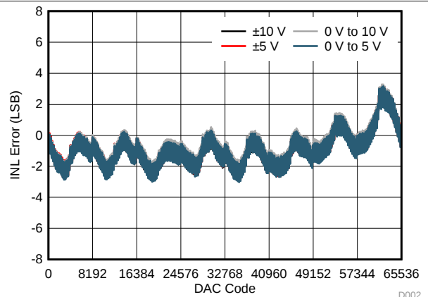
図 6. VOUT INL vs Code (DC/DC Disabled)
