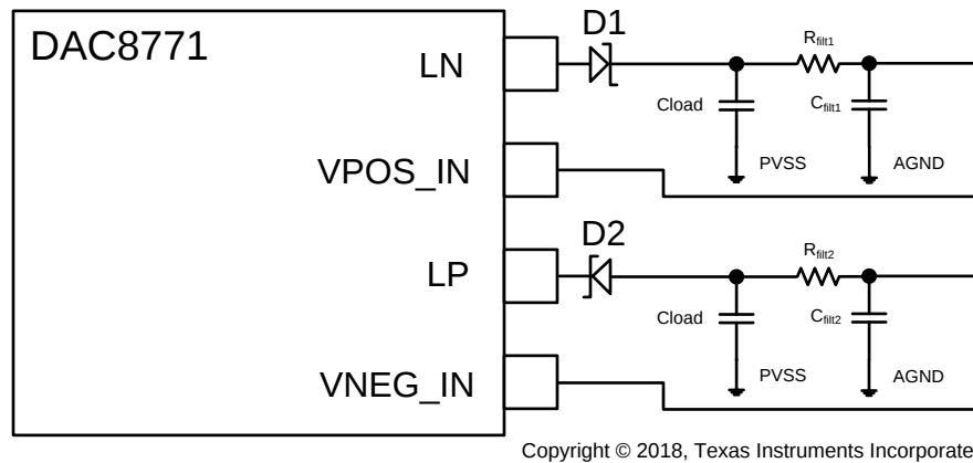
FIG 100. Buck-Boost Converter Positive and Negative Outputs
