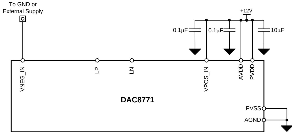
131. DAC8771 With External Supplies
