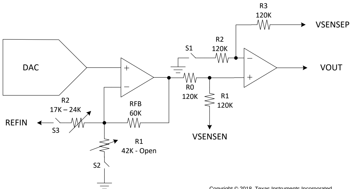
Figure 98. Voltage Output
