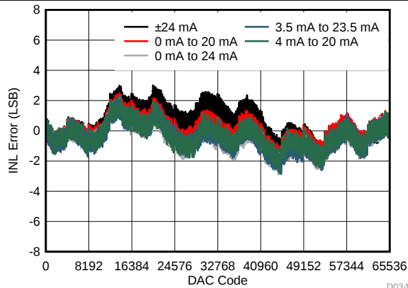
FIG 38. IOUT INL vs Code (DC/DC Disabled)
