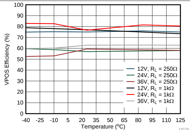
FIG 81. VPOS Efficiency vs Temperature
