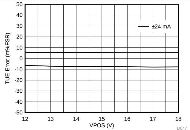
FIG 53. IOUT Bipolar Range TUE vs VPOS
