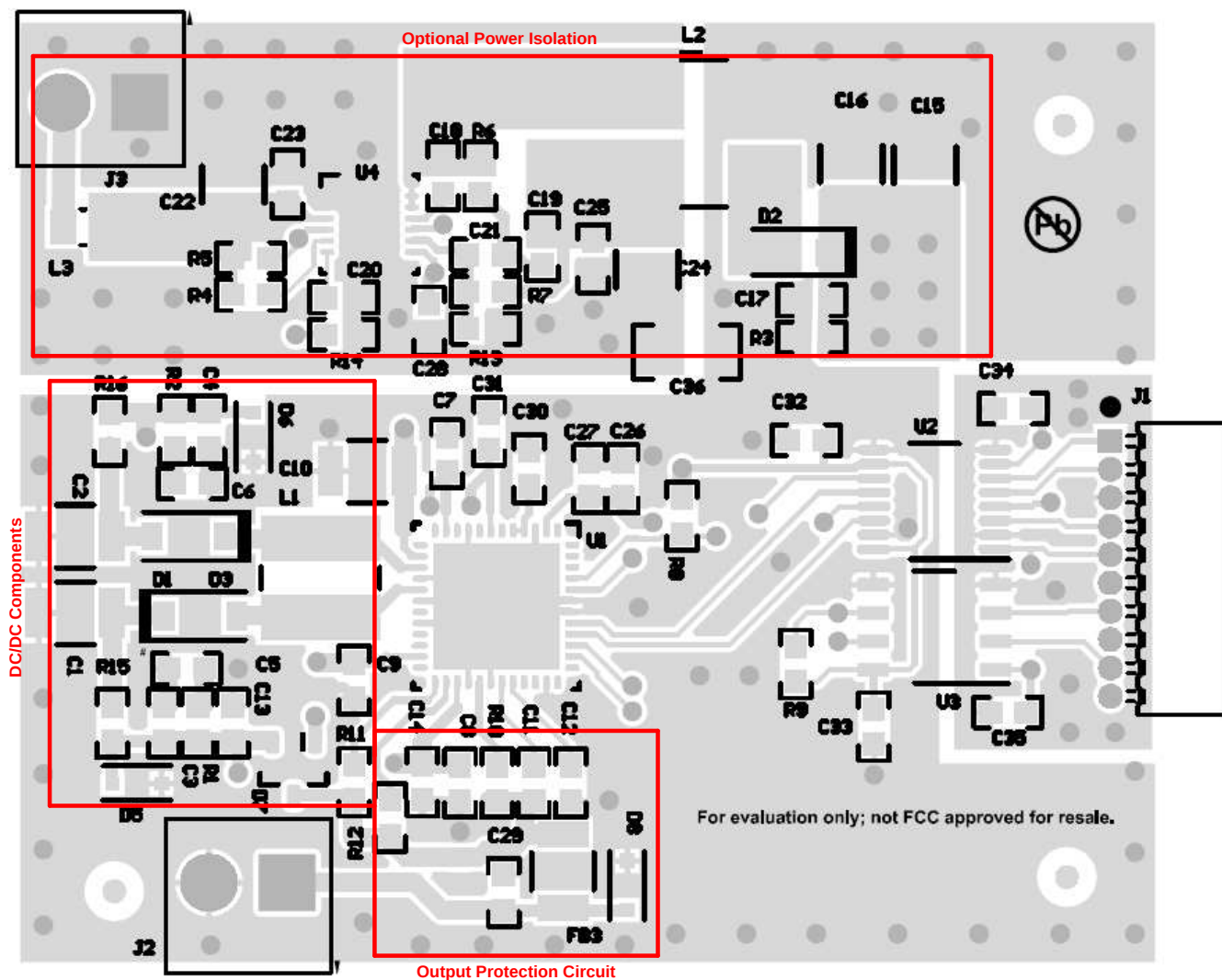
FIG 132. Application Example Layout
