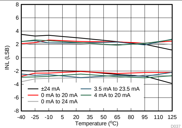
FIG 41. IOUT INL vs Temperature
