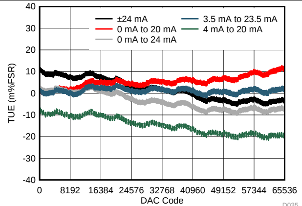
FIG 39. IOUT TUE vs Code (DC/DC Enabled)
