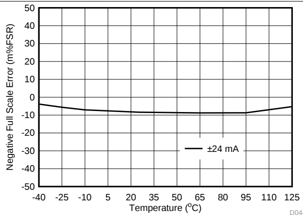
图 48. IOUT Negative Full-Scale Error vs Temperature
