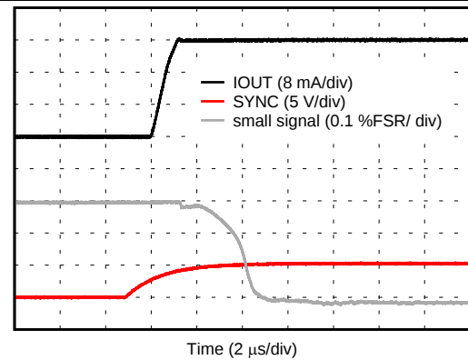
FIG 55. IOUT Settling Time, Rising Signal
