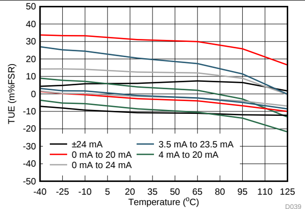
FIG 43. IOUT TUE vs Temperature
