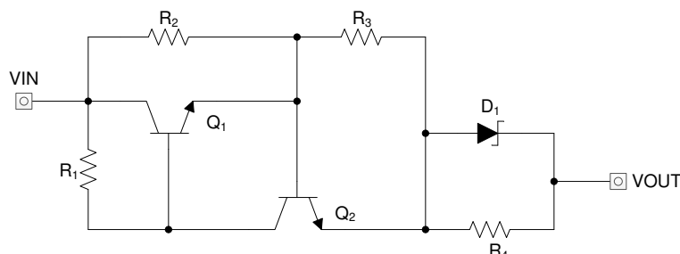
Figure 9-5. Unidirectional Current Limiter Circuit
