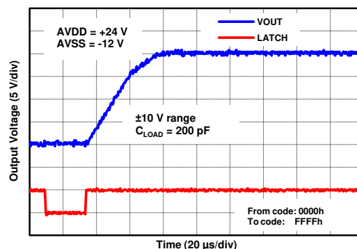
7-34. BP10V Rising
