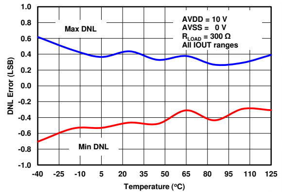
FIG 7-64. IOUT DNL vs Temperature (External R_{SET} )
