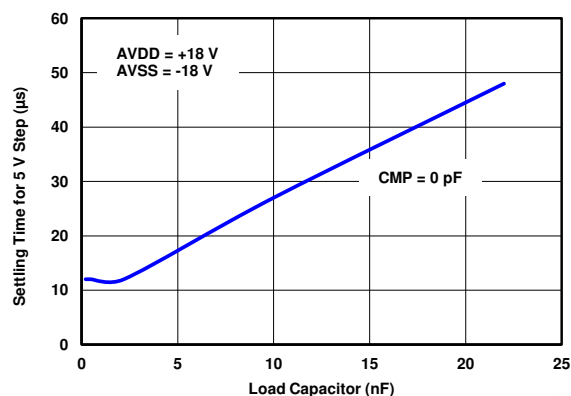
7-36. VOUT Settling Time vs Load (No Compensation Capacitor)
