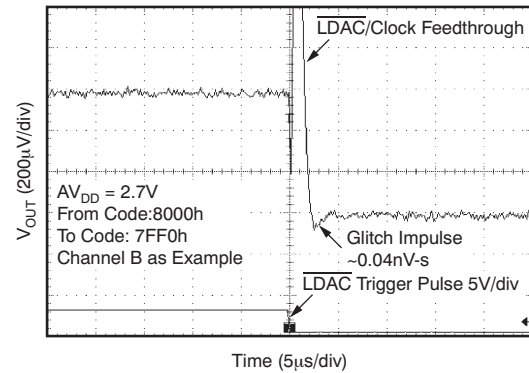
Figure 119. Glitch Energy: 2.7 V, 16-LSB Step, Falling Edge
