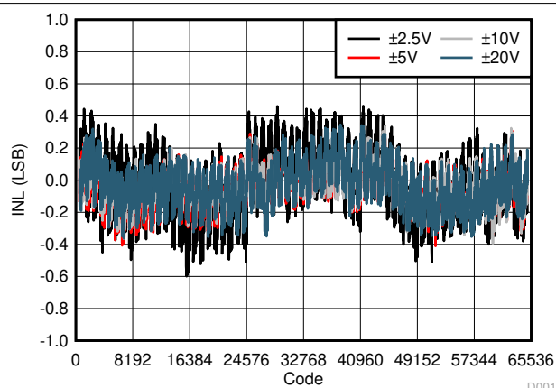
7-3. Integral Linearity Error vs Digital Input Code (Bipolar Outputs)
