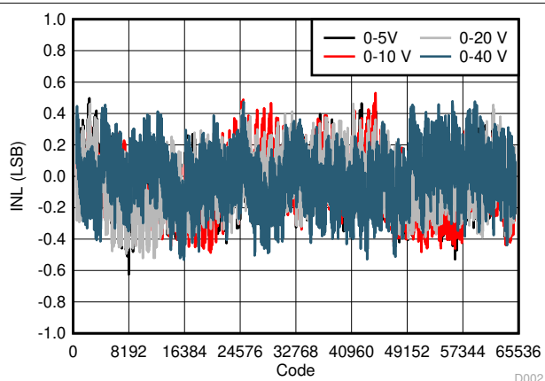
7-4. Integral Linearity Error vs Digital Input Code (Unipolar Outputs)
