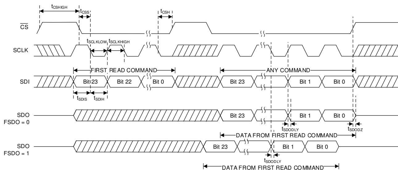
7-2. Serial Interface Read Timing Diagram
