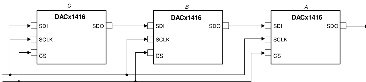
8-5. Daisy-Chain Layout
