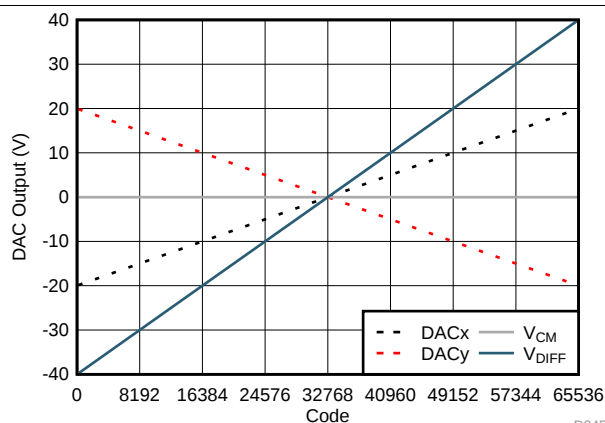
FIG 48. Differential Bipolar Output (16-Bit): \pm 20 -V Output Range
