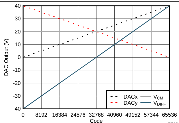
FIG 49. Differential Unipolar Output (16-Bit): 0 to 40-V Output Range
