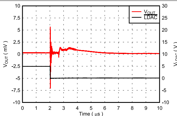
FIG 7-37. Glitch Impulse, 1 LSB Step, Falling Edge
