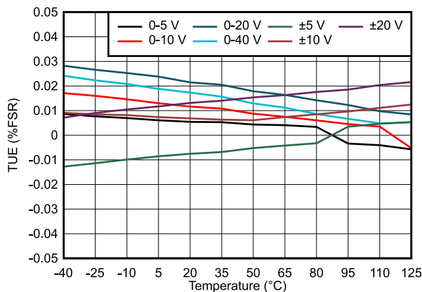
FIG 7-19. TUE vs Temperature
