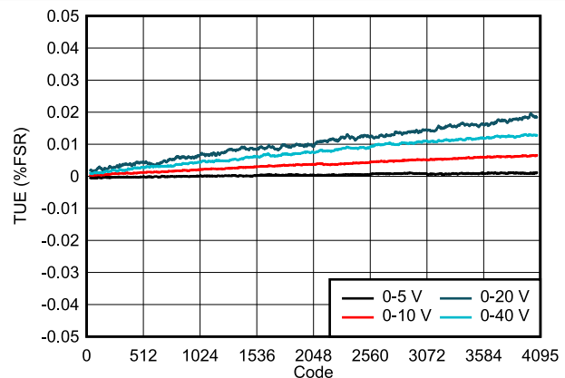
FIG 7-14. DAC61404 TUE vs Digital Input Code (Unipolar Outputs)
