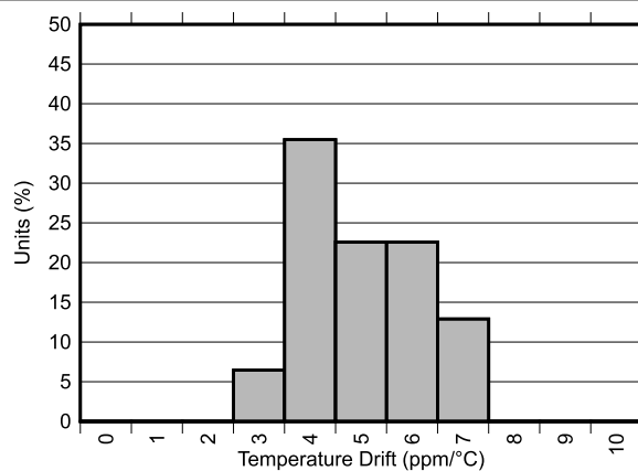
7-48. Internal Reference Temperature Drift Histogram
