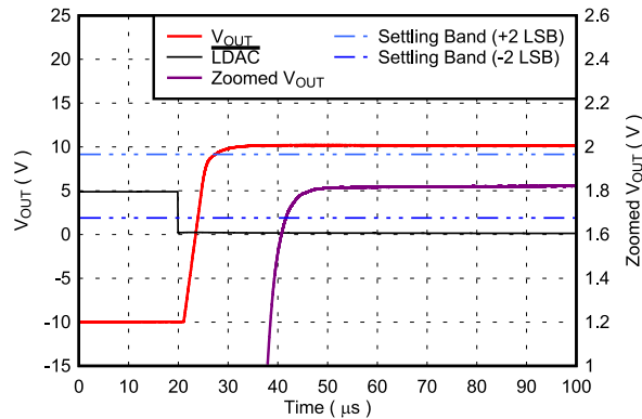
FIG 7-33. Full-Scale Settling Time, Rising Edge
