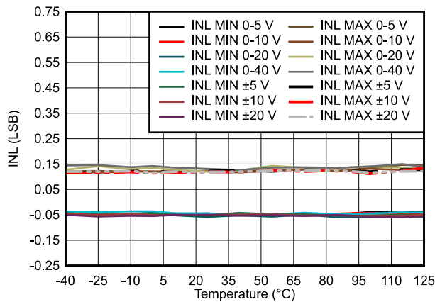
FIG 7-17. DAC61404 INL vs Temperature
