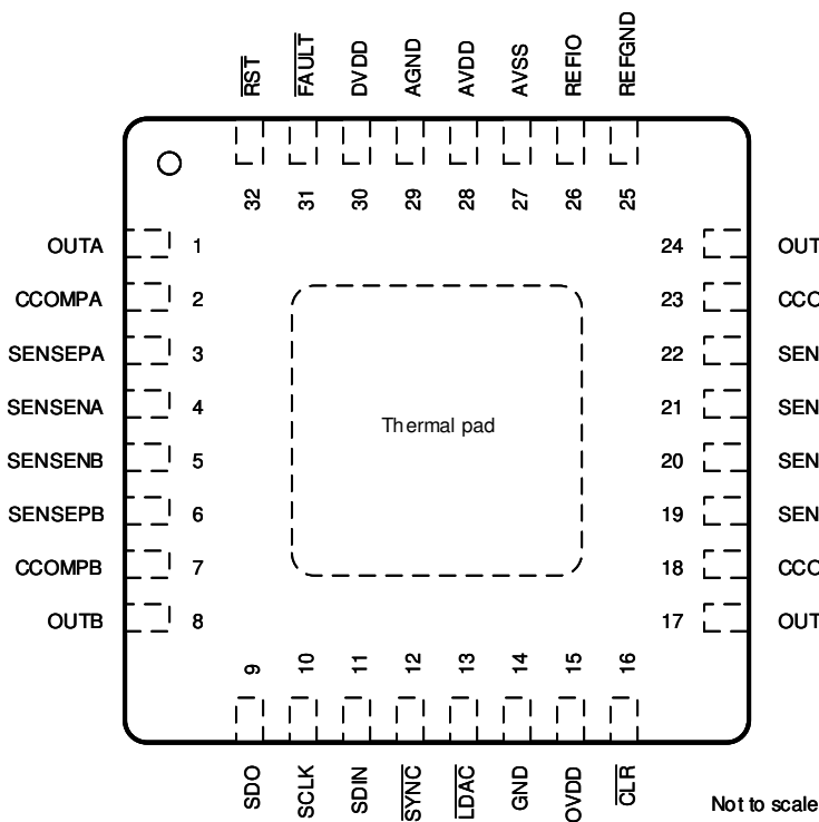
图 6-1. RHB (32-pin VQFN) Package, Top View
