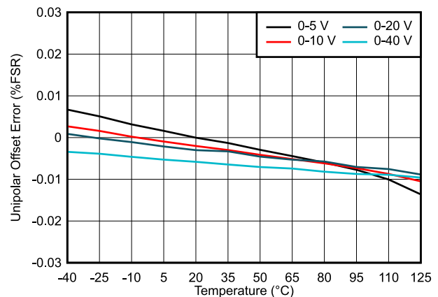
FIG 7-20. Unipolar Offset Error vs Temperature
