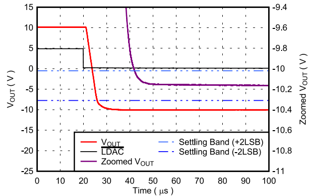
FIG 7-34. Full-Scale Settling Time, Falling Edge
