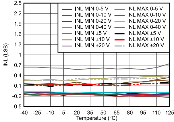
FIG 7-15. DAC81404 INL vs Temperature
