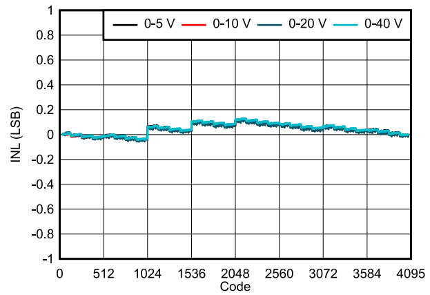
FIG 7-10. DAC61404 INL vs Digital Input Code (Unipolar Outputs)
