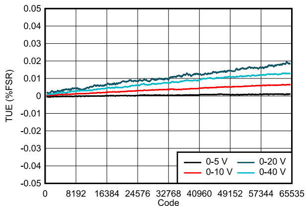
FIG 7-8. DAC81404 TUE vs Digital Input Code (Unipolar Outputs)
