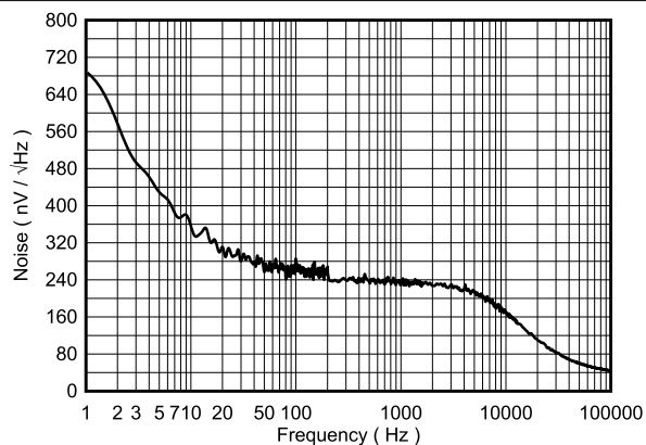
7-46. Internal Reference Noise Density vs Frequency
