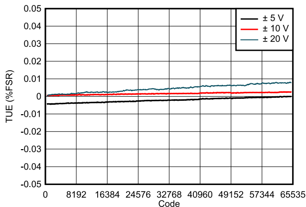
FIG 7-7. DAC81404 TUE vs Digital Input Code (Bipolar Outputs)
