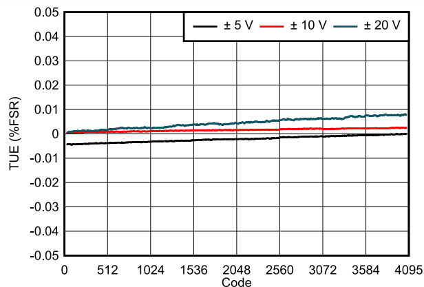
FIG 7-13. DAC61404 TUE vs Digital Input Code (Bipolar Outputs)
