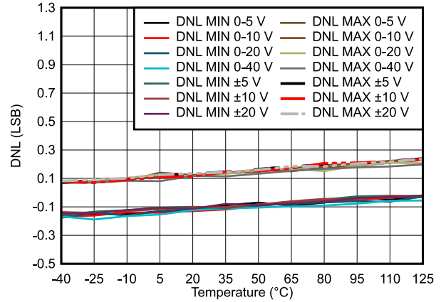
FIG 7-16. DAC81404 DNL vs Temperature
