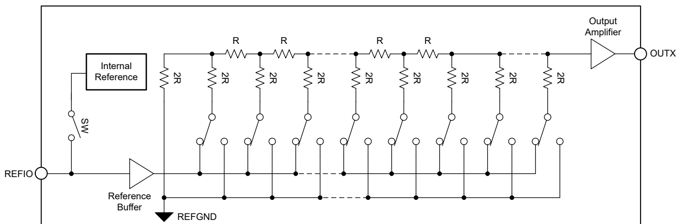
8-2. R-2R Ladder
