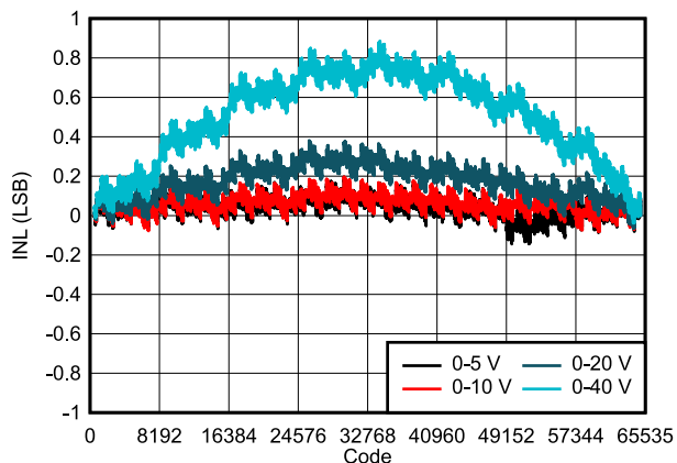
FIG 7-4. DAC81404 INL vs Digital Input Code (Unipolar Outputs)
