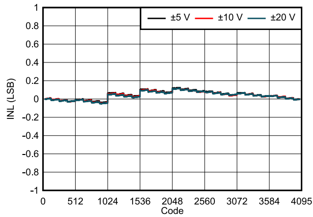
FIG 7-9. DAC61404 INL vs Digital Input Code (Bipolar Outputs)
