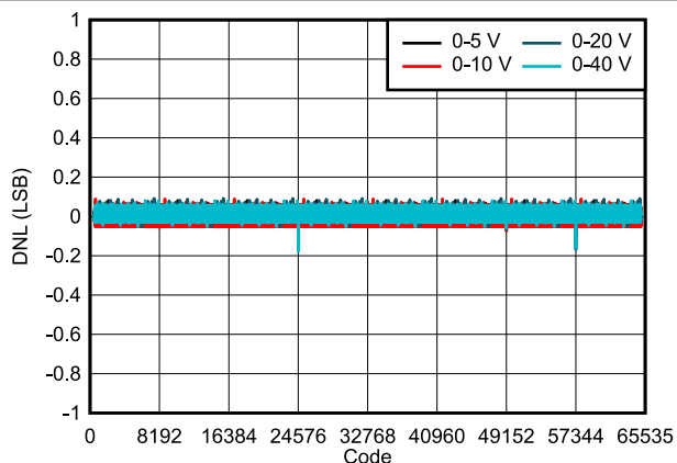
FIG 7-6. DAC81404 DNL vs Digital Input Code (Unipolar Outputs)
