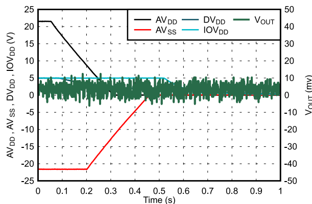
7-39. Power-Down Response
