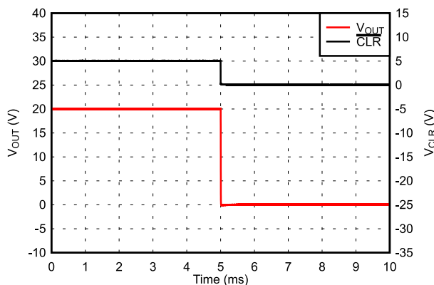
7-40. Clear Command Response
