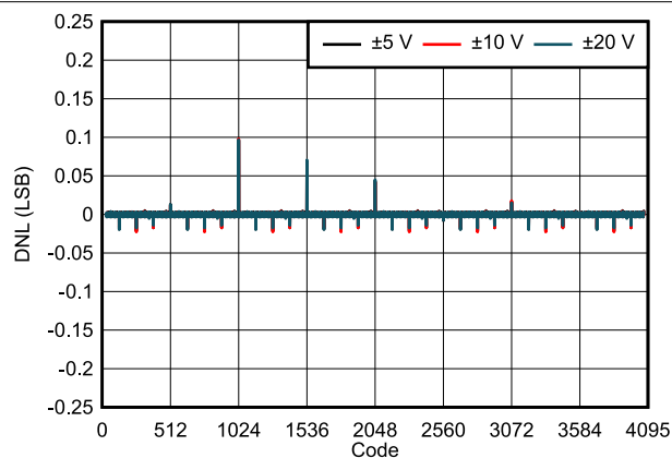
FIG 7-11. DAC61404 DNL vs Digital Input Code (Bipolar Outputs)
