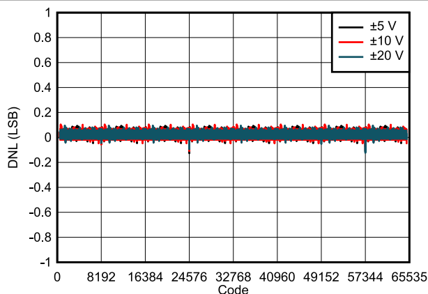
FIG 7-5. DAC81404 DNL vs Digital Input Code (Bipolar Outputs)
