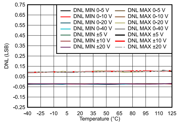
FIG 7-18. DAC61404 DNL vs Temperature
