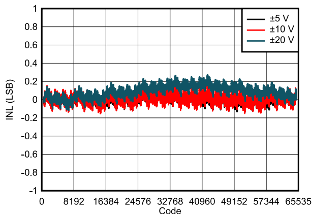
FIG 7-3. DAC81404 INL vs Digital Input Code (Bipolar Outputs)
