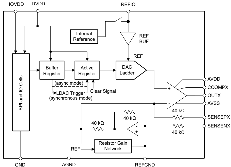
8-1. Device Architecture
