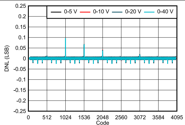
FIG 7-12. DAC61404 DNL vs Digital Input Code (Unipolar Outputs)
