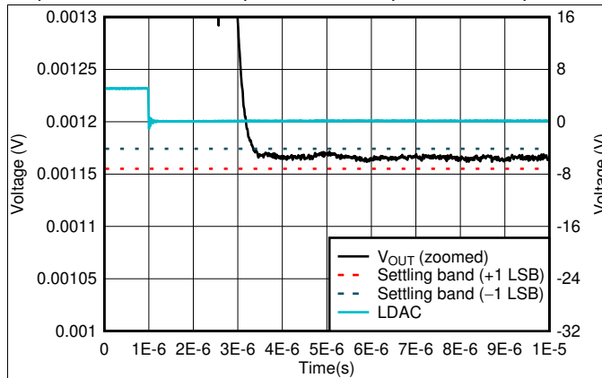
FIG 39. 100 Codes Settling Time, Falling Edge
