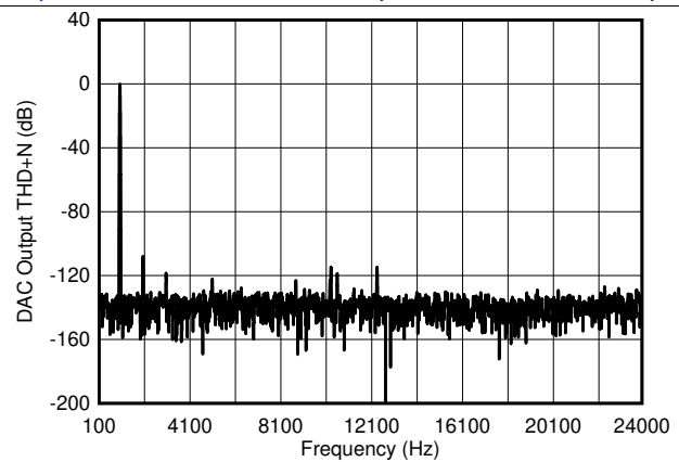
FIG 40. Total Harmonic Distortion (THD + N) vs Frequency
