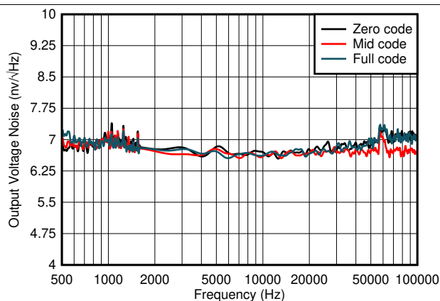
FIG 41. DAC Output Noise Spectral Density
