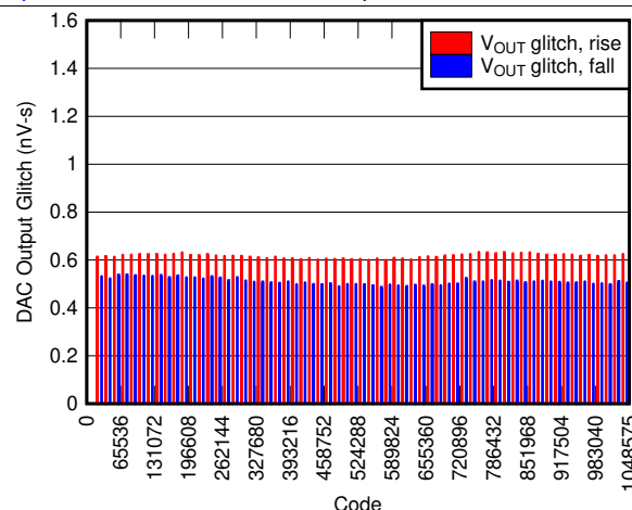
FIG 34. Segment Glitch Impulse, 1-LSB Step
