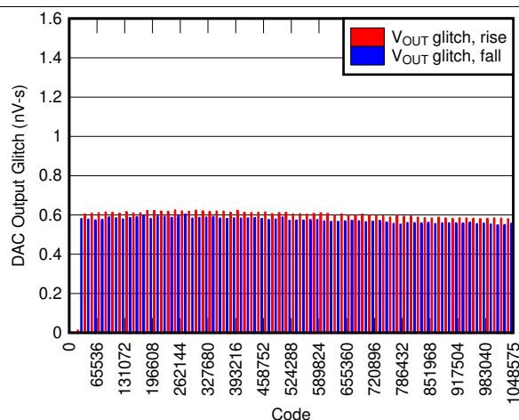
FIG 33. Segment Glitch Impulse, 1-LSB Step
