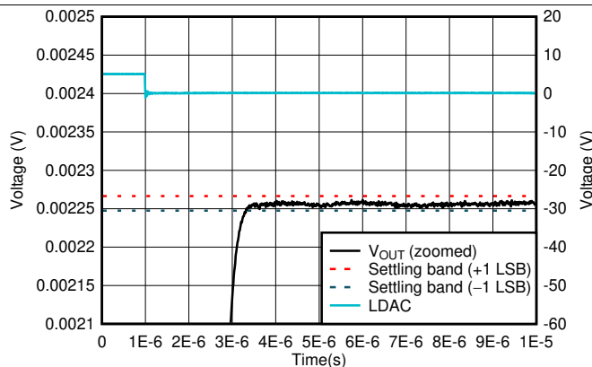
FIG 36. Full-Scale Settling Time, Rising Edge
