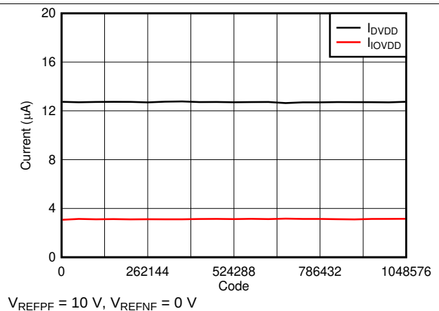
FIG 20. Supply Current ( DV_{DD} and IOV_{DD} ) vs Digital Input Code
