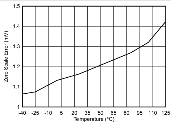
Figure 5-10. Zero-Scale Error vs Temperature
