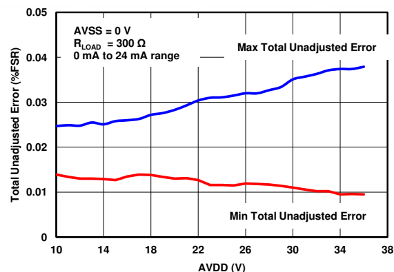
7-52. IOUT TUE vs Supply (External R_{SET} )
