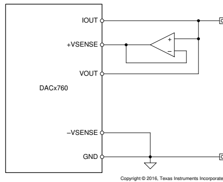
FIG 9-2. VOUT and IOUT Tied Together to One Pin
