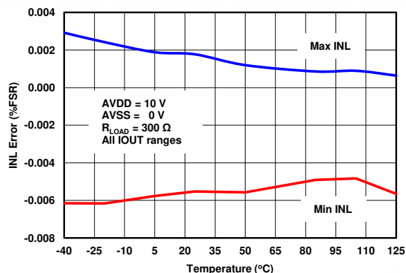
FIG 7-57. IOUT INL vs Temperature (External R_{SET} )
