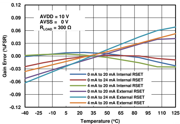
7-69. IOOUT Gain Error vs Temperature
