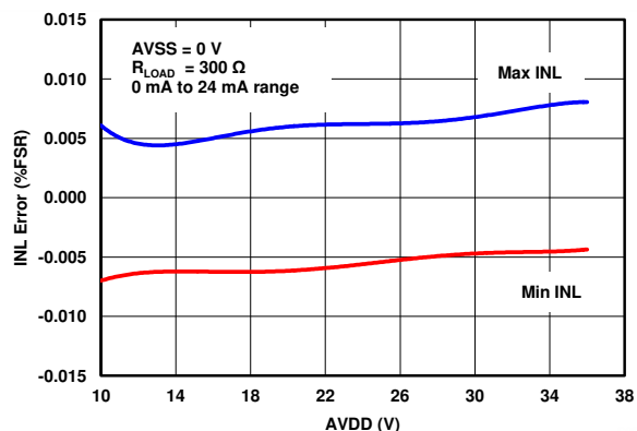
FIG 7-58. IOUT INL vs Supply (Internal R_{SET} )
