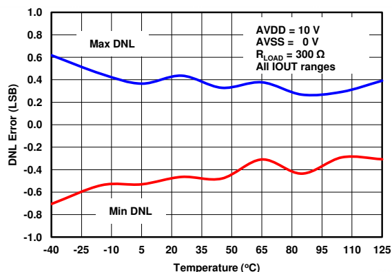
FIG 7-64. IOUT DNL vs Temperature (External R_{SET} )
