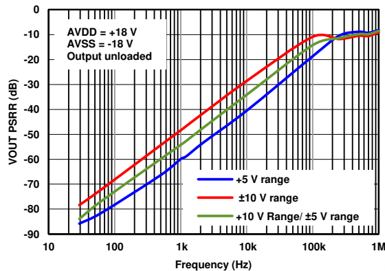
FIG 7-45. AVDD PSRR for VOUT
