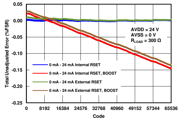
FIG 7-46. IOU TUE vs Code (0 mA to 24 mA)
