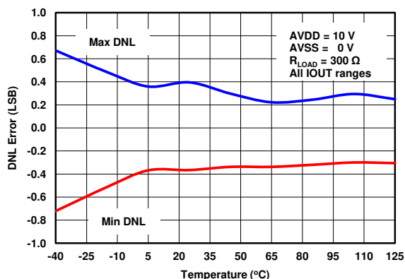
FIG 7-63. IOUT DNL vs Temperature (Internal R_{SET} )
