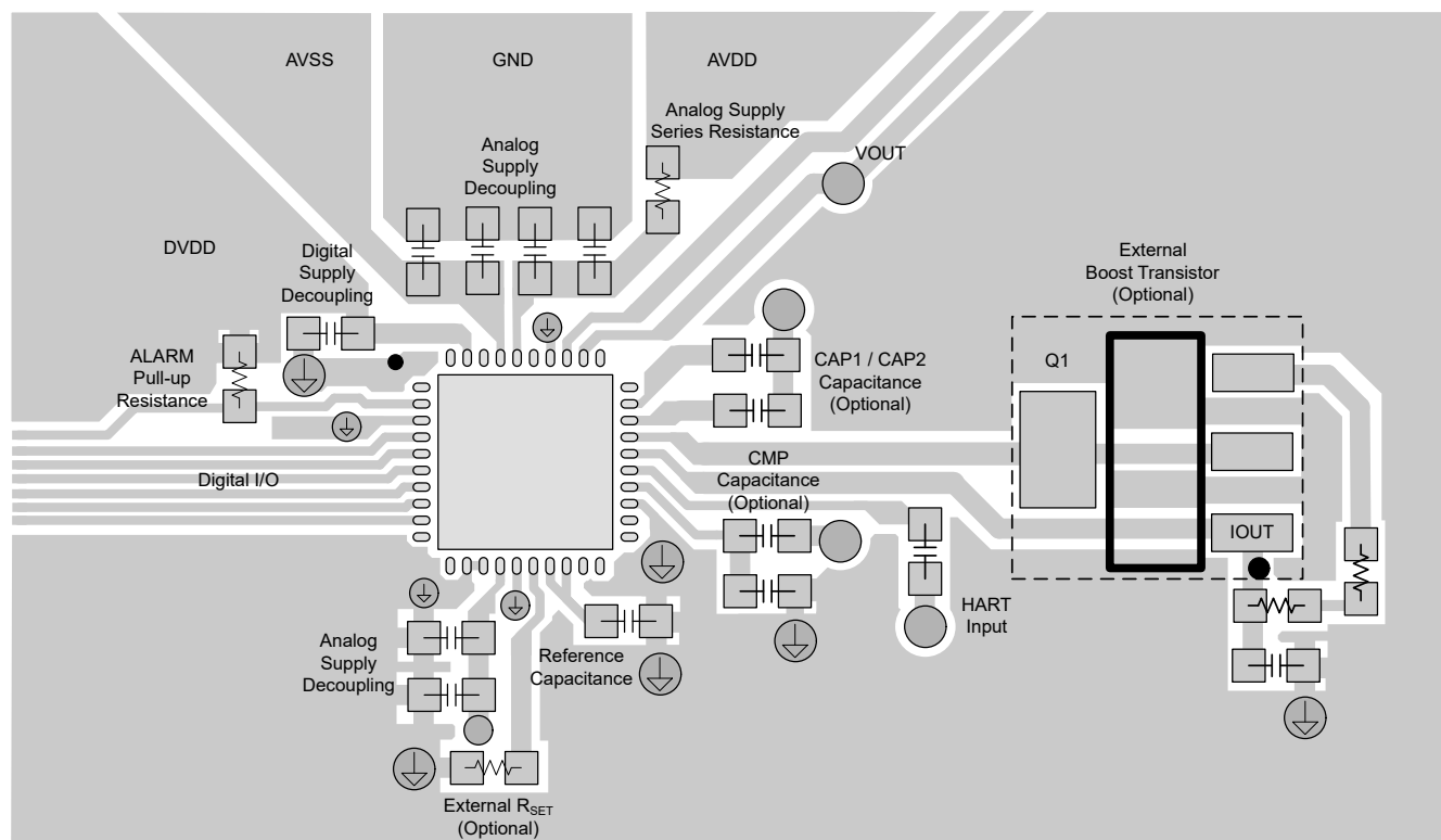
✎ 11-1. DACx760 Layout Example
