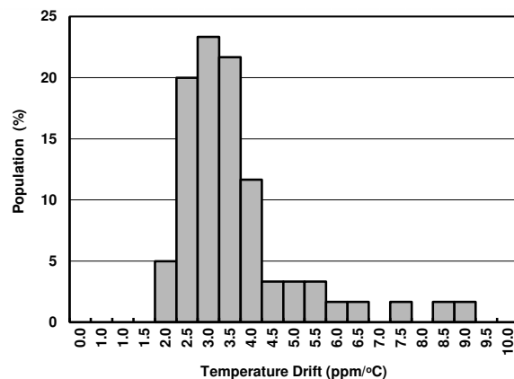
7-4. Internal Reference Temperature Drift Histogram
