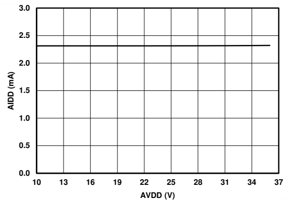
7-10. AIIDD vs AVDD
