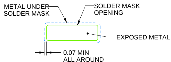
SOLDER MASK DETAILS
