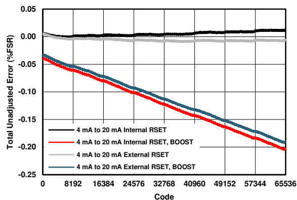
FIG 7-16. IOUT TUE vs Code (4 mA to 20 mA)
