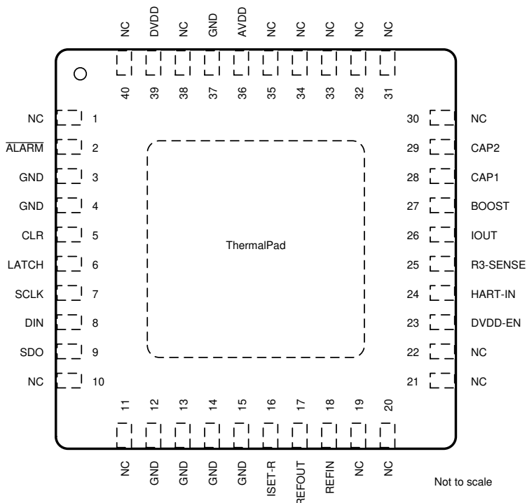
6-1. RHA Package, 40-Pin VQFN, Top View
