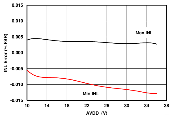
FIG 7-27. IOUT INL vs Supply (External R_{SET} )
