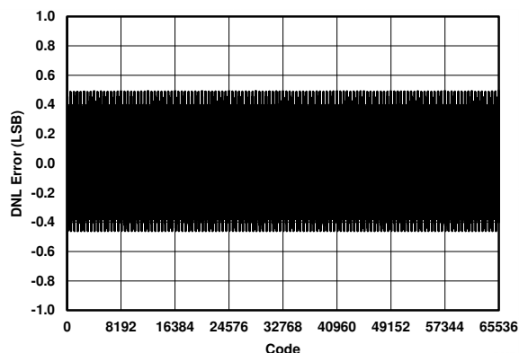
FIG 7-28. IOUT DNL vs Code (0 mA to 24 mA)
