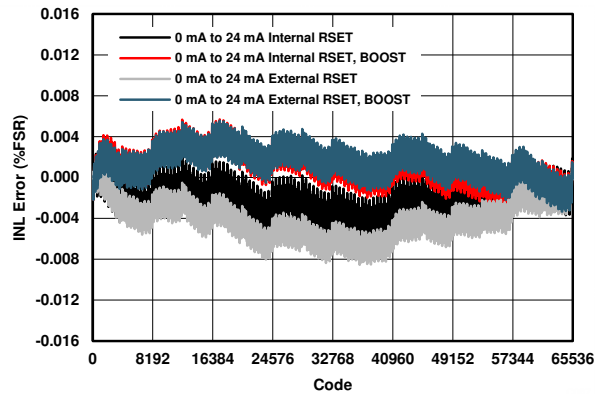
FIG 7-21. IOUT INL vs Code (0 mA to 24 mA)
