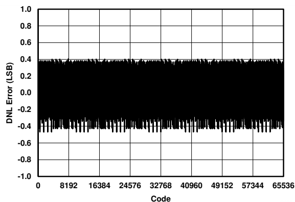
FIG 7-28. IOUT DNL vs Code (0 mA to 24 mA)
