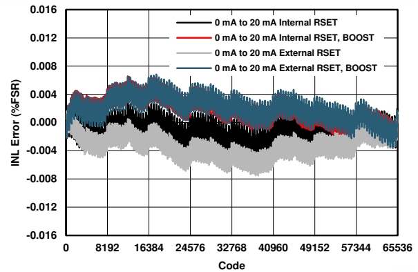
FIG 7-22. IOUT INL vs Code (0 mA to 20 mA)
