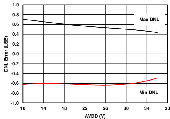
FIG 7-33. IOOUT DNL vs Supply (Internal R_{SET} )
