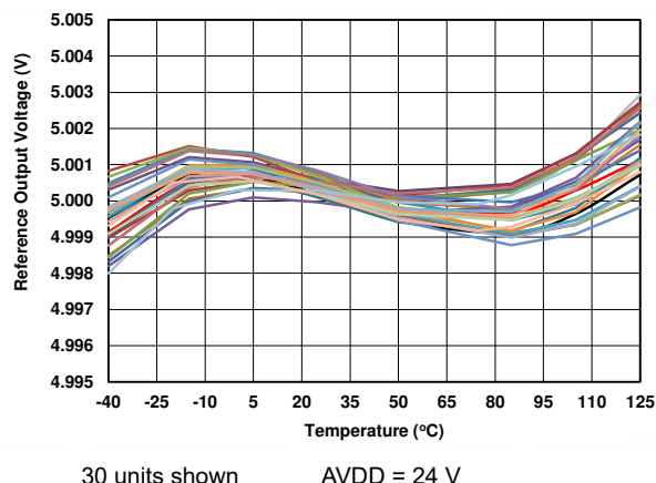
7-3. REFOUT vs Temperature
