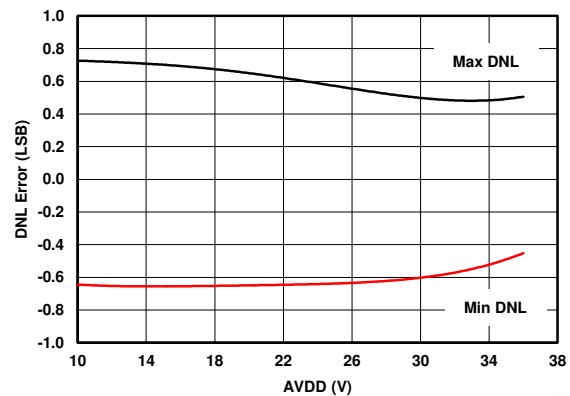
FIG 7-34. IOOUT DNL vs Supply (External R_{SET} )
