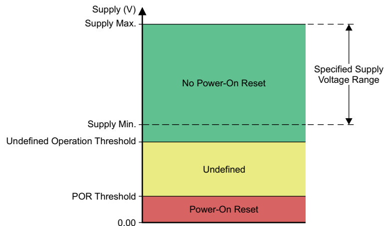
FIG 8-3. Relevant Voltage Levels for POR Circuit
