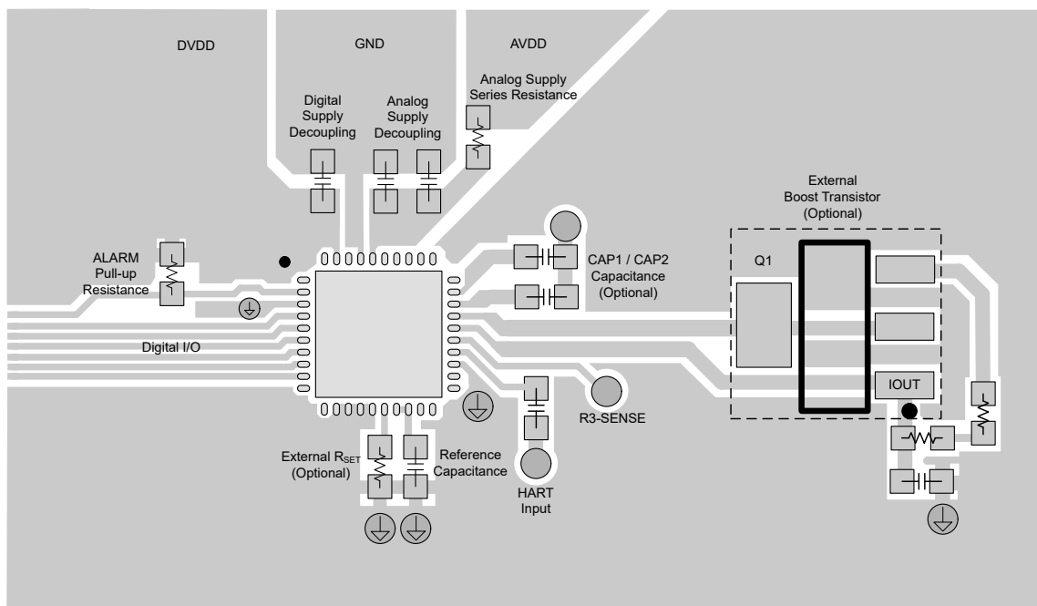
☒ 11-1. Example Layout
