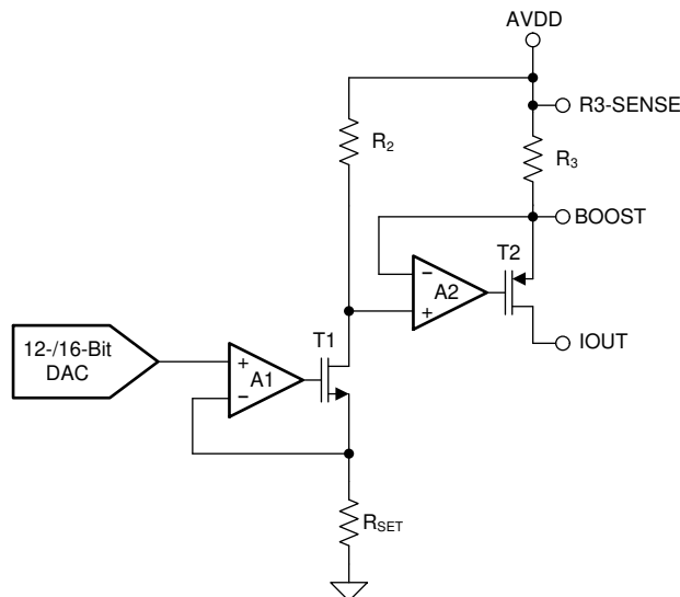
Figure 8-2. Current Output
