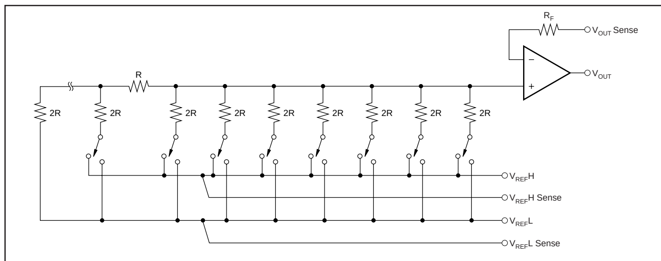
FIGURE 1. DAC7744 Architecture.
