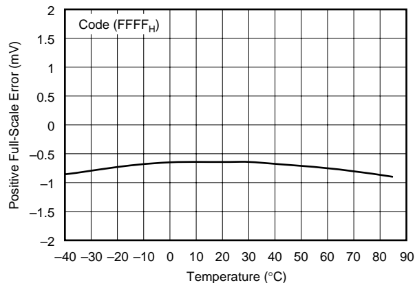
POSITIVE FULL-SCALE ERROR vs TEMPERATURE
