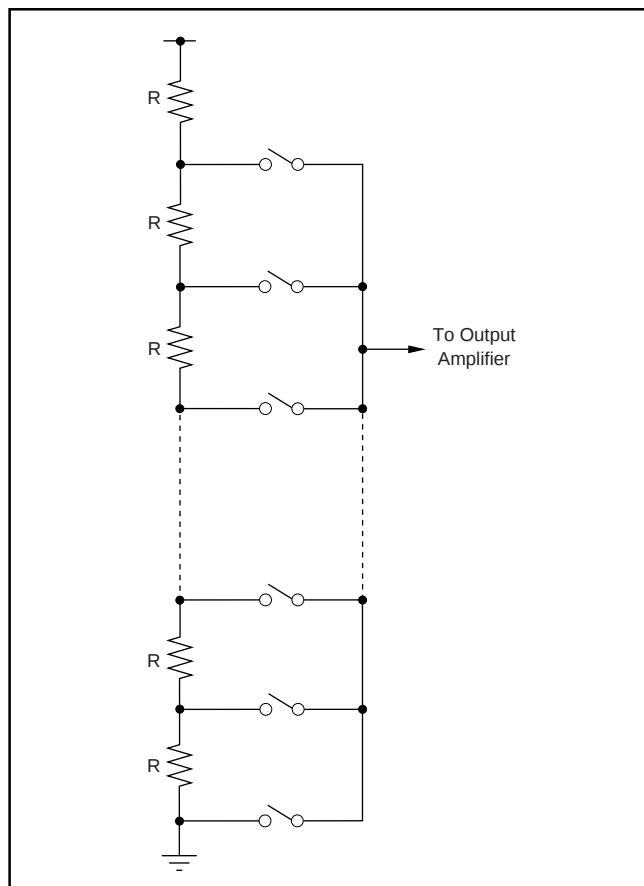
FIGURE 2. Resistor String.
