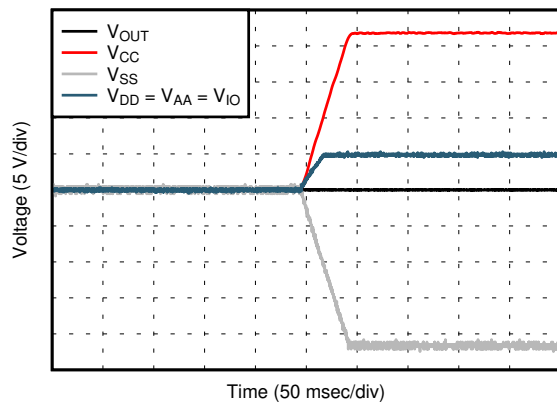
7-35. Power-Up Response
