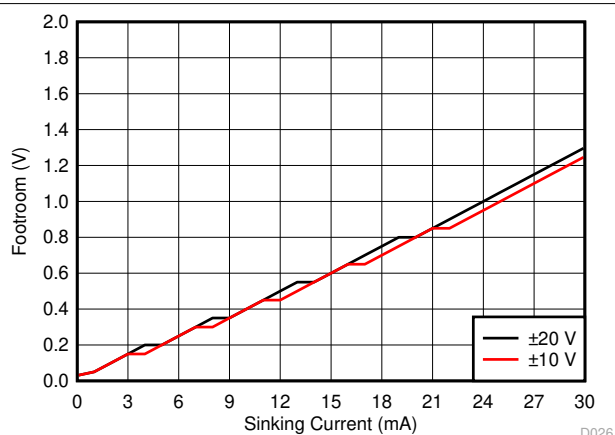
7-28. V_{SS} Footroom vs Sinking Current
