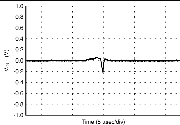
7-29. Full-Scale Settling Time, Rising Edge
