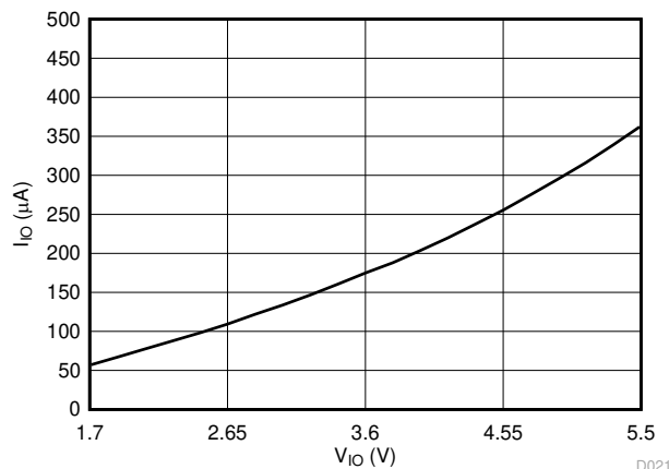
Figure 7-23. Supply Current ( I_{LO} ) vs Supply Voltage
