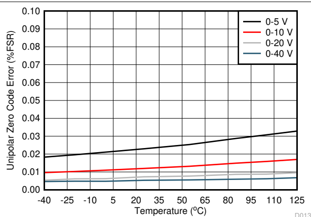
Figure 7-15. Unipolar Zero Code Error vs Temperature
