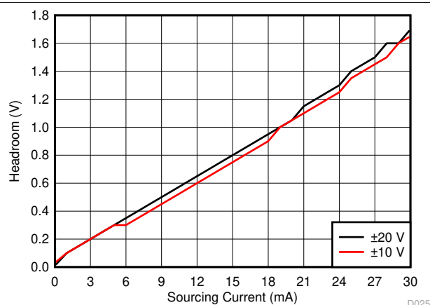
7-27. V_{CC} Headroom vs Sourcing Current
