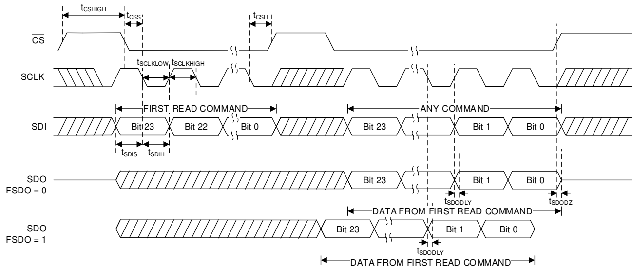
7-2. Serial Interface Read Timing Diagram
