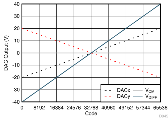
FIG 8-2. Differential Bipolar Output (16-Bit): ±20-V Output Range
