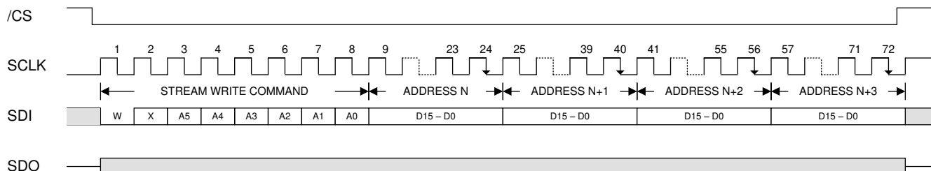
FIG 8-4. Serial Interface Streaming Cycle
