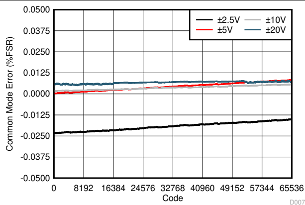
FIG 7-9. Common Mode Error vs Digital Input Code (Differential Bipolar Outputs)
