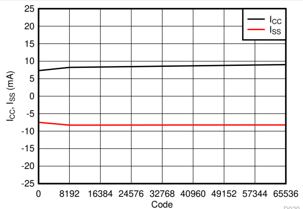
Figure 7-22. Supply Current ( I_{CC} , I_{SS} ) vs Digital Input Code
