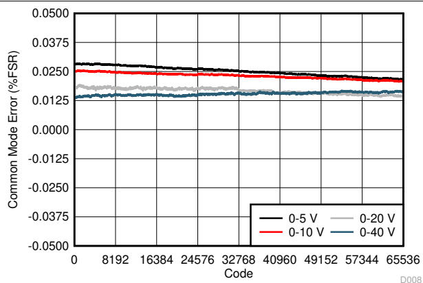
FIG 7-10. Common Mode Error vs Digital Input Code (Differential Unipolar Outputs)
