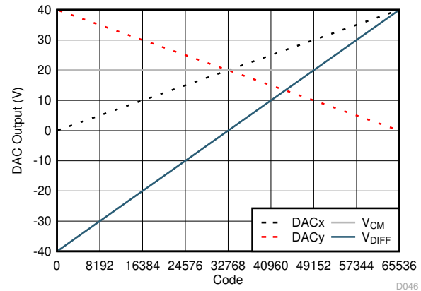
FIG 8-3. Differential Unipolar Output (16-Bit): 0-V to 40-V Output Range
