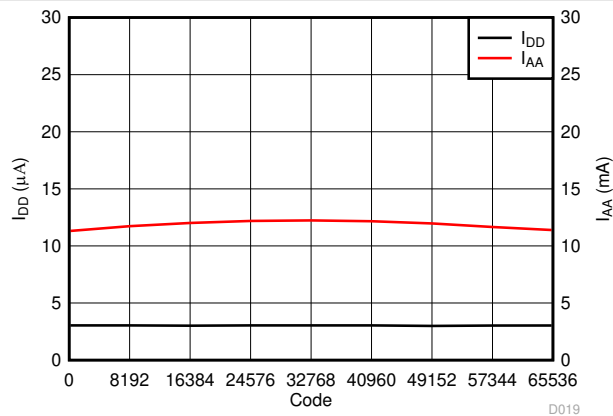
Figure 7-21. Supply Current ( I_{DD} , I_{AA} ) vs Digital Input Code
