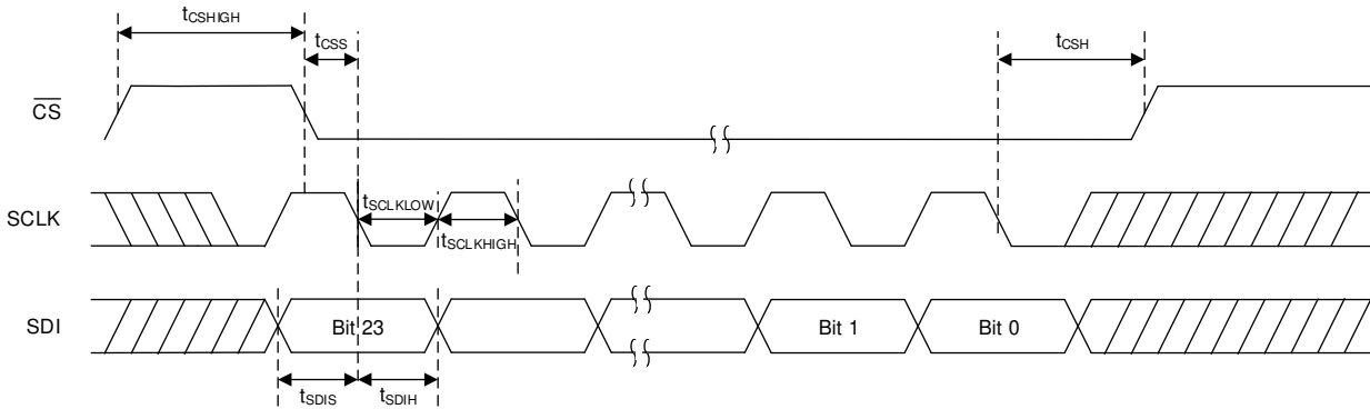
7-1. Serial Interface Write Timing Diagram
