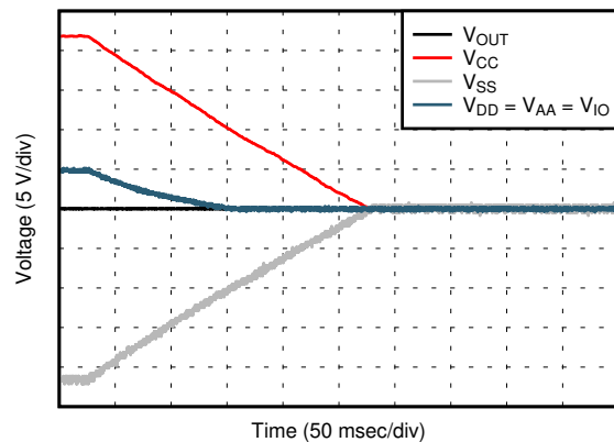
7-36. Power-Down Response
