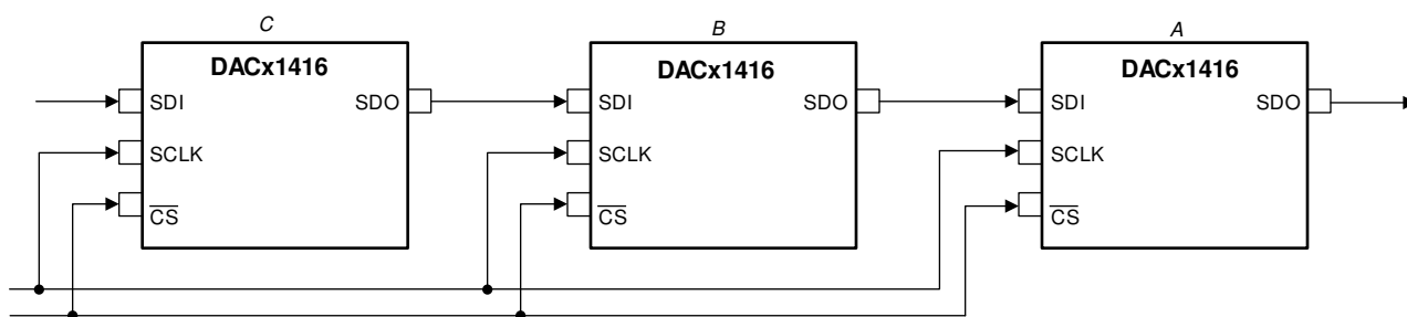
FIG 8-5. Daisy-Chain Layout
