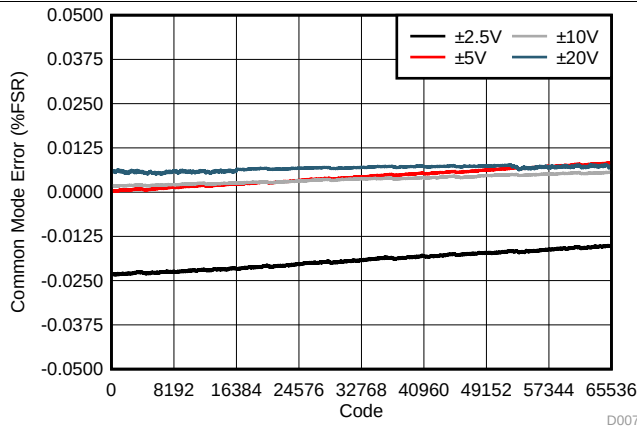
FIG 7. Common Mode Error vs Digital Input Code (Differential Bipolar Outputs)
