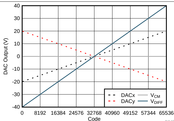
Figure 48. Differential Bipolar Output (16-Bit): ±20-V Output Range
