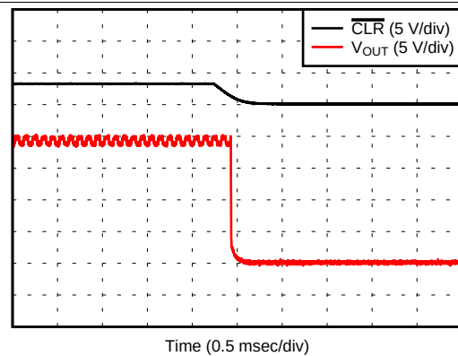
✎ 34. Power-Down Response
