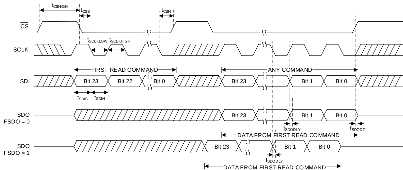
46. Serial Interface Read Timing Diagram
