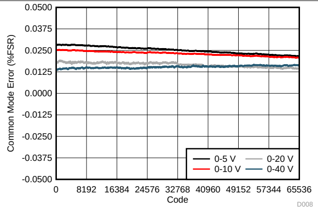
FIG 8. Common Mode Error vs Digital Input Code (Differential Unipolar Outputs)
