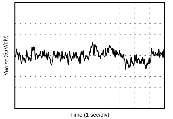
Figure 43. Internal Reference Noise
