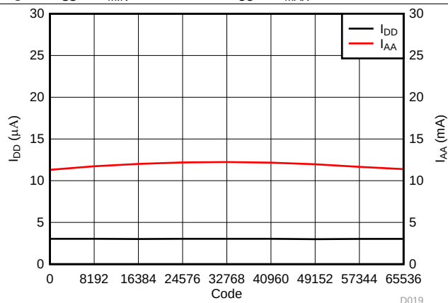
FIG 19. Supply Current ( I_{DD} , I_{AA} ) vs Digital Input Code
