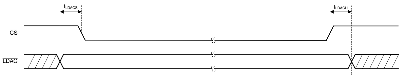
Figure 64. Digital Logic Timing Diagram
