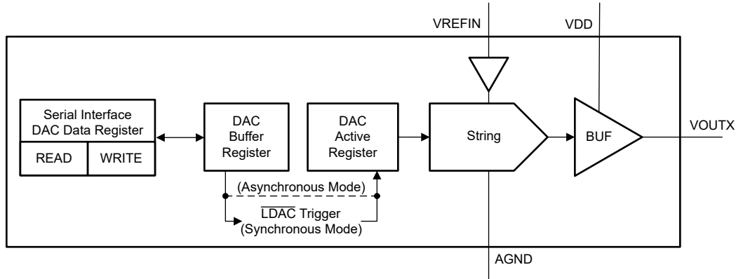
図 6-1. DACx3508 DAC Architecture
