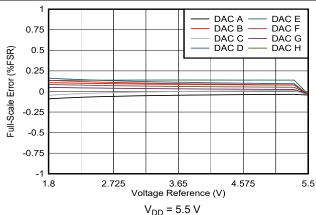
図 5-35. Full-Scale Error vs Voltage Reference
