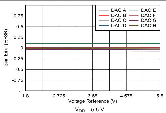
図 5-31. Gain Error vs Voltage Reference
