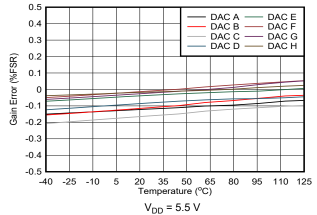
図 5-29. Gain Error vs Temperature
