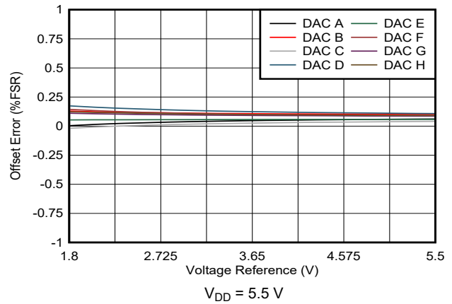
図 5-27. Offset Error vs Voltage Reference
