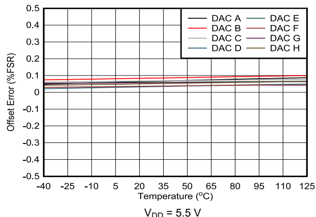
Figure 5-25. Offset Error vs Temperature
