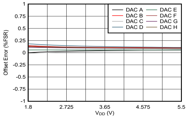
図 5-26. Offset Error vs Supply Voltage
