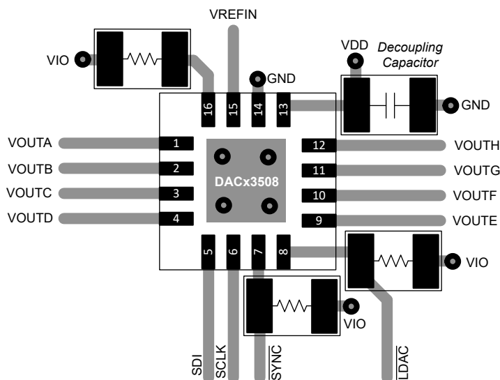
Figure 8-5. Layout Example
