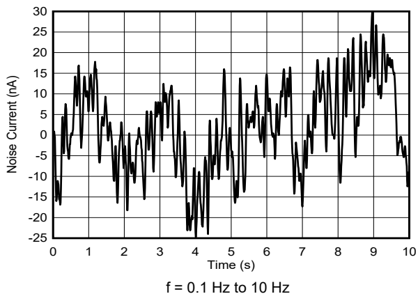
6-50. Current Output Flicker Noise
