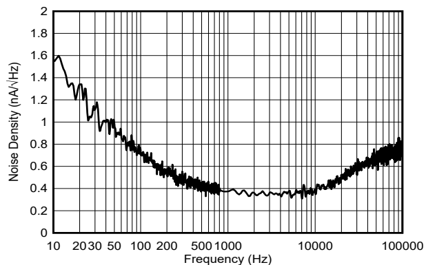
6-49. Current Output Noise Density
