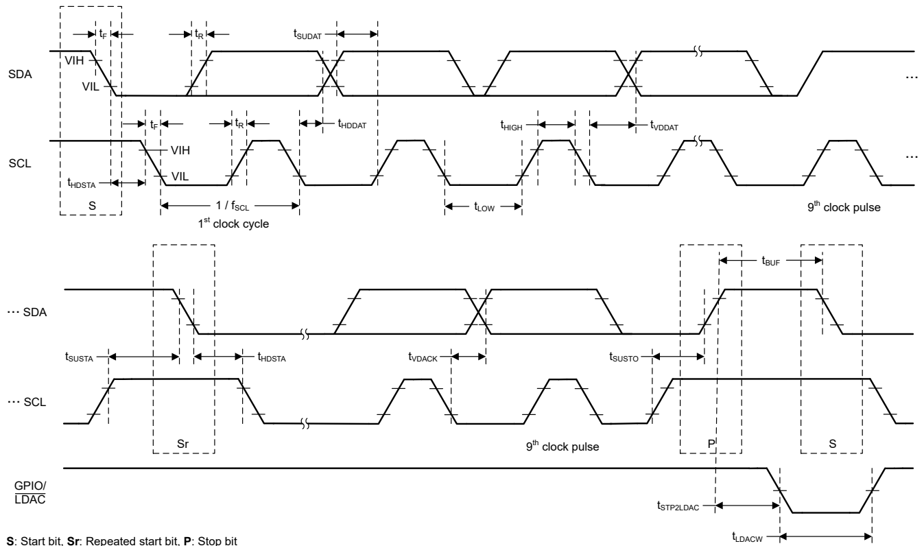
FIG 6-1. I 2 C Timing Diagram
