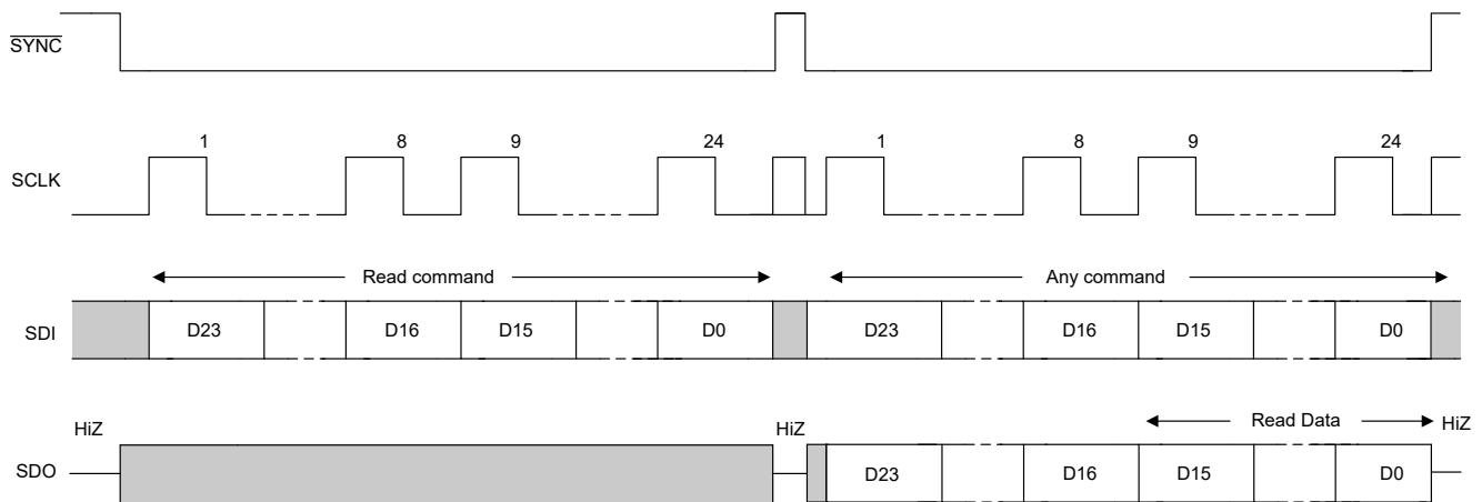
図 7-17. SPI Read Cycle
