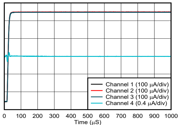
FIG 6-45. Current Output Power-On Glitch
