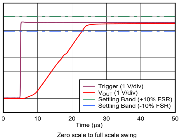
FIG 6-21. Voltage Output Setting Time: Rising Edge
