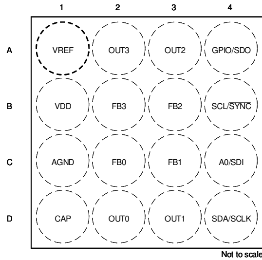
図 5-1. YBH Package, 16-pin DSBGA (Top View)
