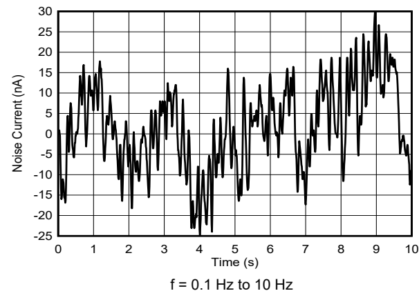
6-47. Current Output Flicker Noise
