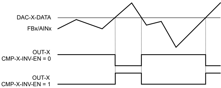
図 7-4. Programmable Comparator Operation
