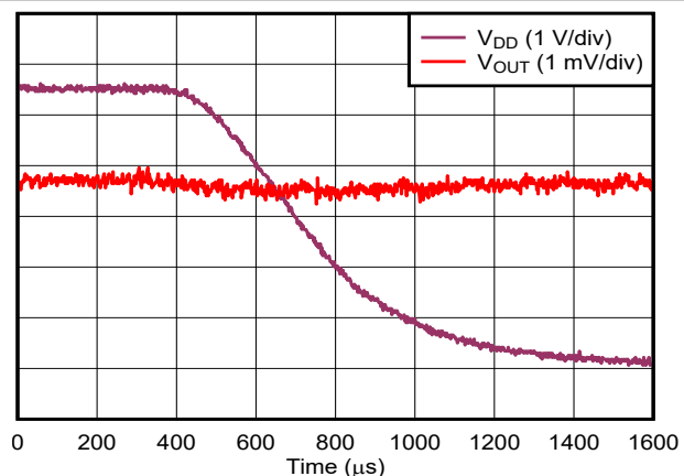
FIG 6-23. Voltage Output Setting Time - Falling Edge
