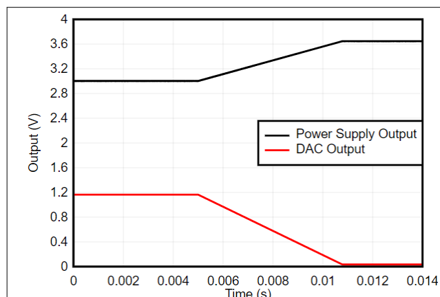
図 8-2. Power-Supply Margin High
