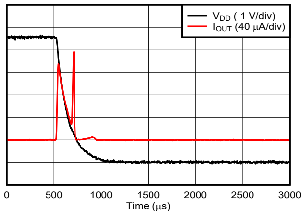
6-43. Current Output Setting Time, Falling Edge
