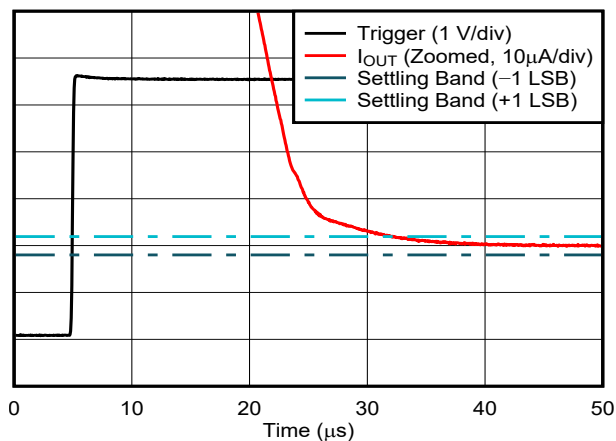
6-43. Current Output Setting Time, Falling Edge
