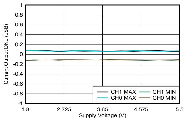
Figure 6-35. Current Output DNL vs Supply Voltage
