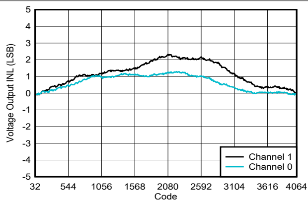
FIG 6-5. Voltage Output INL vs Digital Input Code
