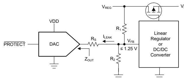
7-9. High-Impedance (Hi-Z) Output and PROTECT Input
