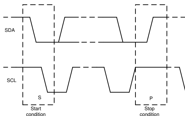
Figure 7-19. Start and Stop Conditions
