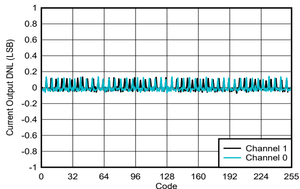
FIG 6-37. Current Output DNL vs Digital Input Code
