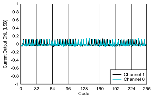
FIG 6-36. Current Output DNL vs Digital Input Code
