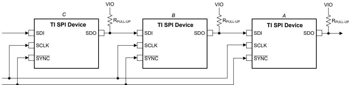
図 7-16. SPI Daisy-Chain Connection
