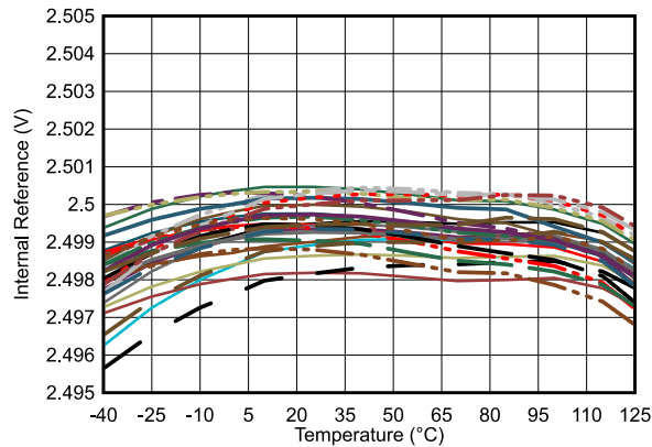
FIG 7-43. Internal Reference Voltage vs Temperature
