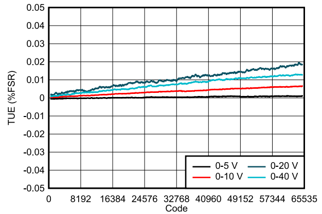
FIG 7-8. DAC81402 TUE vs Digital Input Code (Unipolar Outputs)
