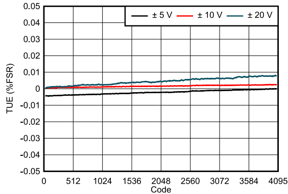
Figure 7-13. DAC61402 TUE vs Digital Input Code (Bipolar Outputs)
