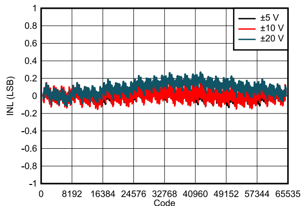
FIG 7-3. DAC81402 INL vs Digital Input Code (Bipolar Outputs)
