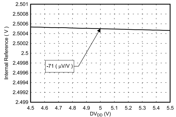
FIG 7-44. Internal Reference Voltage vs Supply Voltage
