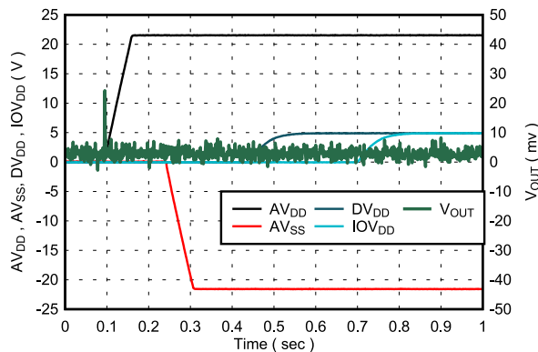
7-38. Power-Up Response
