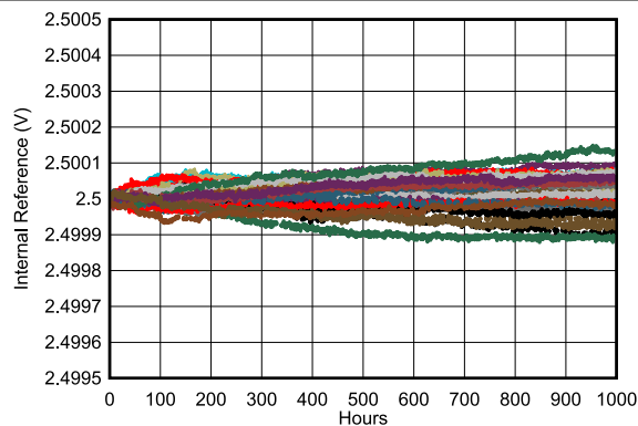
FIG 7-45. Internal Reference Voltage vs Time
