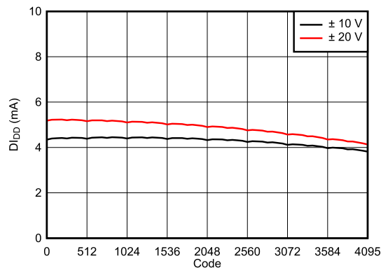
7-26. Supply Current ( DI_{DD} ) vs Digital Input Code
