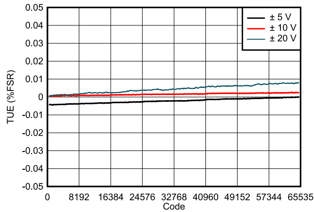
FIG 7-7. DAC81402 TUE vs Digital Input Code (Bipolar Outputs)
