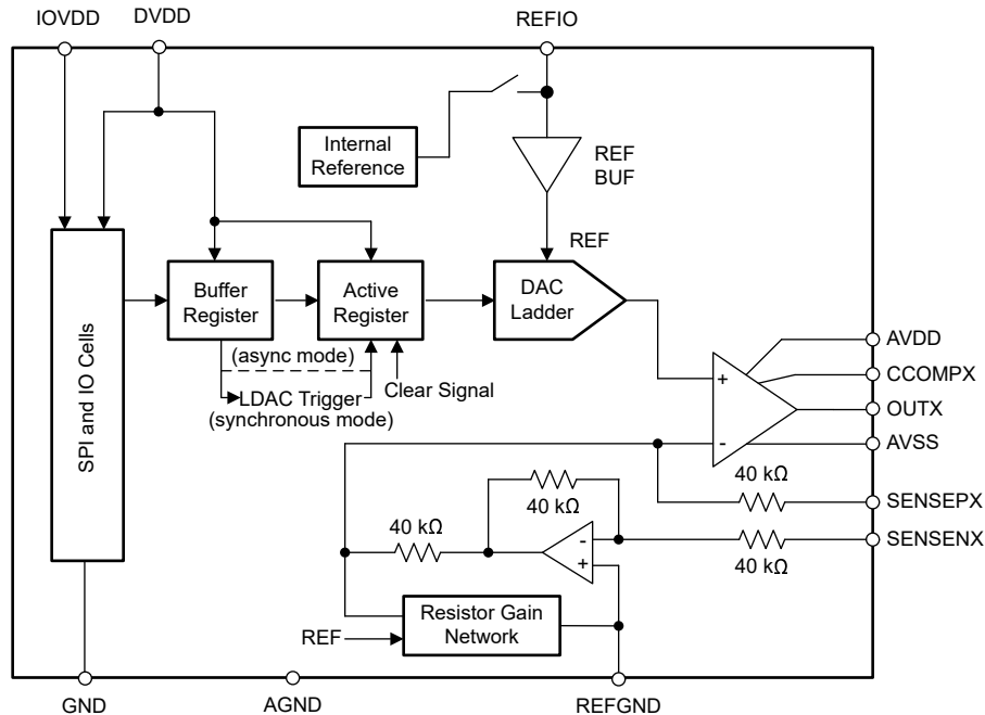
8-1. Device Architecture
