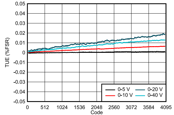
Figure 7-14. DAC61402 TUE vs Digital Input Code (Unipolar Outputs)
