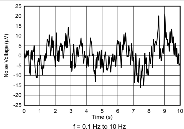
FIG 6-29. Voltage Output Flicker Noise
