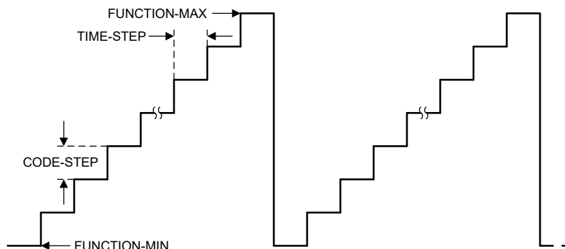
Figure 7-5. Sawtooth Waveform
