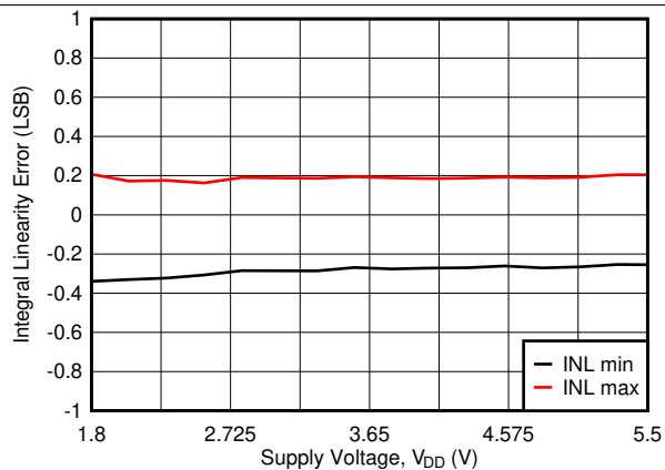
FIG 22. Integral Linearity Error vs Supply Voltage
