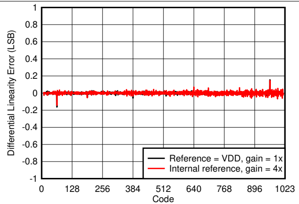
FIG 13. Differential Linearity Error vs Digital Input Code
