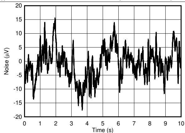
FIG 46. DAC Output Noise: 0.1 Hz to 10 Hz
