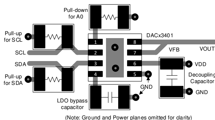
Figure 75. Layout Example
