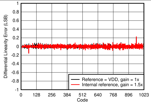
FIG 3. Differential Linearity Error vs Digital Input Code
