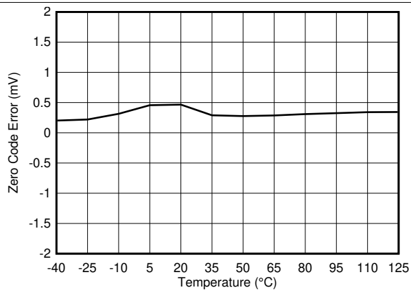
FIG 18. Zero Code Error vs Temperature
