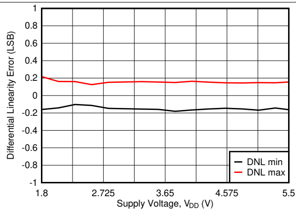
FIG 23. Differential Linearity Error vs Supply Voltage
