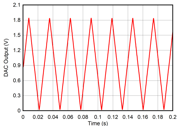
Figure 65. Triangular Waveform
