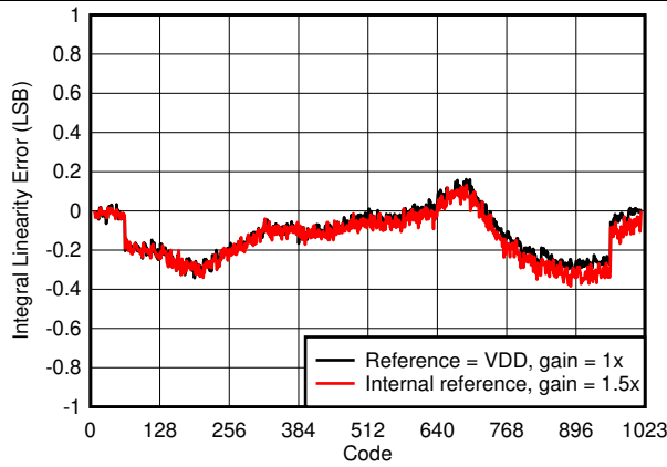
FIG 2. Integral Linearity Error vs Digital Input Code
