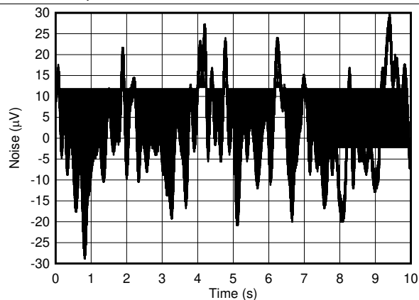
FIG 47. DAC Output Noise: 0.1 Hz to 10 Hz
