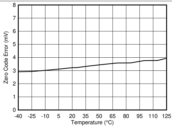
FIG 8. Zero Code Error vs Temperature
