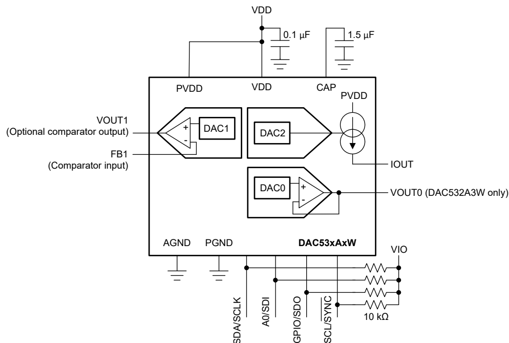
Figure 6-2. Comparator Interface
