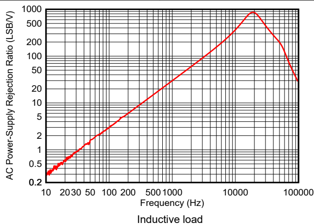
Figure 5-49. Current Output AC PSRR vs Frequency
