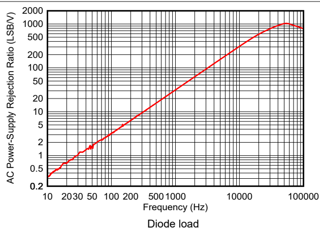
Figure 5-48. Current Output AC PSRR vs Frequency
