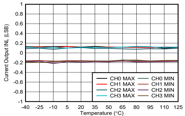
FIG 6-32. Current Output INL vs Temperature
