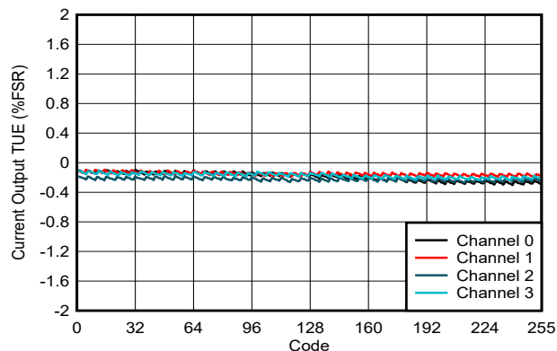
6-37. Current Output TUE vs Digital Input Code
