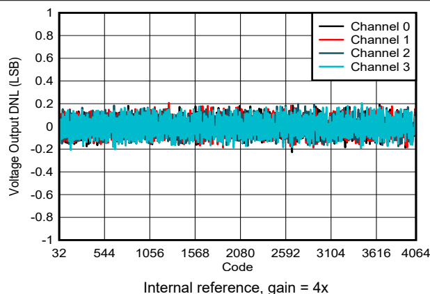
FIG 6-8. Voltage Output DNL vs Digital Input Code
