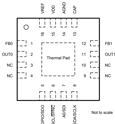
図 5-1. RTE (16-pin WQFN) Package, Top View
