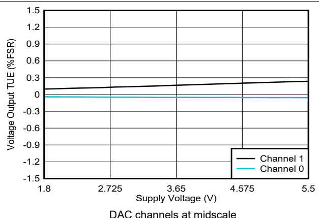
FIG 6-15. Voltage Output TUE vs Supply Voltage
