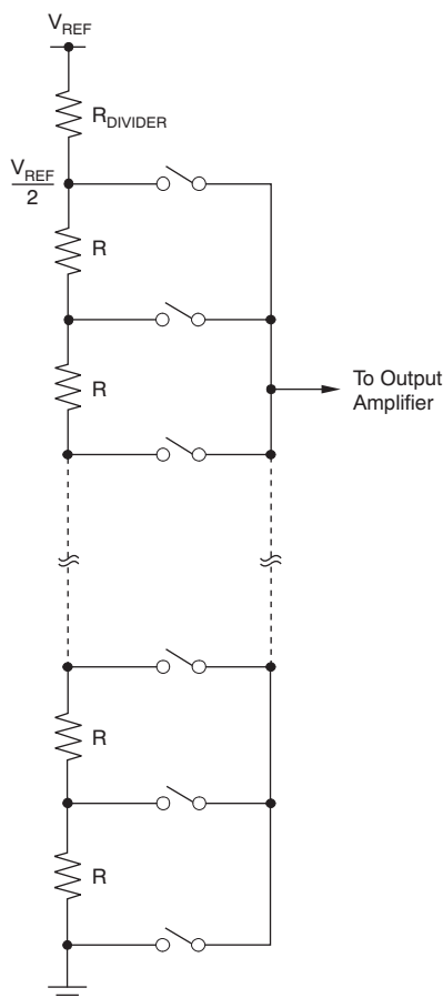
Figure 87. Resistor String
