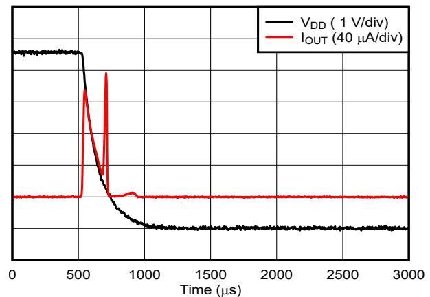
FIG 6-50. Current Output Setting Time, Falling Edge
