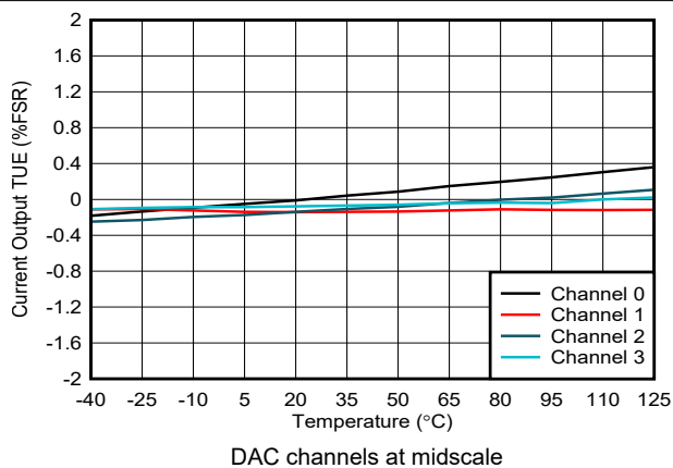
Figure 6-44. Current Output TUE vs Temperature
