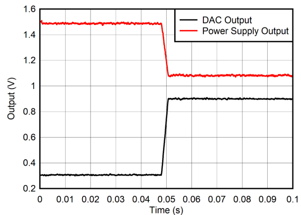
9-6. Power Supply Margin Low
