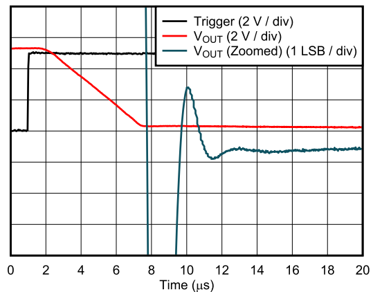
FIG 7-37. Glitch Impulse, Falling Edge, 1-LSB Step
