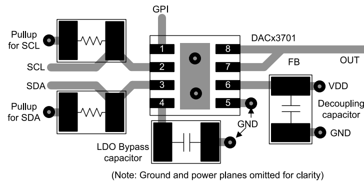
Figure 11-1. Layout Example
