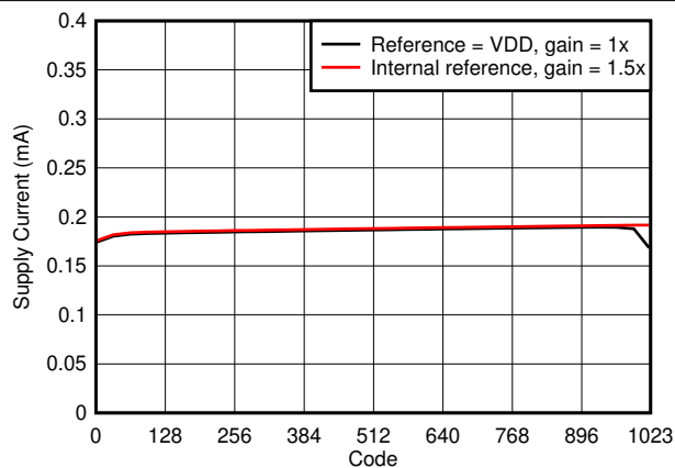
7-28. Supply Current vs Digital Input Code
