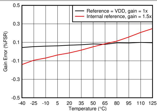
FIG 7-9. Gain Error vs Temperature
