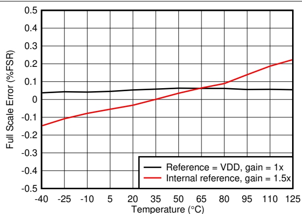
FIG 7-10. Full-Scale Error vs Temperature
