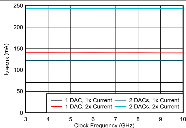
FIG 6-48. VEEM18 Current vs Clock Frequency and Output Current
