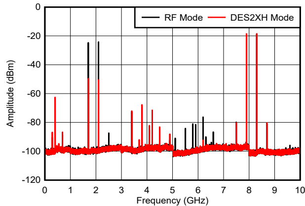
✎ 6-55. Dual Tone, f_{\text{OUT}} = 8097\text{ MHz} , 0 dBFS
