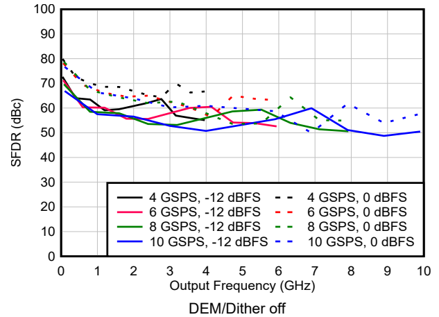
Figure 6-112. SFDR vs Frequency and Sample Rate in DES2X Modes
