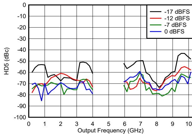
FIG 6-185. HD5 vs Frequency and Digital Amplitude in DES2X Modes
