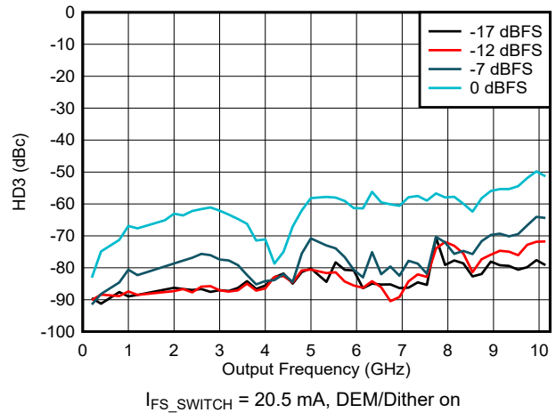
図 6-162. HD3 vs Frequency and Digital Amplitude in NRZ/RF Modes
