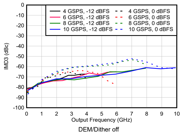
図 6-132. IMD3 vs Frequency and Sample Rate in DES2X Modes
