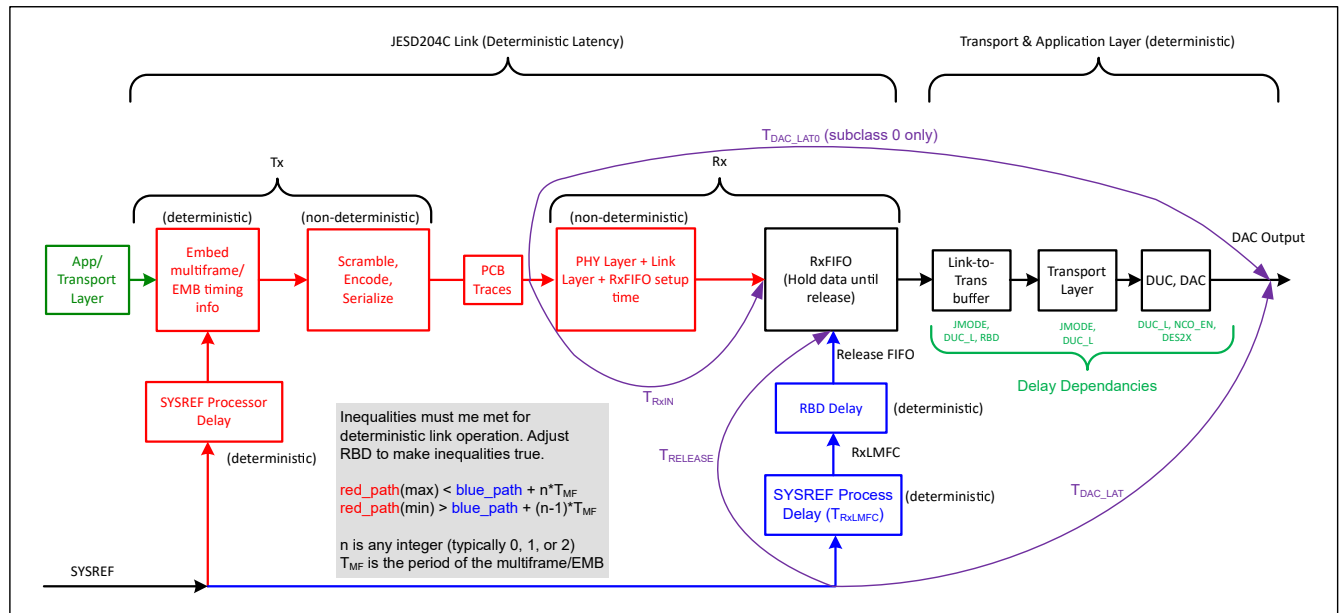
図 7-57. Definition of Device Latencies
