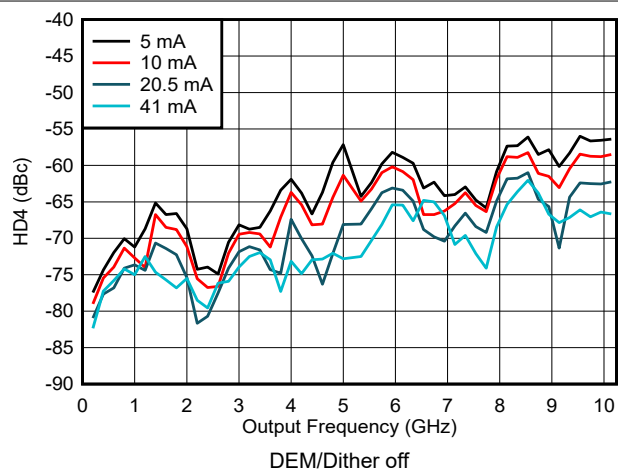
FIG 6-173. HD4 vs Frequency and Output Current in NRZ/RF Modes
