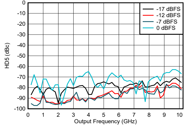
FIG 6-184. HD5 vs Frequency and Digital Amplitude in NRZ/RF Modes
