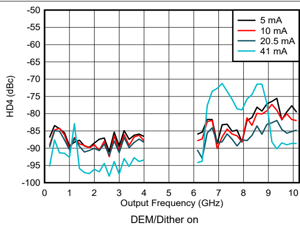
FIG 6-176. HD4 vs Frequency and Output Current in DES2X Modes
