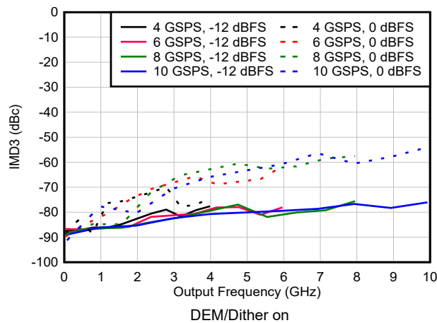
図 6-129. IMD3 vs Frequency and Sample Rate in NRZ/RF Modes
