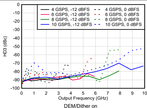
FIG 6-171. HD3 vs Frequency and Sample Rate in DES2X Modes
