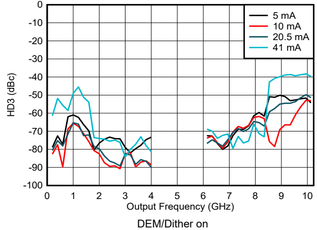
図 6-160. HD3 vs Frequency and Output Current in DES2X Modes
