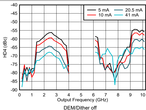
FIG 6-175. HD4 vs Frequency and Output Current in DES2X Modes
