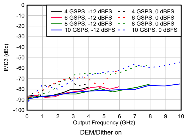
図 6-131. IMD3 vs Frequency and Sample Rate in DES2X Modes
