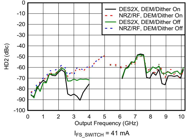
Figure 6-94. HD2 vs Frequency and Mode
