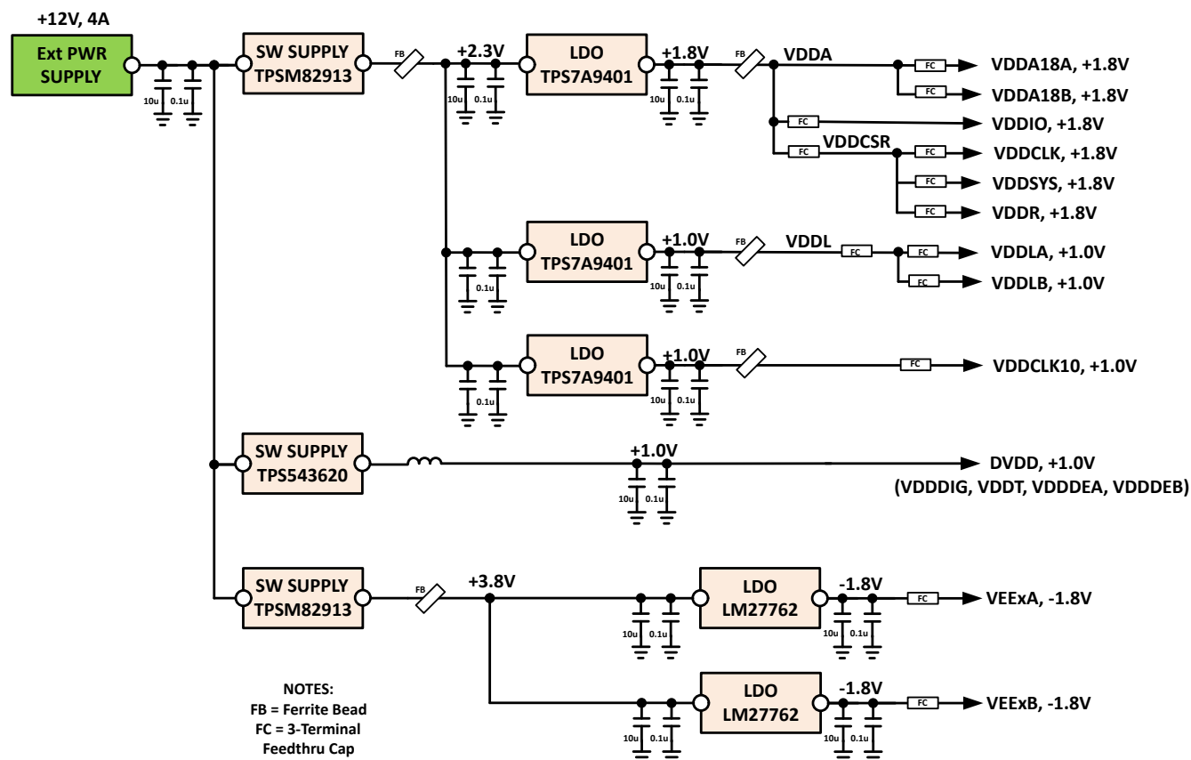
8-23. Recommended Power Supply Block Diagram
