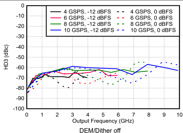
FIG 6-172. HD3 vs Frequency and Sample Rate in DES2X Modes
