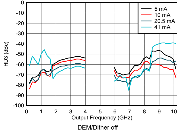
図 6-159. HD3 vs Frequency and Output Current in DES2X Modes
