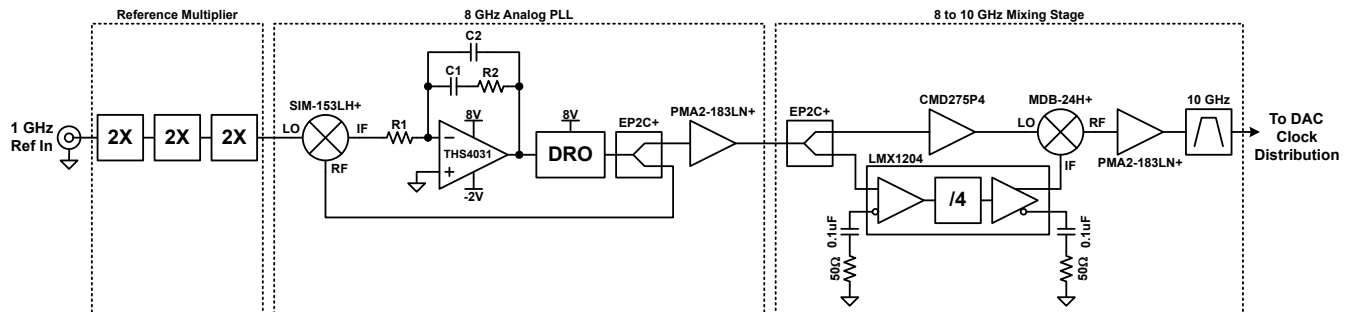
Figure 8-12. 10 GHz Clock Synthesizer
