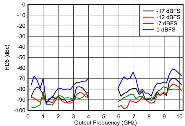
FIG 6-186. HD5 vs Frequency and Digital Amplitude in DES2X Modes
