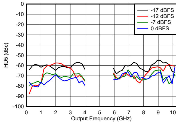
FIG 6-183. HD5 vs Frequency and Digital Amplitude in NRZ/RF Modes
