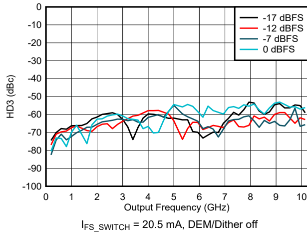
図 6-161. HD3 vs Frequency and Digital Amplitude in NRZ/RF Modes
