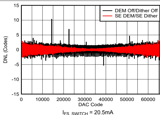
図 6-11. DNL vs DAC Code: 20.5mA
