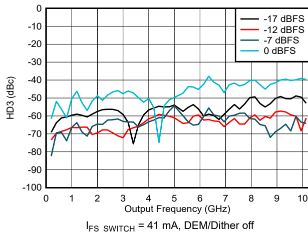
図 6-163. HD3 vs Frequency and Digital Amplitude in NRZ/RF Modes
