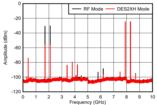
✎ 6-56. Dual Tone, f_{\text{OUT}} = 8097\text{ MHz} , -6 dBFS
