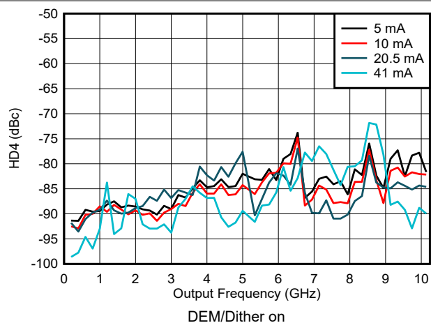
FIG 6-174. HD4 vs Frequency and Output Current in NRZ/RF Modes
