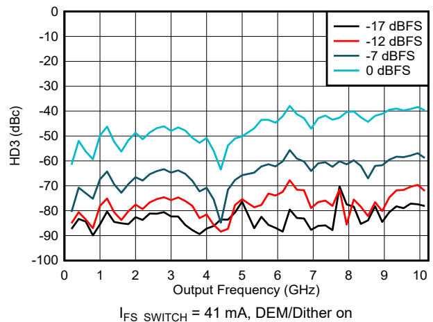
図 6-164. HD3 vs Frequency and Digital Amplitude in NRZ/RF Modes
