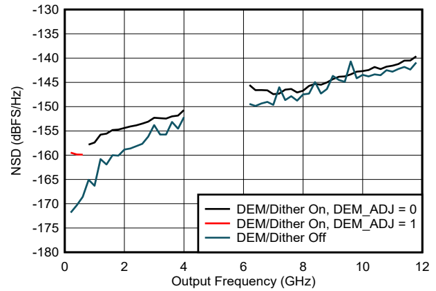
FIG 6-59. NSD vs Output Frequency and DEM/Dither Mode
