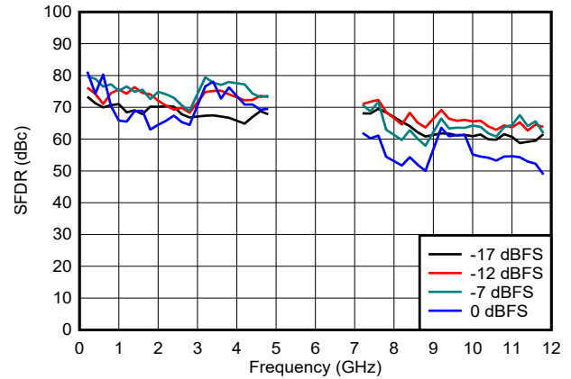
図 6-99. SFDR vs Frequency and Digital Amplitude in DES2X Modes
