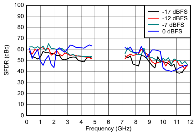
図 6-98. SFDR vs Frequency and Digital Amplitude in DES2X Modes
