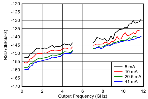
FIG 6-61. NSD vs Output Frequency and Output Current
