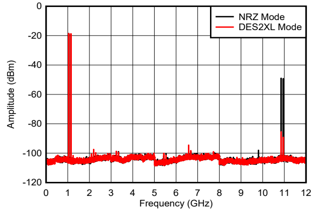
图 6-44. Dual Tone, f_{\text{OUT}} = 1097\text{ MHz} , -6 dBFS
