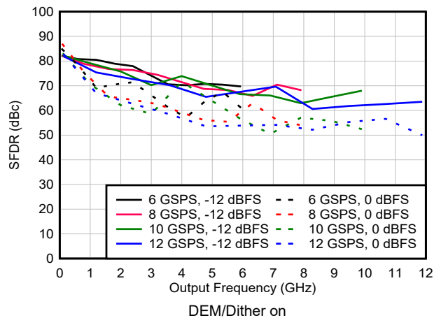
図 6-102. SFDR vs Frequency and Sample Rate in NRZ/RF Modes
