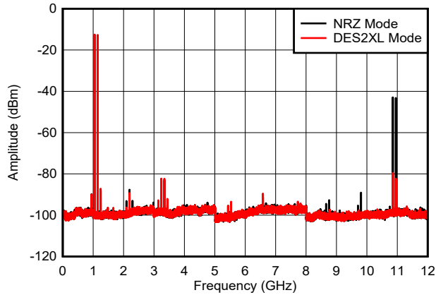
图 6-43. Dual Tone, f_{\text{OUT}} = 1097\text{ MHz} , 0 dBFS
