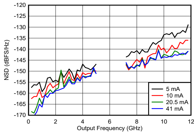
FIG 6-60. NSD vs Output Frequency and Output Current
