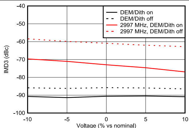
図 6-153. IMD3 vs Voltage in DES2XL Mode
