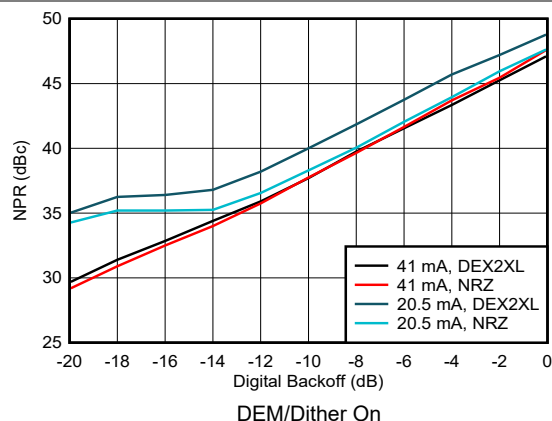
図 6-211. Noise Power Ratio vs Digital Backoff: 1 st Nyquist Zone
