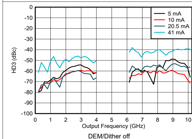
図 6-172. HD3 vs Frequency and Output Current in NRZ/RF Modes
