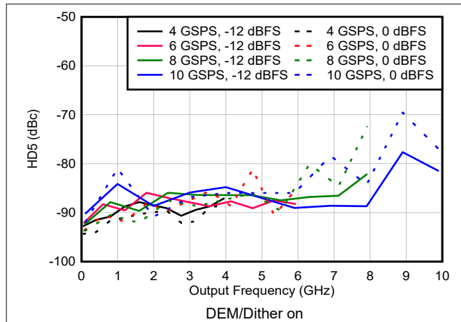
図 6-204. HD5 vs Frequency and Sample Rate in NRZ/RF Modes
