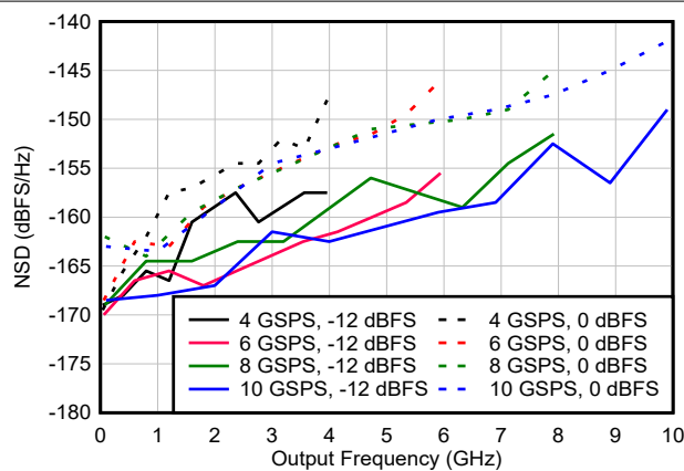
Figure 6-77. NSD vs Output Frequency and Sample Rate
