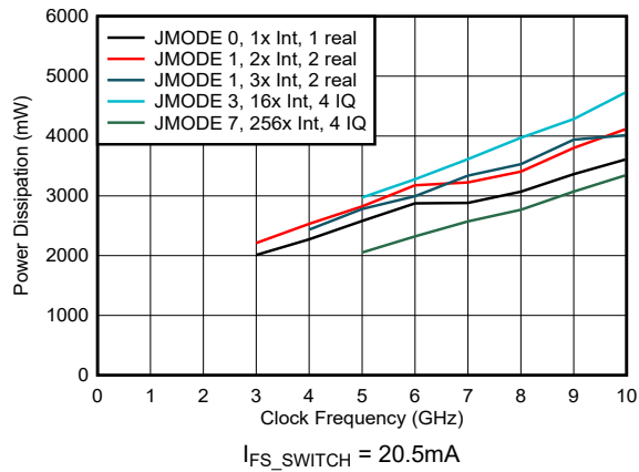
6-89. Power Dissipation vs Clock Frequency and Digital Mode
