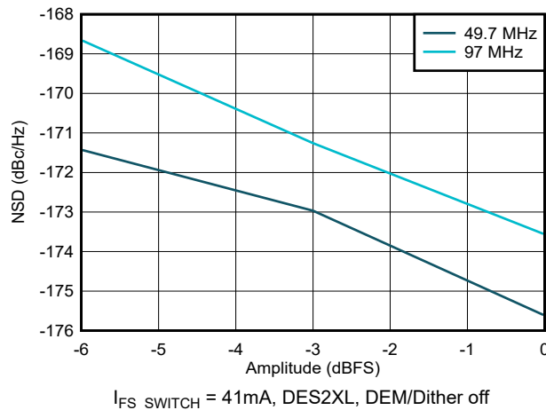
図 6-60. NSD vs Digital Amplitude at Low Frequency
