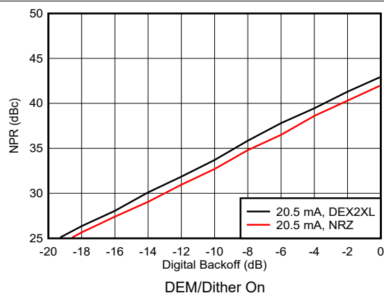
図 6-213. Noise Power Ratio vs Digital Backoff: 2 nd Nyquist Zone
