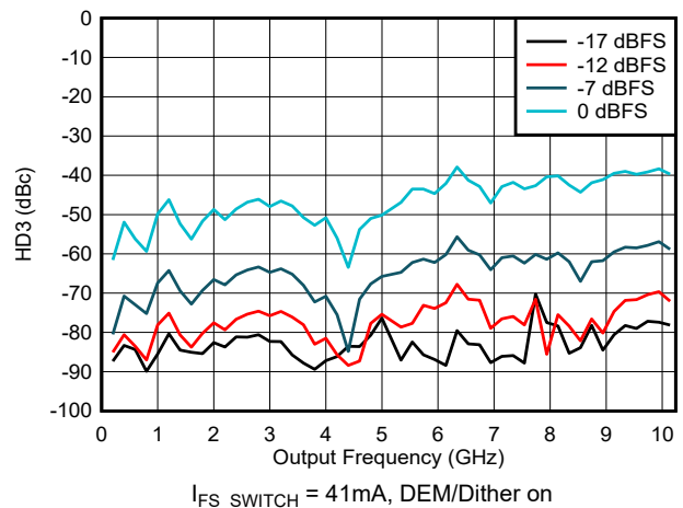
図 6-179. HD3 vs Frequency and Digital Amplitude in NRZ/RF Modes
