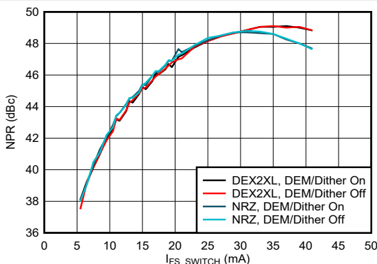
図 6-214. Noise Power Ratio vs Output Current: 1 st Nyquist Zone
