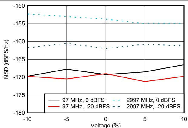
図 6-87. NSD vs Supply Voltage
