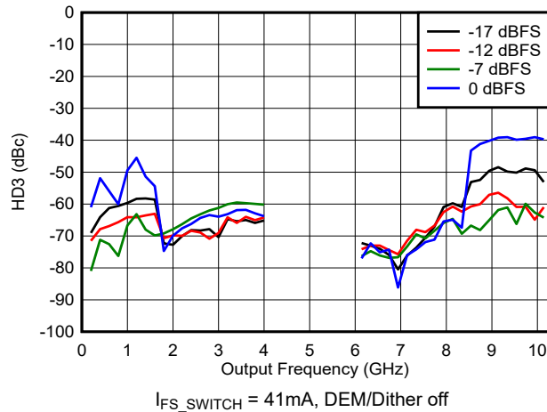
FIG 6-182. HD3 vs Frequency and Digital Amplitude in DES2X Modes
