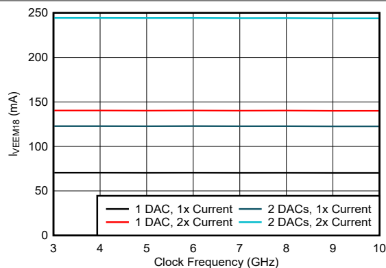
Figure 6-96. VEEM18 Current vs Clock Frequency and DAC Mode
