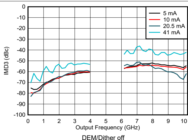
図 6-130. IMD3 vs Frequency and Output Current in DES2X Modes
