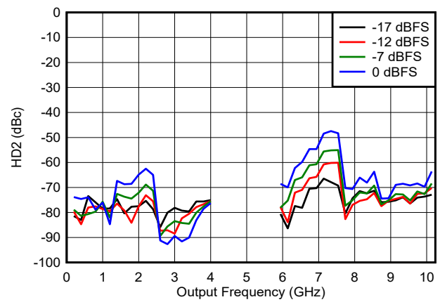
Figure 6-165. HD2 vs Frequency and Digital Amplitude in DES2X Modes
