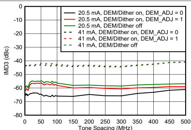
6-141. IMD3 vs Tone Spacing in DES2XL Mode
