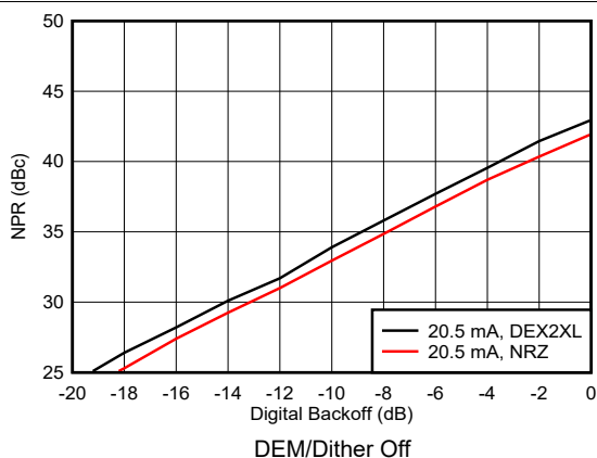
図 6-212. Noise Power Ratio vs Digital Backoff: 2 nd Nyquist Zone
