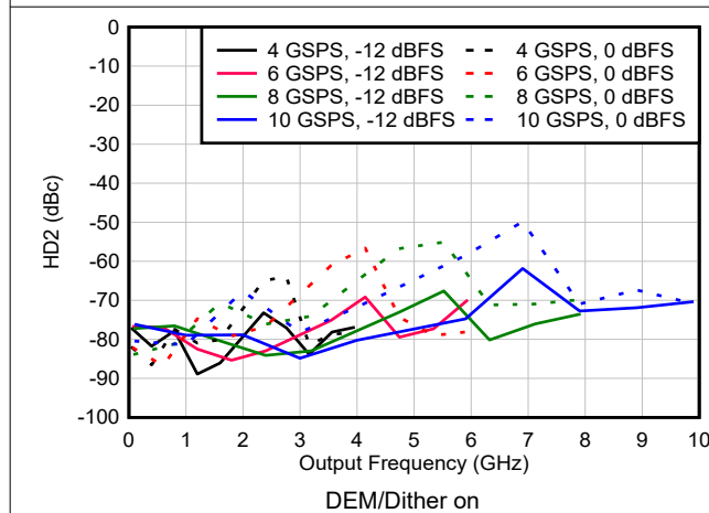
図 6-170. HD2 vs Frequency and Sample Rate in DES2X Modes
