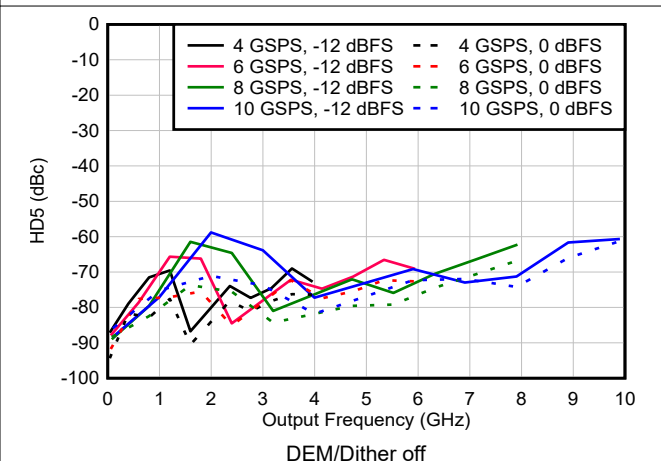
図 6-207. HD5 vs Frequency and Sample Rate in DES2X Modes
