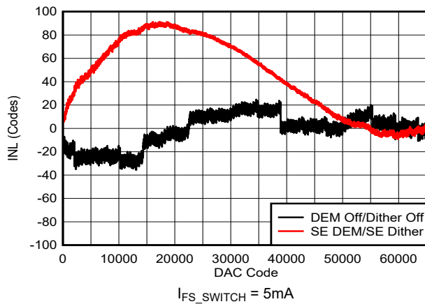
図 6-14. INL vs DAC Code: 5mA
