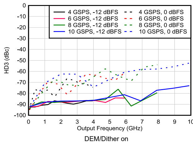
FIG 6-184. HD3 vs Frequency and Sample Rate in NRZ/RF Modes
