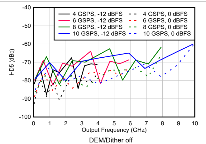
図 6-205. HD5 vs Frequency and Sample Rate in NRZ/RF Modes
