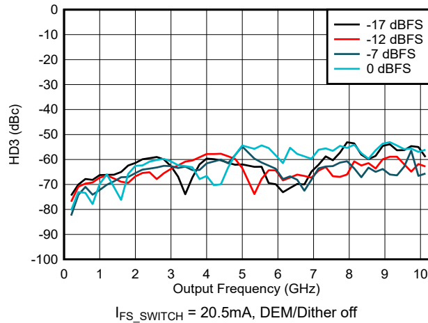
図 6-176. HD3 vs Frequency and Digital Amplitude in NRZ/RF Modes
