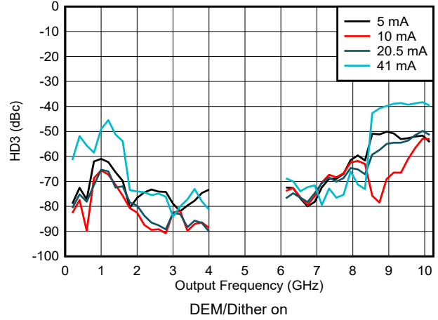
図 6-175. HD3 vs Frequency and Output Current in DES2X Modes
