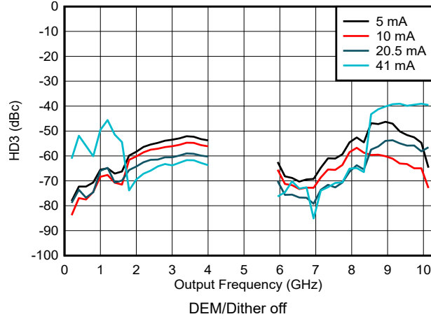
図 6-174. HD3 vs Frequency and Output Current in DES2X Modes
