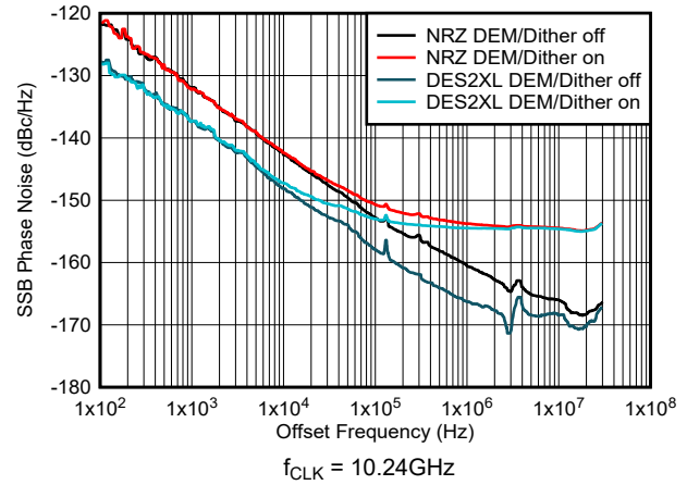
图 6-217. Phase Noise vs Offset Frequency at 1GHz
