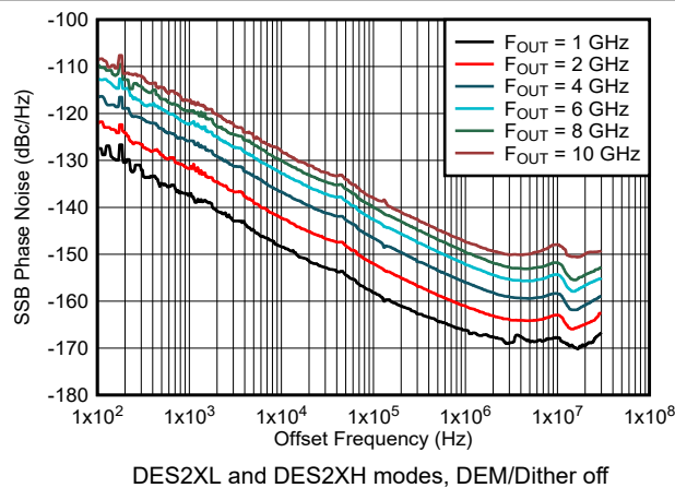
图 6-218. Phase Noise vs Offset Frequency and Output Frequency
