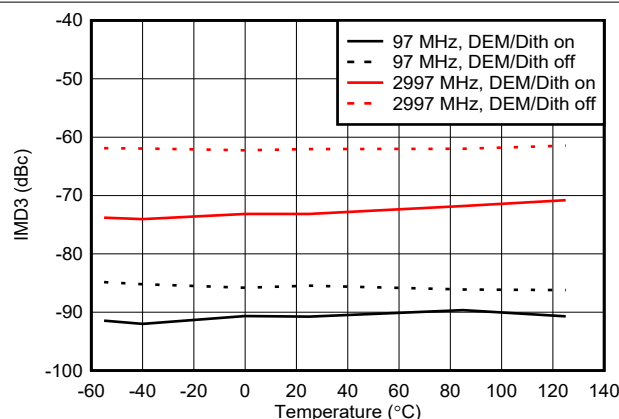
図 6-148. IMD3 vs Temperature in NRZ Mode
