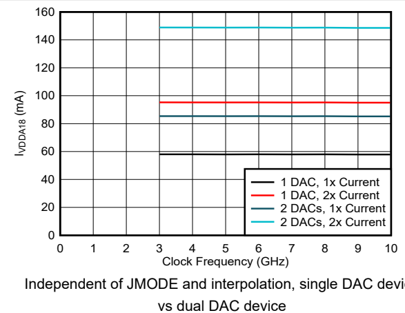
6-94. VDDA18 Current vs Clock Frequency and DAC Mode
