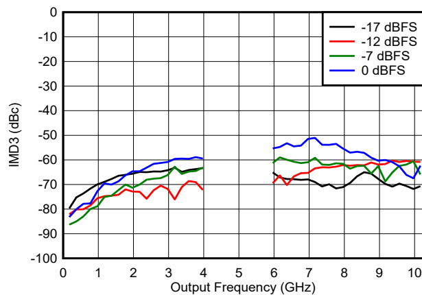
FIG 6-134. IMD3 vs Frequency and Digital Amplitude in NRZ/RF Modes
