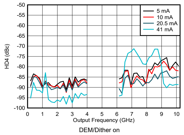
図 6-191. HD4 vs Frequency and Output Current in DES2X Modes
