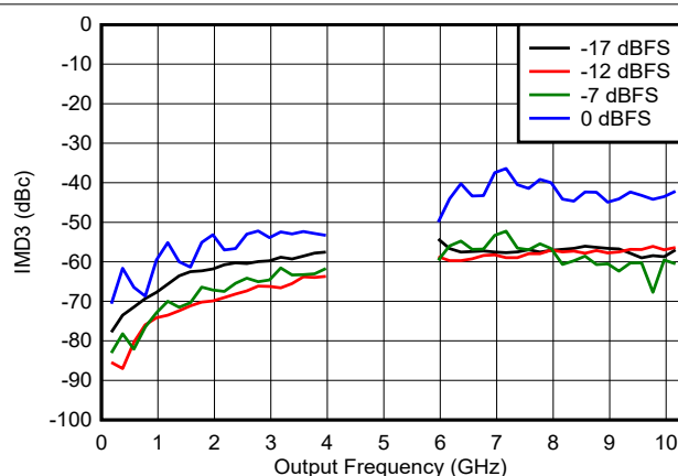
6-138. IMD3 vs Frequency and Digital Amplitude in DES2X Modes
