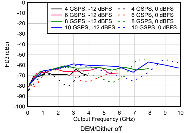
図 6-187. HD3 vs Frequency and Sample Rate in DES2X Modes
