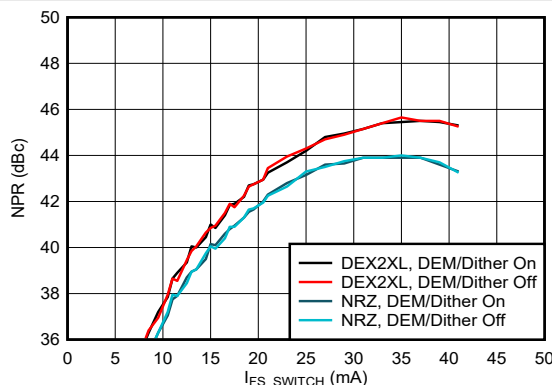
図 6-215. Noise Power Ratio vs Output Current: 2 nd Nyquist Zone
