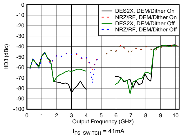
Figure 6-111. HD3 vs Frequency and Mode
