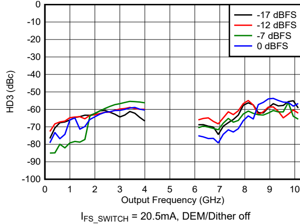
FIG 6-180. HD3 vs Frequency and Digital Amplitude in DES2X Modes
