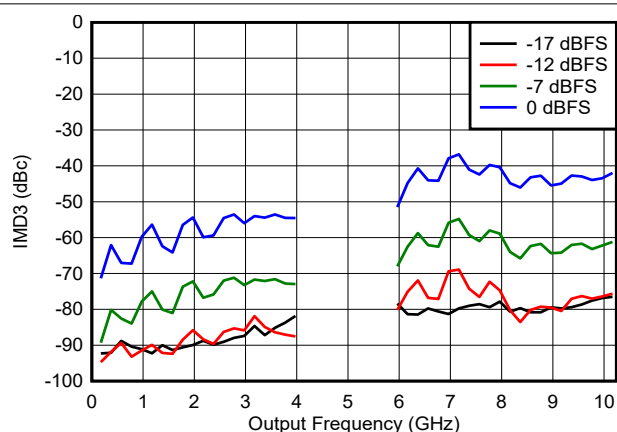
6-139. IMD3 vs Frequency and Digital Amplitude in DES2X Modes
