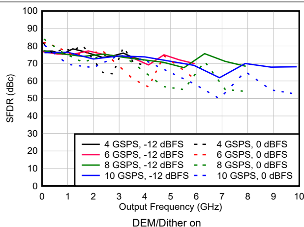
図 6-126. SFDR vs Frequency and Sample Rate in DES2X Modes
