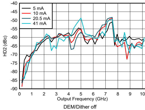
6-156. HD2 vs Frequency and Output Current in NRZ/RF Modes
