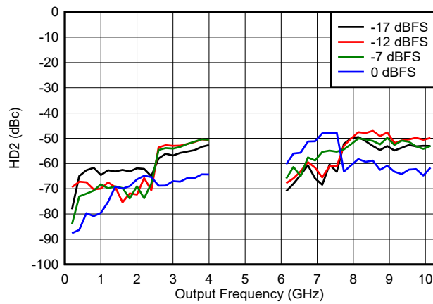
Figure 6-162. HD2 vs Frequency and Digital Amplitude in NRZ/RF Modes
