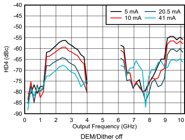
図 6-190. HD4 vs Frequency and Output Current in DES2X Modes
