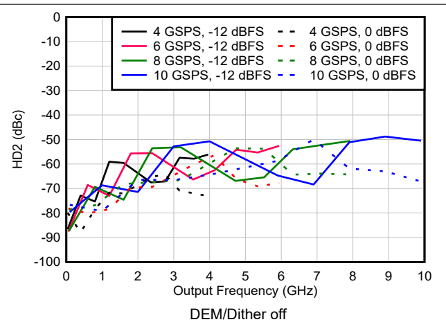
図 6-171. HD2 vs Frequency and Sample Rate in DES2X Modes
