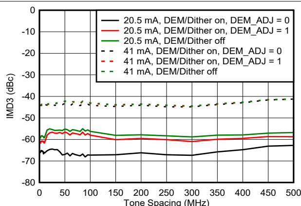
6-140. IMD3 vs Tone Spacing in NRZ Mode
