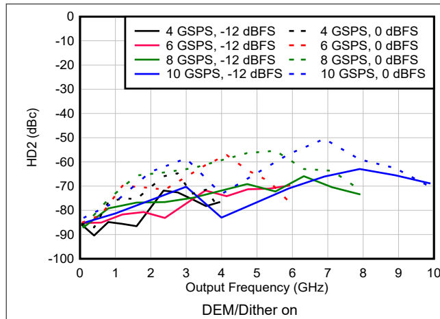
図 6-168. HD2 vs Frequency and Sample Rate in NRZ/RF Modes
