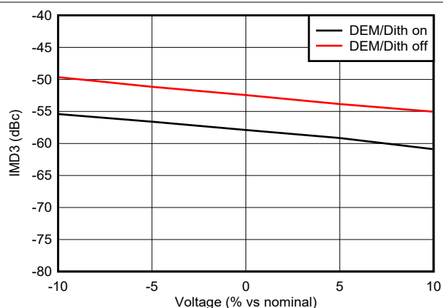
図 6-155. IMD3 vs Voltage in DES2XH Mode at 7247MHz
