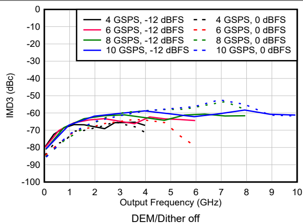
図 6-145. IMD3 vs Frequency and Sample Rate in NRZ/RF Modes
