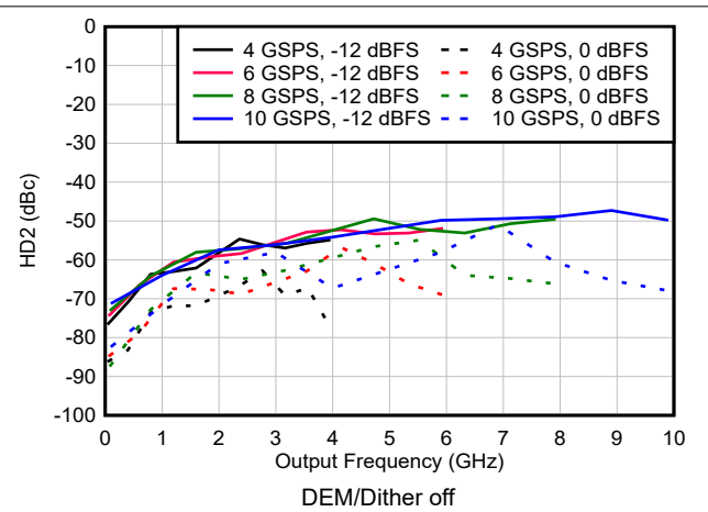
図 6-169. HD2 vs Frequency and Sample Rate in NRZ/RF Modes
