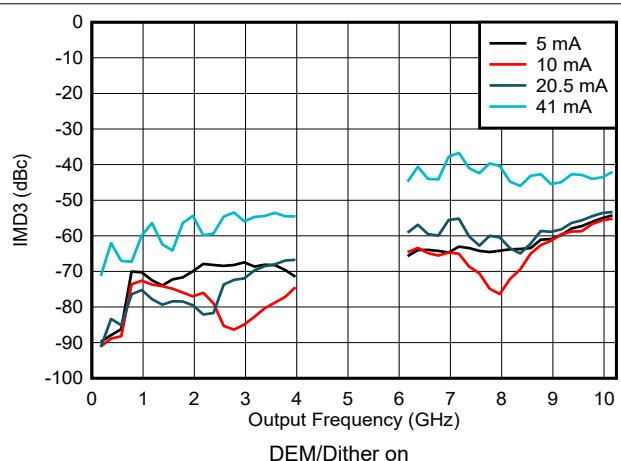
図 6-131. IMD3 vs Frequency and Output Current in DES2X Modes
