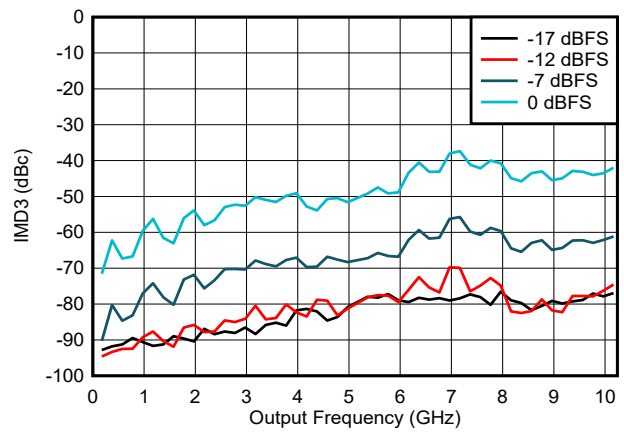
FIG 6-133. IMD3 vs Frequency and Digital Amplitude in NRZ/RF Modes
