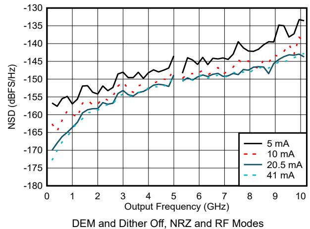
図 6-61. NSD vs Output Frequency and Output Current
