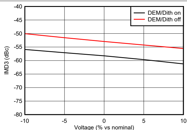
図 6-154. IMD3 vs Voltage in RF Mode at 7247MHz
