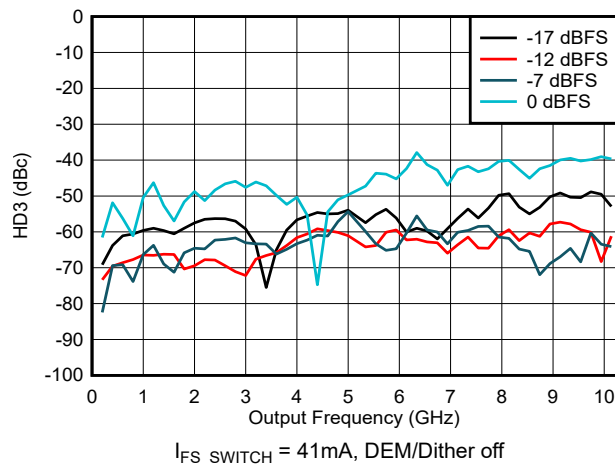
図 6-178. HD3 vs Frequency and Digital Amplitude in NRZ/RF Modes
