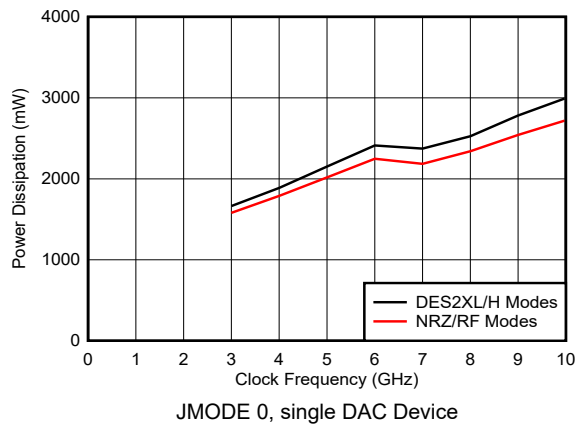
6-91. Power Dissipation vs Clock Frequency and DAC Mode
