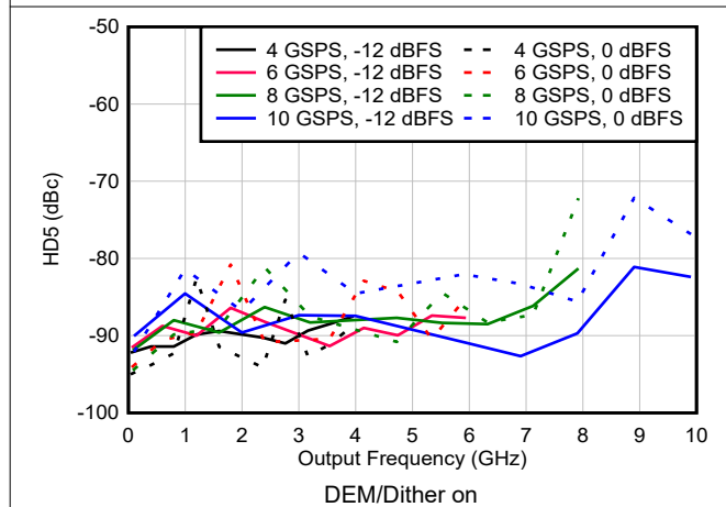
図 6-206. HD5 vs Frequency and Sample Rate in DES2X Modes
