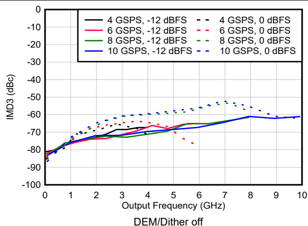
図 6-147. IMD3 vs Frequency and Sample Rate in DES2X Modes
