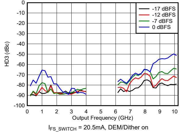
FIG 6-181. HD3 vs Frequency and Digital Amplitude in DES2X Modes
