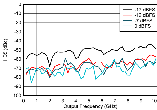
FIG 6-198. HD5 vs Frequency and Digital Amplitude in NRZ/RF Modes
