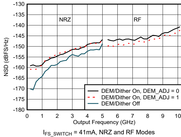
図 6-58. NSD vs Output Frequency and DEM/Dither Mode
