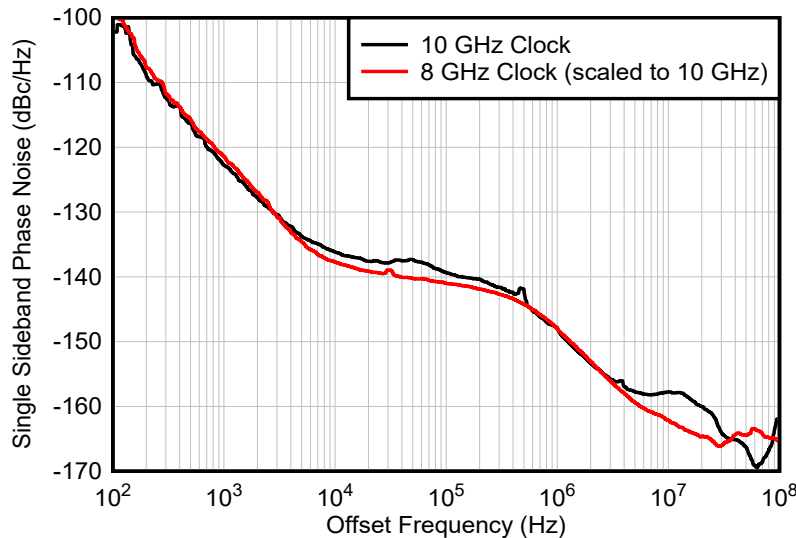
8-12. 8GHz and 10GHz Clock Phase Noise
