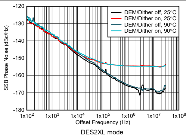
图 6-220. Phase Noise vs Offset Frequency at 1GHz
