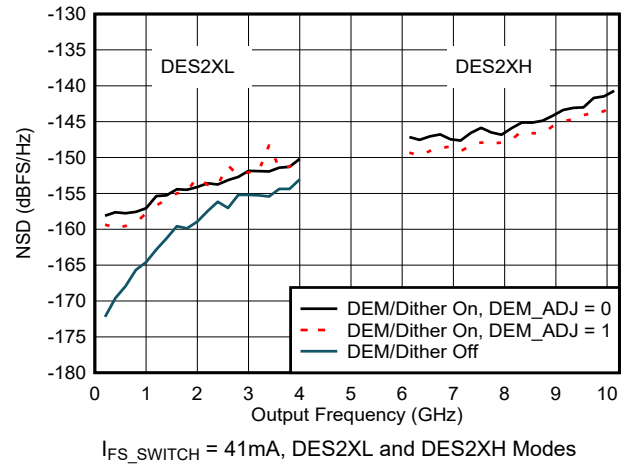
図 6-59. NSD vs Output Frequency and DEM/Dither Mode
