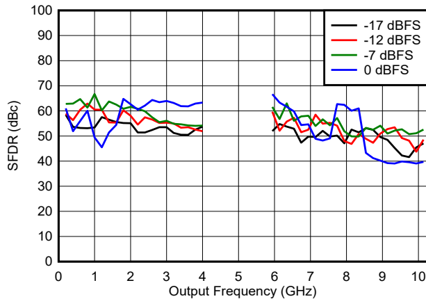
I_{FS\_SWITCH} = 41\text{mA} , DEM/Dither off 6-122. SFDR vs Frequency and Digital Amplitude in DES2X Modes
