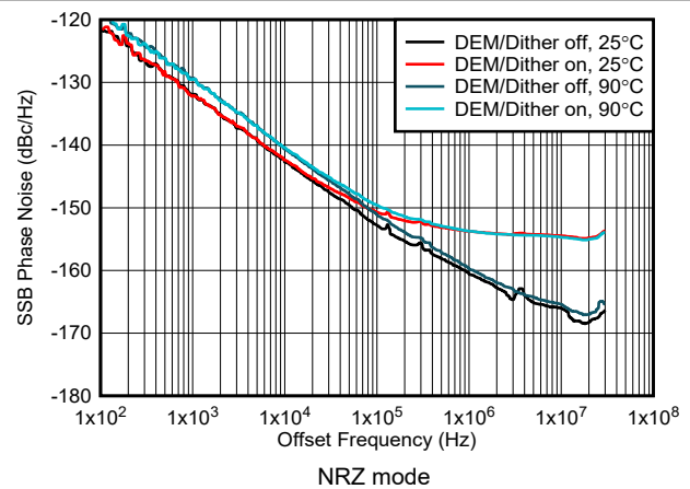
图 6-219. Phase Noise vs Offset Frequency at 1GHz
