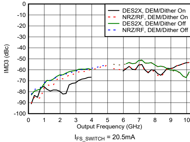
図 6-106. IMD3 vs Frequency and Mode
