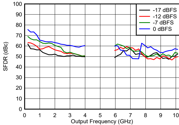
I_{FS\_SWITCH} = 20.5\text{mA} , DEM/Dither off 6-120. SFDR vs Frequency and Digital Amplitude in DES2X Modes
