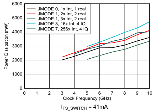
6-90. Power Dissipation vs Clock Frequency and Digital Mode
