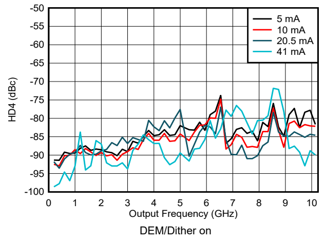
図 6-189. HD4 vs Frequency and Output Current in NRZ/RF Modes
