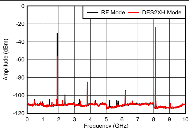
図 6-34. f_{\text{OUT}} = 8097\text{MHz} , 0dBFS
