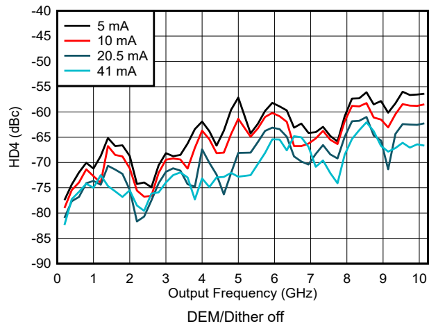
図 6-188. HD4 vs Frequency and Output Current in NRZ/RF Modes
