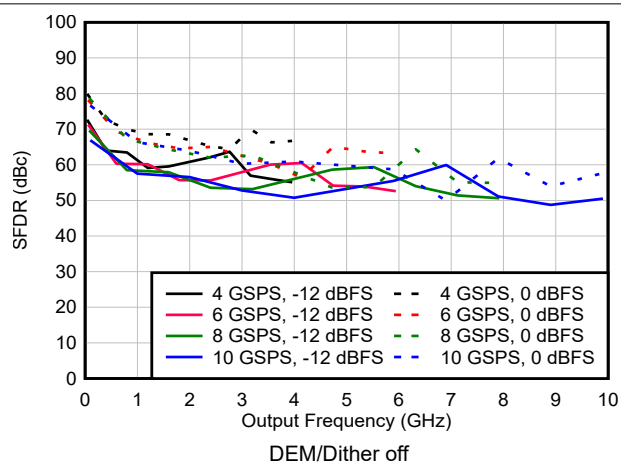
図 6-127. SFDR vs Frequency and Sample Rate in DES2X Modes
