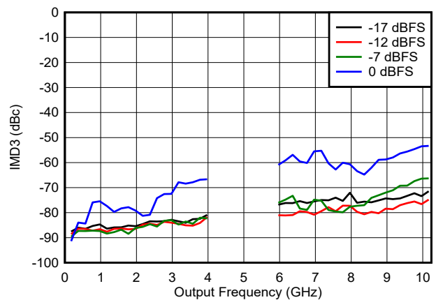
FIG 6-135. IMD3 vs Frequency and Digital Amplitude in NRZ/RF Modes
