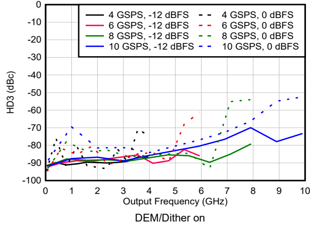
図 6-186. HD3 vs Frequency and Sample Rate in DES2X Modes
