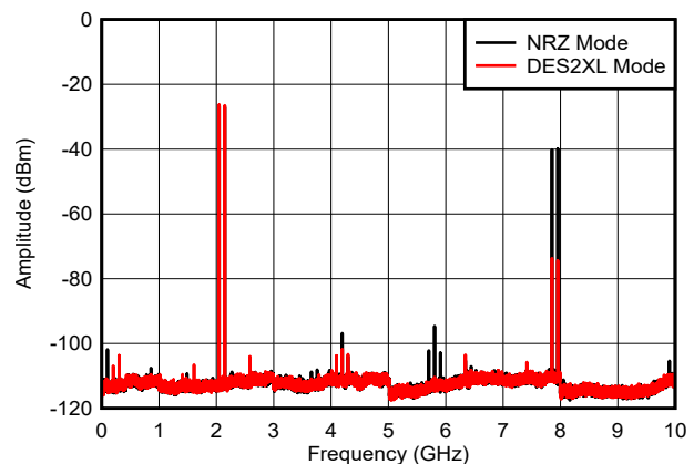
図 6-46. Dual Tone, f_{\text{OUT}} = 2097\text{ MHz} , 0dBFS
