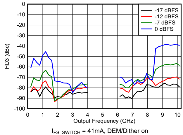
FIG 6-183. HD3 vs Frequency and Digital Amplitude in DES2X Modes
