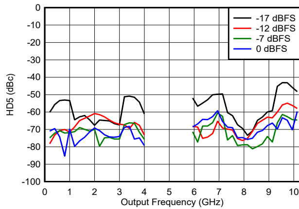
FIG 6-200. HD5 vs Frequency and Digital Amplitude in DES2X Modes
