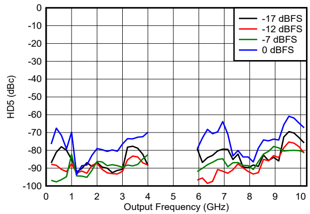
FIG 6-201. HD5 vs Frequency and Digital Amplitude in DES2X Modes
