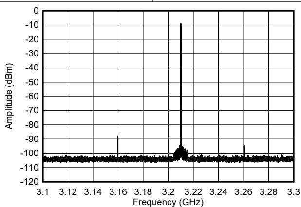
図 8-19. In Band Single Tone Frequency Spectra with f_{OUT} = 3.211\text{GHz}
