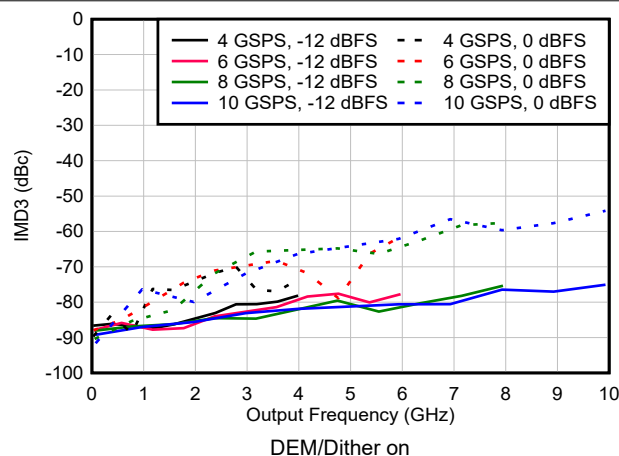
図 6-146. IMD3 vs Frequency and Sample Rate in DES2X Modes
