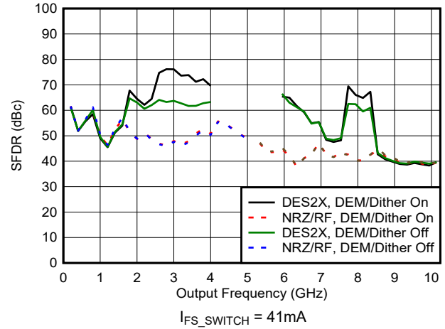
図 6-105. SFDR vs Frequency and Mode
