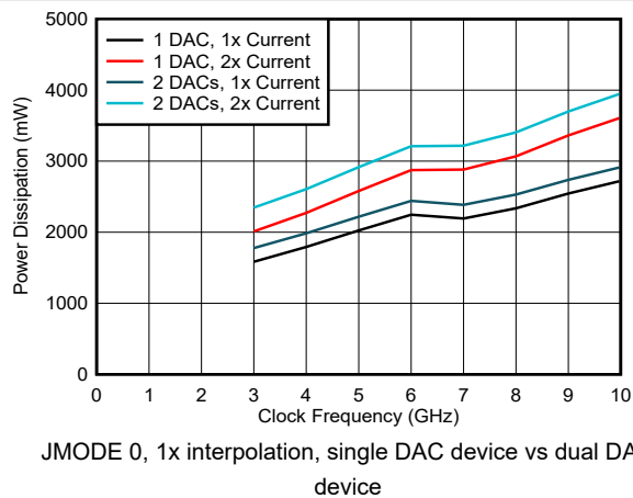
6-93. Power Dissipation vs Clock Frequency and DAC Mode
