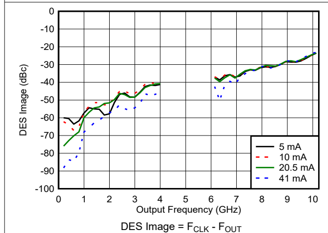
図 6-208. DES Image vs Frequency and Output Current in DES2X Modes
