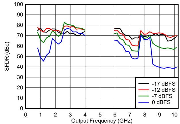
I_{FS\_SWITCH} = 41\text{mA} , DEM/Dither on 6-123. SFDR vs Frequency and Digital Amplitude in DES2X Modes
