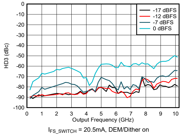
図 6-177. HD3 vs Frequency and Digital Amplitude in NRZ/RF Modes
