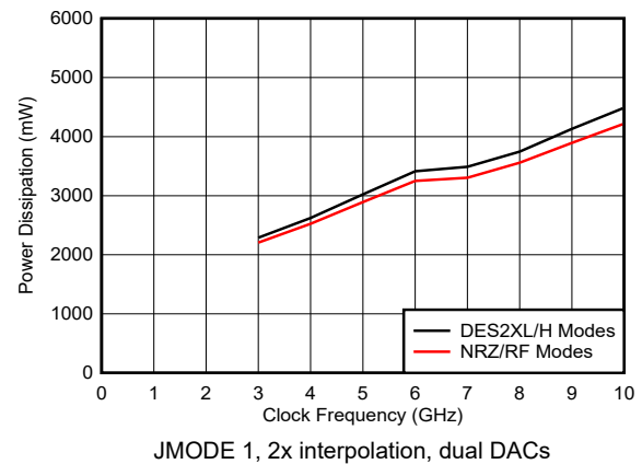
6-92. Power Dissipation vs Clock Frequency and DAC Mode
