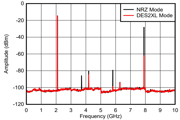
✎ 6-26. f_{\text{OUT}} = 2097\text{ MHz} , -6dBFS
