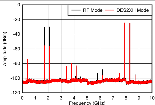
✎ 6-56. Dual Tone, f_{\text{OUT}} = 8097\text{MHz} , -6dBFS
