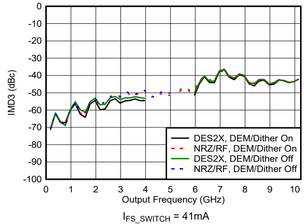
図 6-107. IMD3 vs Frequency and Mode
