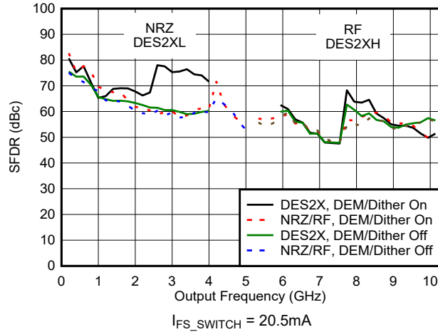
図 6-104. SFDR vs Frequency and Mode
