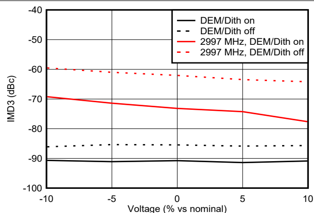
図 6-152. IMD3 vs Voltage in NRZ Mode
