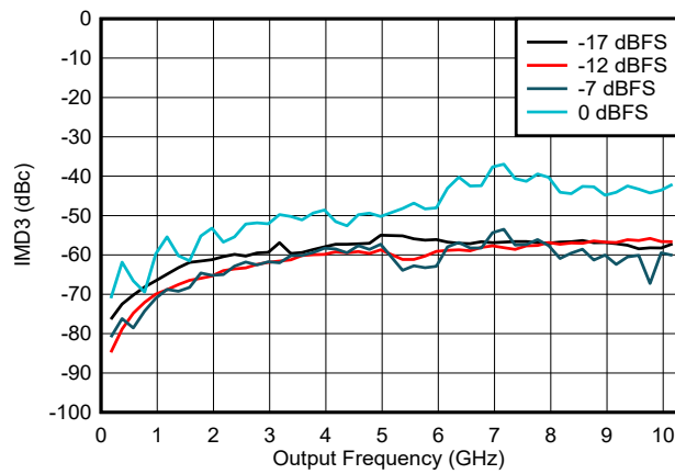
FIG 6-132. IMD3 vs Frequency and Digital Amplitude in NRZ/RF Modes
