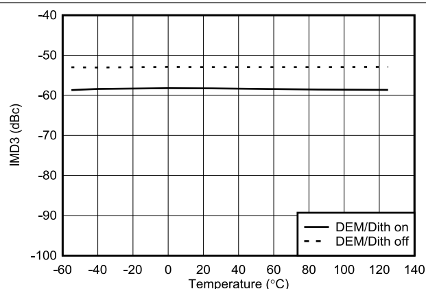
図 6-150. IMD3 vs Temperature in RF Mode at 7247MHz
