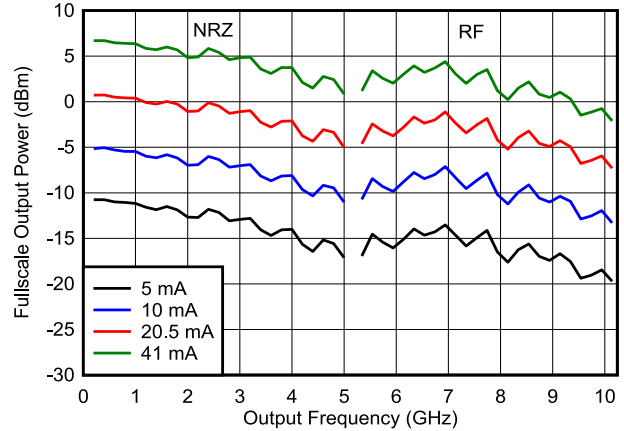
図 6-9. Output Power vs Frequency (NRZ/RF modes)
