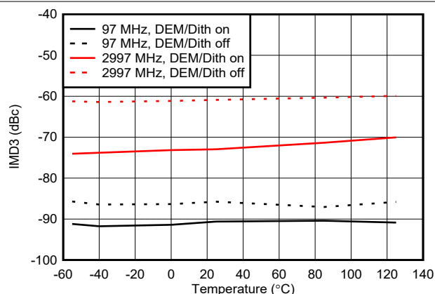
図 6-149. IMD3 vs Temperature in DES2XL Mode
