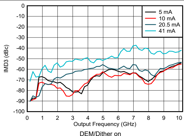
図 6-129. IMD3 vs Frequency and Output Current in NRZ/RF Modes
