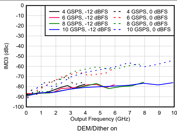
図 6-144. IMD3 vs Frequency and Sample Rate in NRZ/RF Modes
