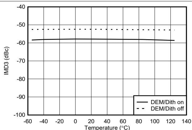
図 6-151. IMD3 vs Temperature in DES2XH Mode at 7247MHz
