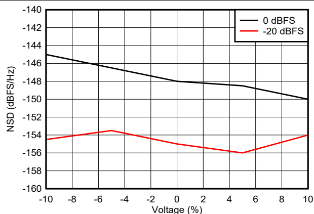
図 6-86. NSD vs Supply Voltage
