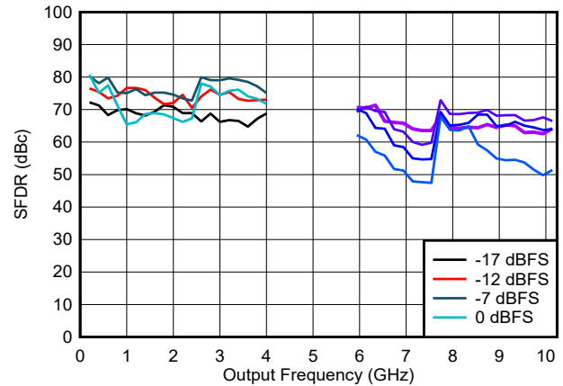
I_{FS\_SWITCH} = 20.5\text{mA} , DEM/Dither on 6-121. SFDR vs Frequency and Digital Amplitude in DES2X Modes
