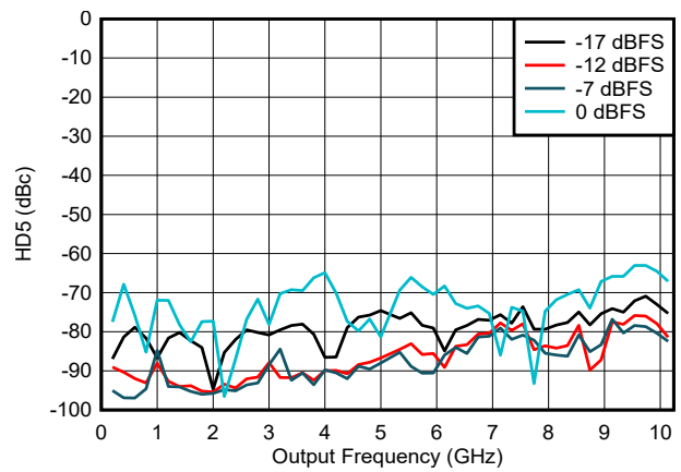
FIG 6-199. HD5 vs Frequency and Digital Amplitude in NRZ/RF Modes
