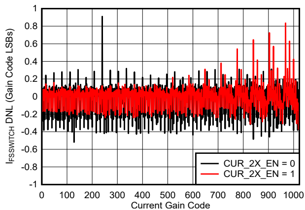
图 6-18. I_{\text{FS\_SWITCH}} Error Differential Non-Linearity vs Gain Code
