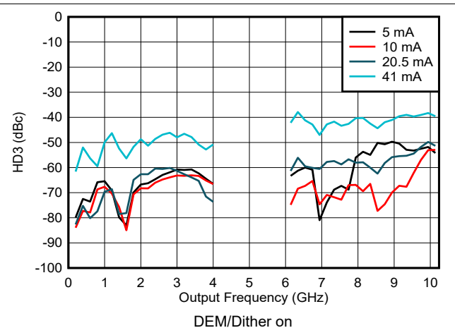
図 6-173. HD3 vs Frequency and Output Current in NRZ/RF Modes
