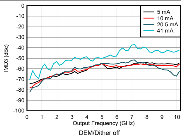
図 6-128. IMD3 vs Frequency and Output Current in NRZ/RF Modes
