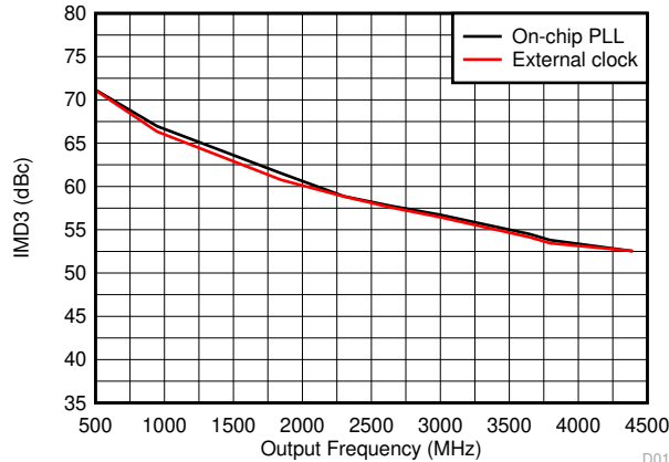
図 6-35. IMD3 vs Output Frequency Over Clocking Option
