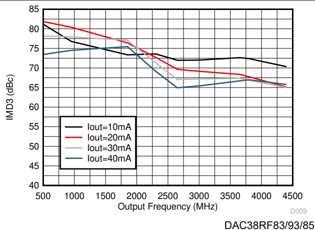
図 6-33. IMD3 vs Output Frequency Over Output Current I_{\text{outFS}}
