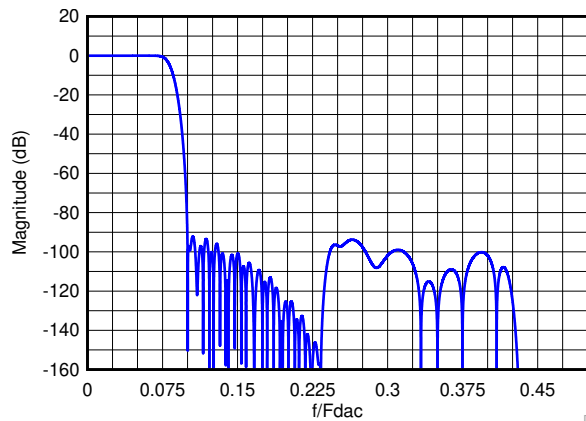
図 7-14. Composite Magnitude Response for 6x Interpolation
