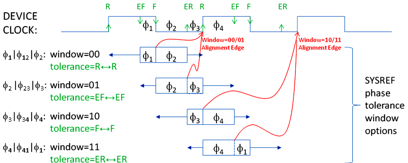
7-11. SYSREF Capture Strategy and Phase Tolerance Windows
