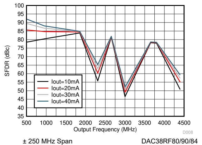
Figure 6-28. SFDR vs Output Frequency Over Output Current I_{\text{outFS}}
