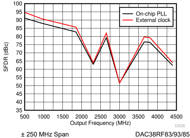
図 6-29. SFDR vs Output Frequency Over Clocking Option
