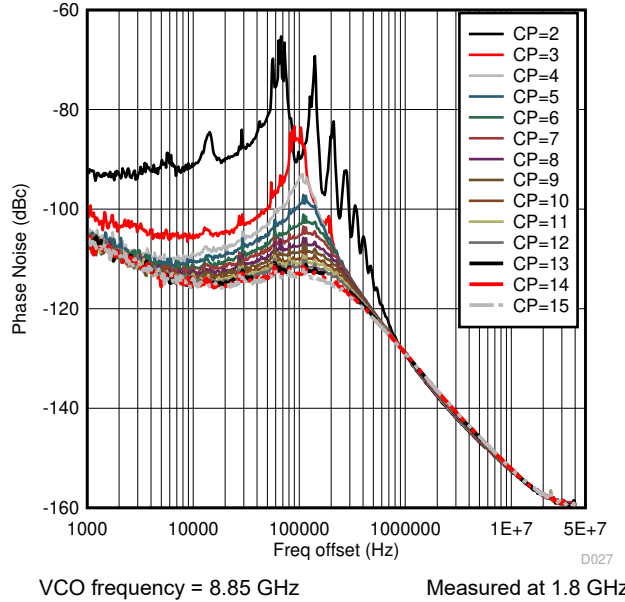
FIG 6-41. VCO1 Phase Noise vs Offset Frequency Over Charge pump current
