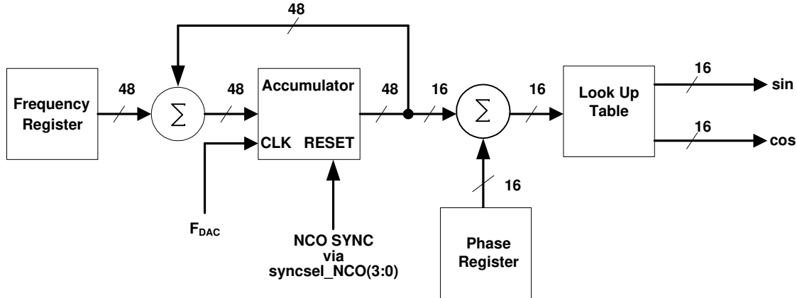
7-22. NCO Block Diagram
