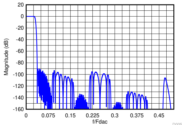
7-18. Composite Magnitude Response for 16x Interpolation
