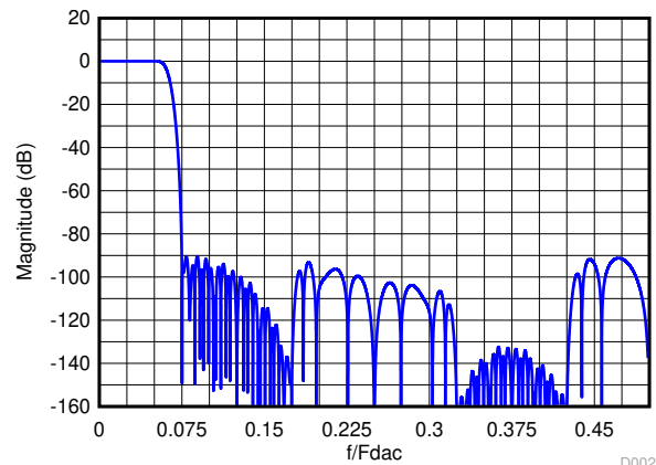
図 7-15. Composite Magnitude Response for 8x Interpolation
