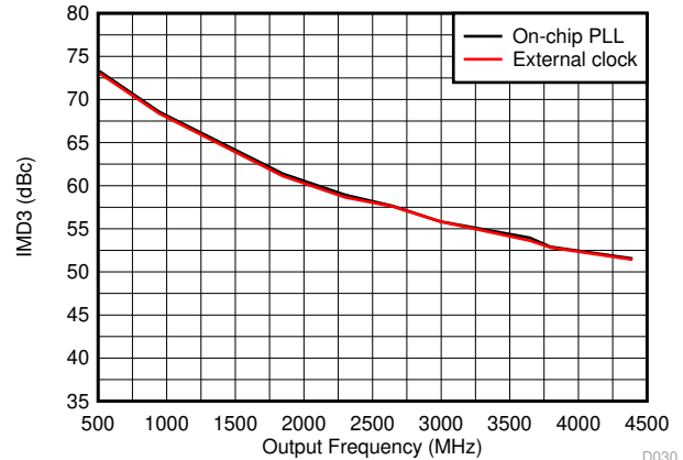
図 6-36. IMD3 vs Output Frequency Over Clocking Option
