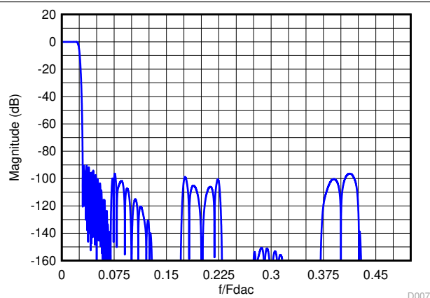
7-20. Composite Magnitude Response for 20x Interpolation
