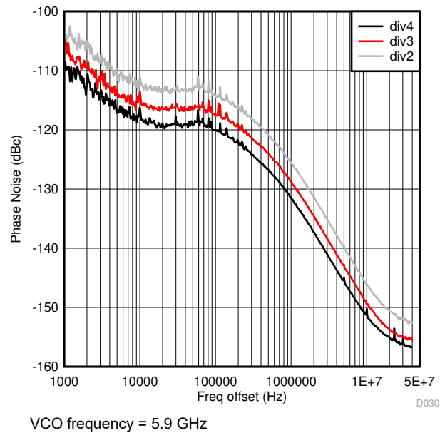
FIG 6-44. VCO0 Output clock Phase Noise vs Offset Frequency Over Divider Ratio
