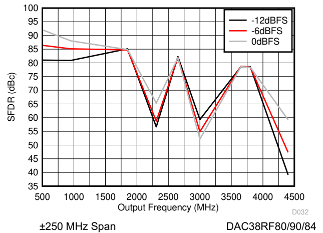
Figure 6-26. SFDR vs Output Frequency Over Input Scale
