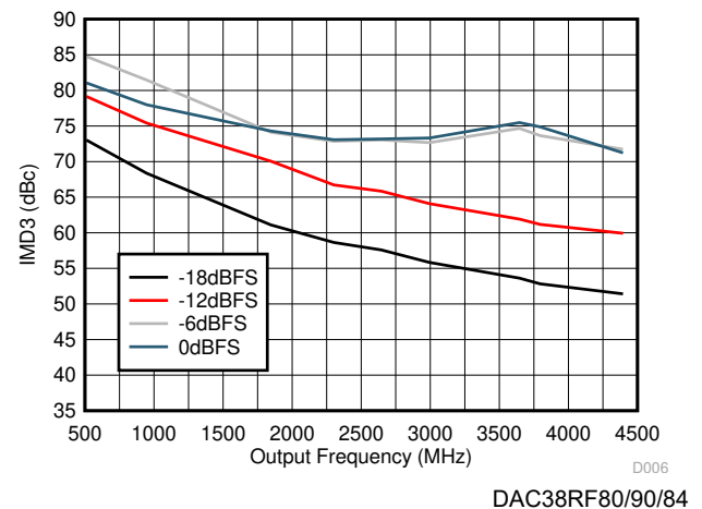
図 6-32. IMD3 vs Output Frequency Over Input Scale
