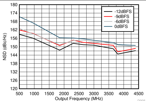
Figure 6-2. NSD vs Output Frequency Over Input Scale
