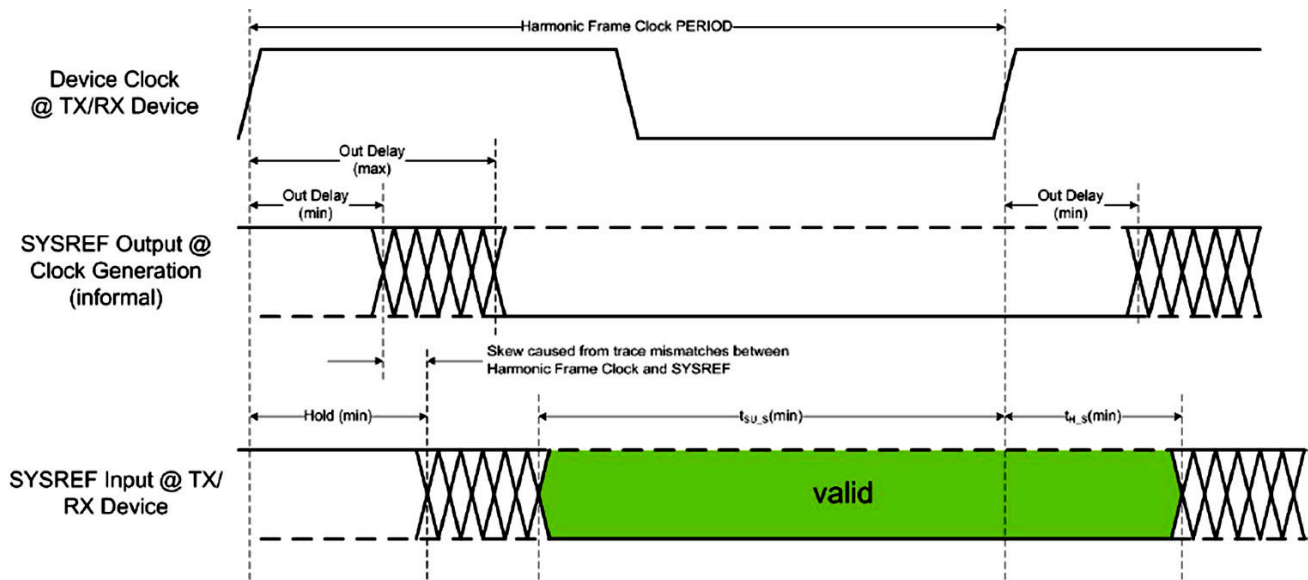
7-10. SYSREF Signal Timing
