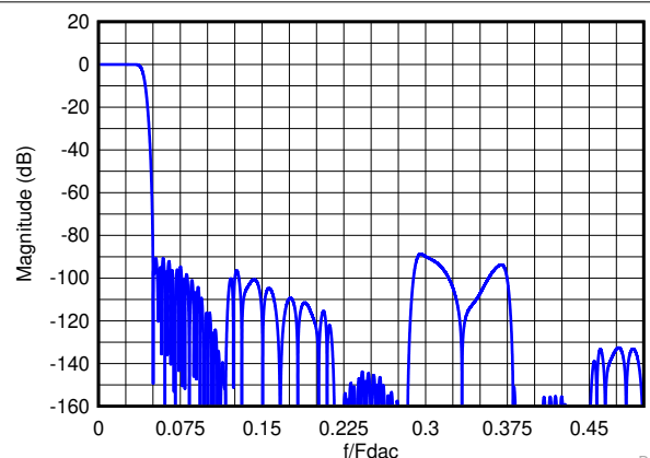
図 7-17. Composite Magnitude Response for 12x Interpolation
