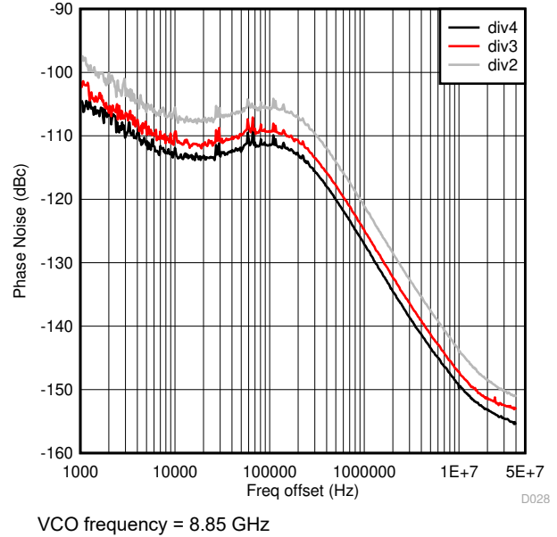
FIG 6-42. VCO1 Output Clock Phase Noise vs Offset frequency Over Divider Ratio
