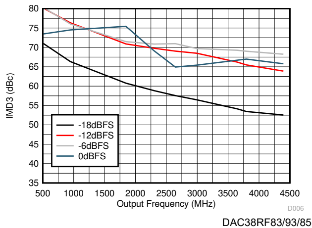
図 6-31. IMD3 vs Output Frequency Over Input Scale
