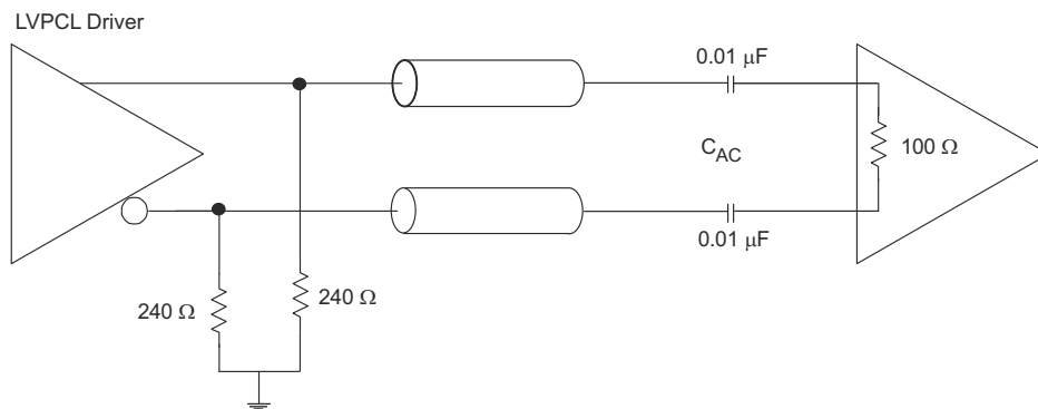
図 7-25. Preferred Clock Input Configuration With a Differential ECL/PECL Clock Source
