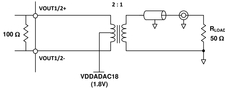
FIG 7-28. Driving a 50-Ω Load Using a 2:1 Impedance Ratio Transformer (DAC38RF83/93/85)
