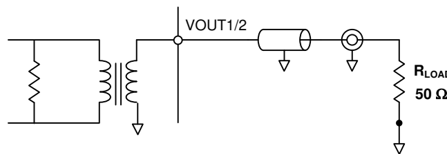
FIG 7-29. Driving a 50-Ω Load (DAC38RF80/90/84)
