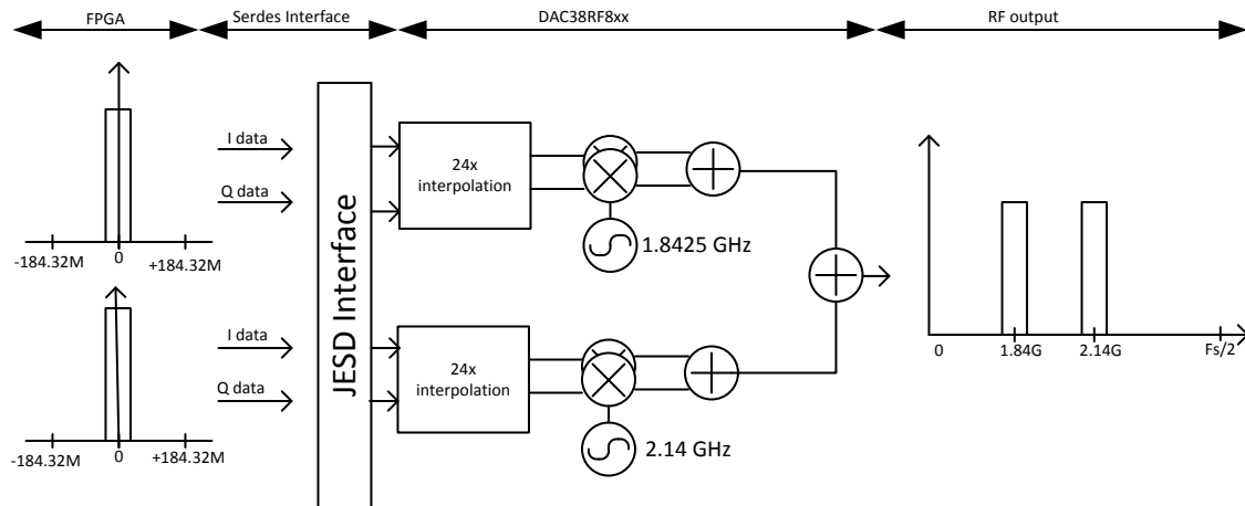
図 8-3. Dual Band LTE Downlink Transmitter Block Diagram
