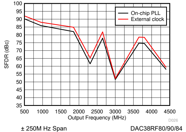
図 6-30. SFDR vs Output Frequency Over Clocking Option
