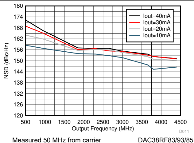
Figure 6-3. NSD vs Output Frequency Over Output Current I_{\text{outFS}}
