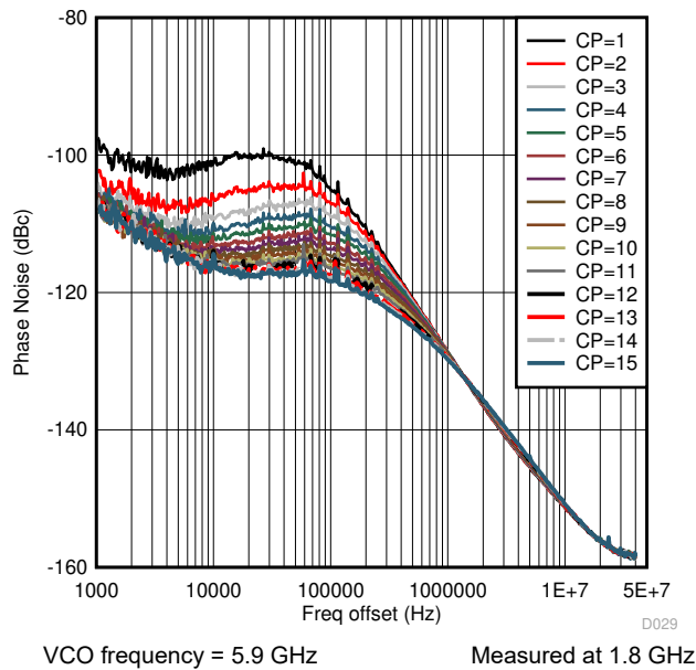
FIG 6-43. VCO0 Phase Noise vs Offset Frequency Over Charge Pump Current
