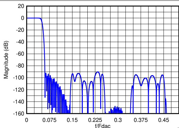
図 7-16. Composite Magnitude Response for 10x Interpolation
