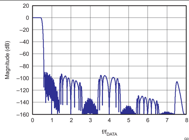
Figure 65. 4x Interpolation Composite Response
